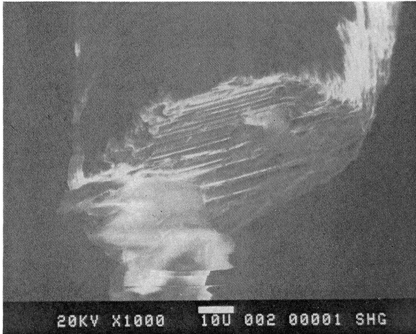
Figure J-1. Cone Element of No. 1 Tip.
