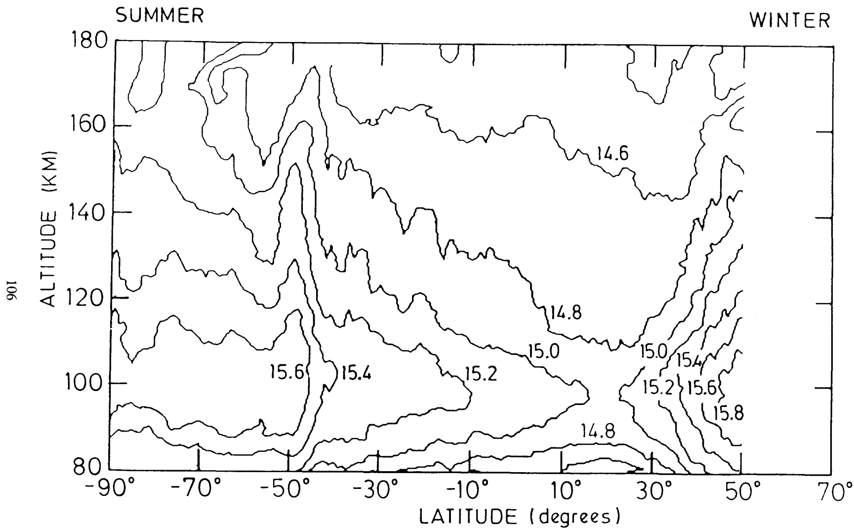
Figure 1. \log_{10} of horizontal column densities ( \text{cm}^{-2} ) of NO observed with the UVNO experiment on the Atmosphere Explorer-D (AE-D) satellite.
