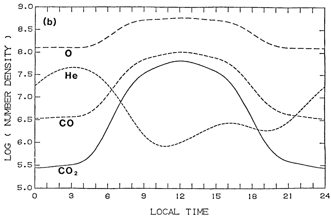
Figure 3. Thermospheric dynamics model results: (a) Equatorial cross-section of temperature versus local time at 170 km. (b) Equatorial cross-section of densities versus local time at 170 km.
