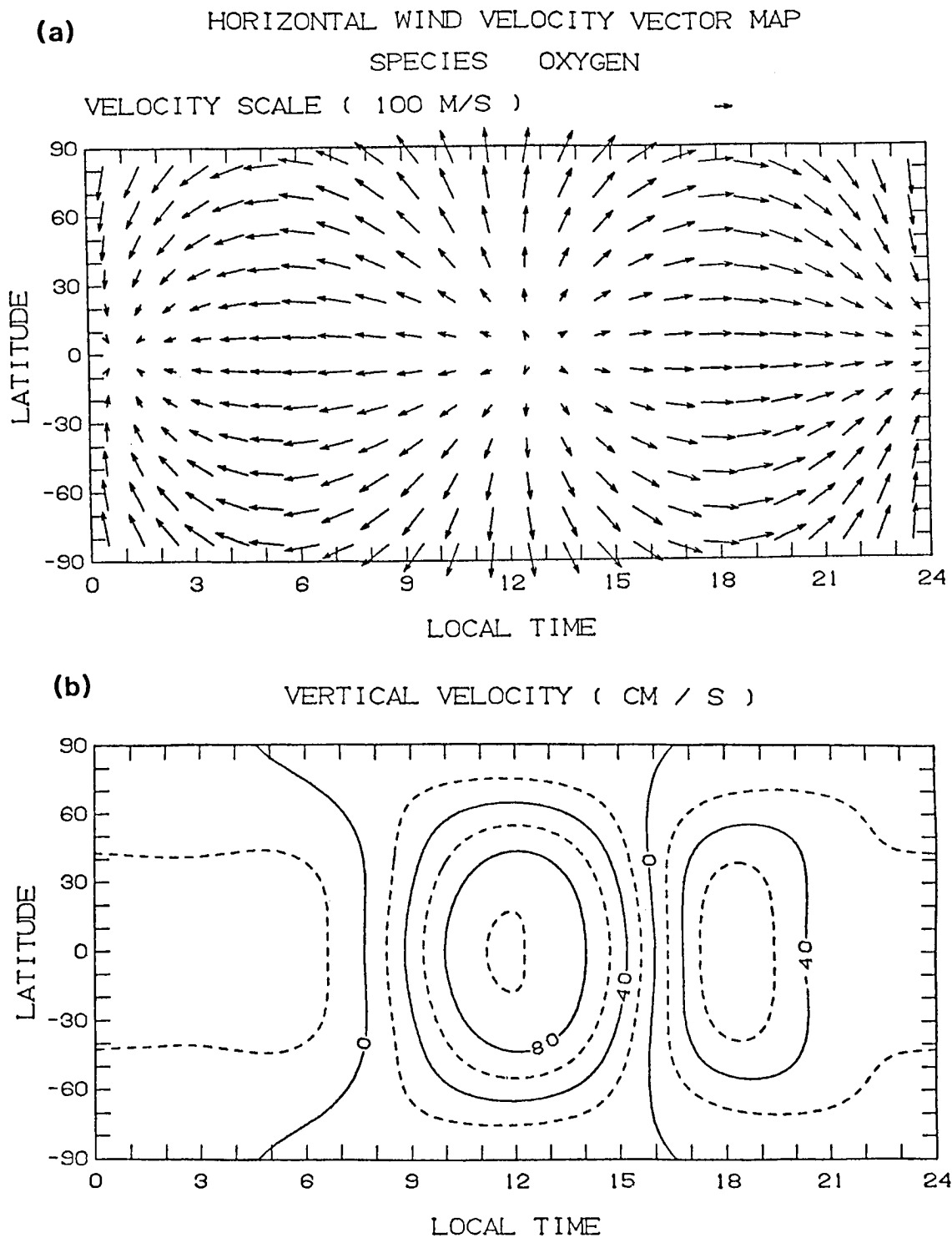
Figure 4. Thermospheric dynamics model results: (a) Horizontal wind velocity vector map at 170 km. (b) Contour map of vertical velocity for oxygen at 170 km.
