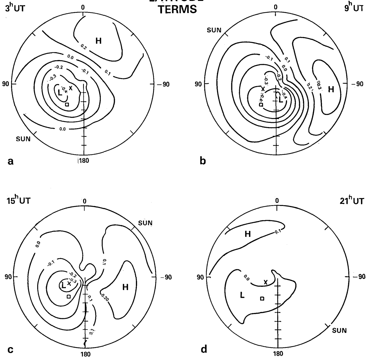
Figure 6. Contour plot in geographic latitude ( -90 to -30 degrees) and longitude coordinates of southern hemisphere He data for six hour UT intervals. Contours indicate the logarithm of He data divided by the MSIS model omitting the UT/longitude and time independent latitude terms of the model for (a) 0 to 6 hrs UT; (b) 6 to 12 hrs UT; (c) 12 to 18 hrs UT; and (d) for 18 to 24 hrs UT.
