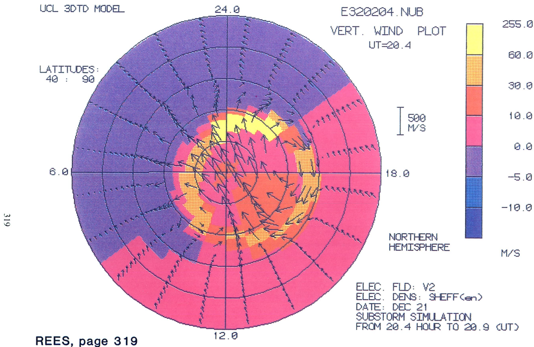
Figure 8. Vertical and Horizontal wind distributions over the Northern Polar region during a geomagnetic substorm. The intense heating from particle and Joule heating effects in the midnight region of the auroral oval generate strong localized upward winds, and force an outward expansion of the thermosphere away from the region of the substorm and westward travelling surge. This Figure shows the onset phase, when the rapid upward vertical winds have been generated, but before the outward expansion has had time to develop.
