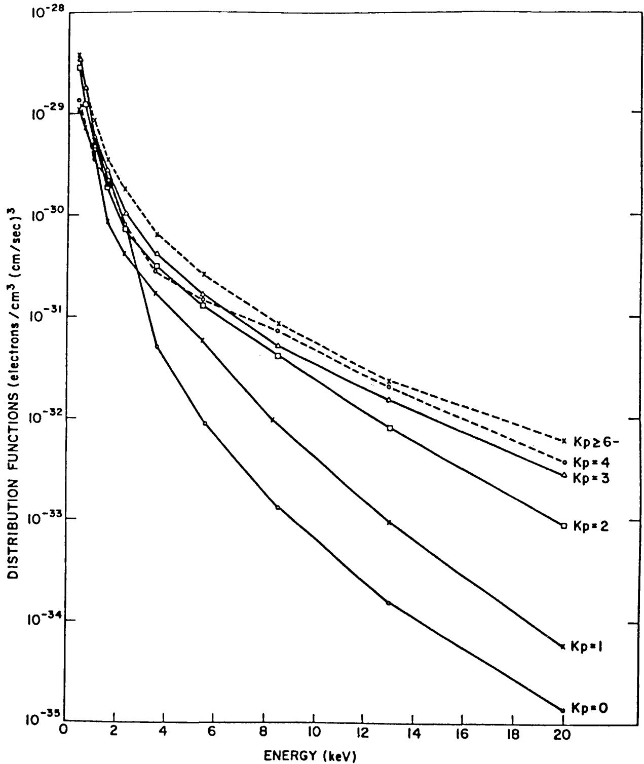
Figure 4. The average distribution function at the pre-noon average energy maximum for each K_p level. The logarithm of the distribution function is plotted versus energy on a linear scale. Only points at energies above 440 eV are included [from Hardy et al., 1985].
