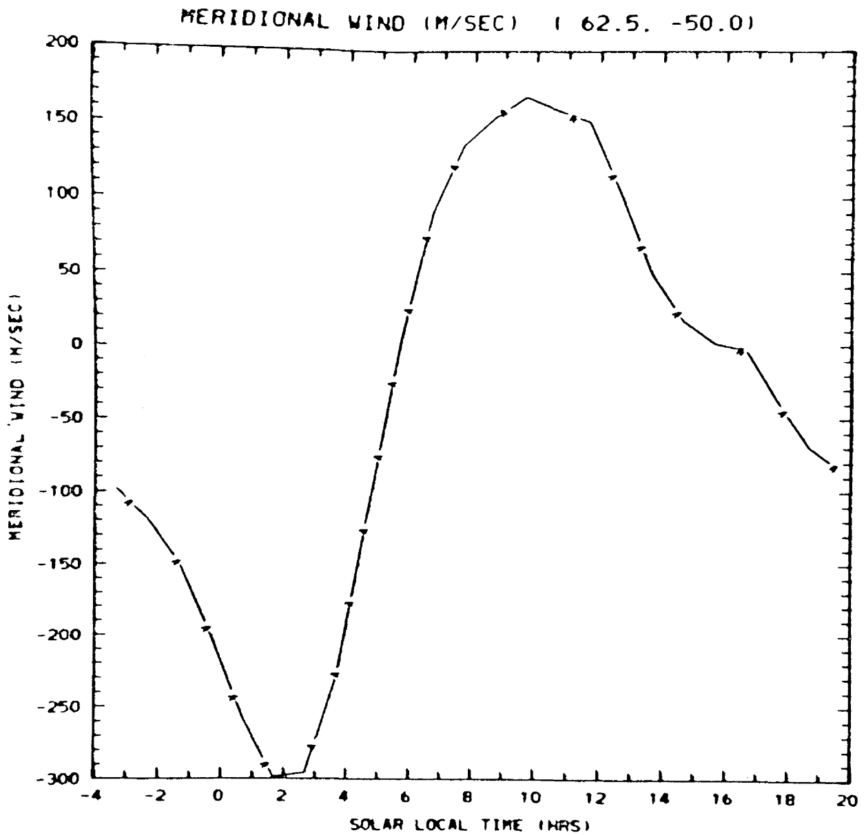
TGCM simulation of the steady-state meridional wind flow at F 2 region altitudes above Sondre Stromfjord during 26-28 June 1984.
