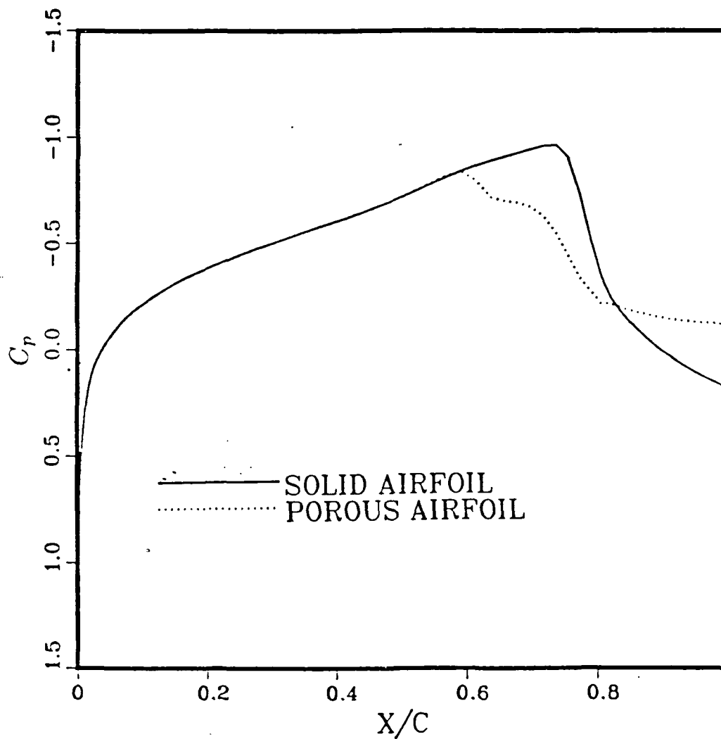
Fig. 6.19 Effects of porosity on a modified RAE 2822 airfoil, x_1 = 0.615 , x_2 = 0.805 , Type 1 porosity on both upper and lower surfaces, \bar{\sigma} = 0.4 , the bottom of cavity is at y/c = 0.0 , Re = 6.5 \times 10^6 , \alpha = 0^\circ , M_\infty = 0.85 and transition is fixed at 0.03.
