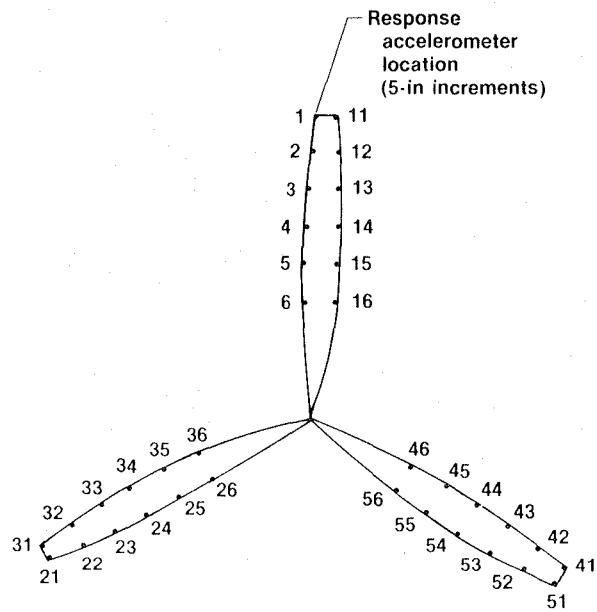
Figure 7. U-8F propeller impact hammer excitation locations.
