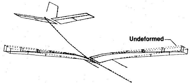
Figure 23. Symmetric wing bending mode shape (empty fuel tanks), 8.03-Hz frequency.
