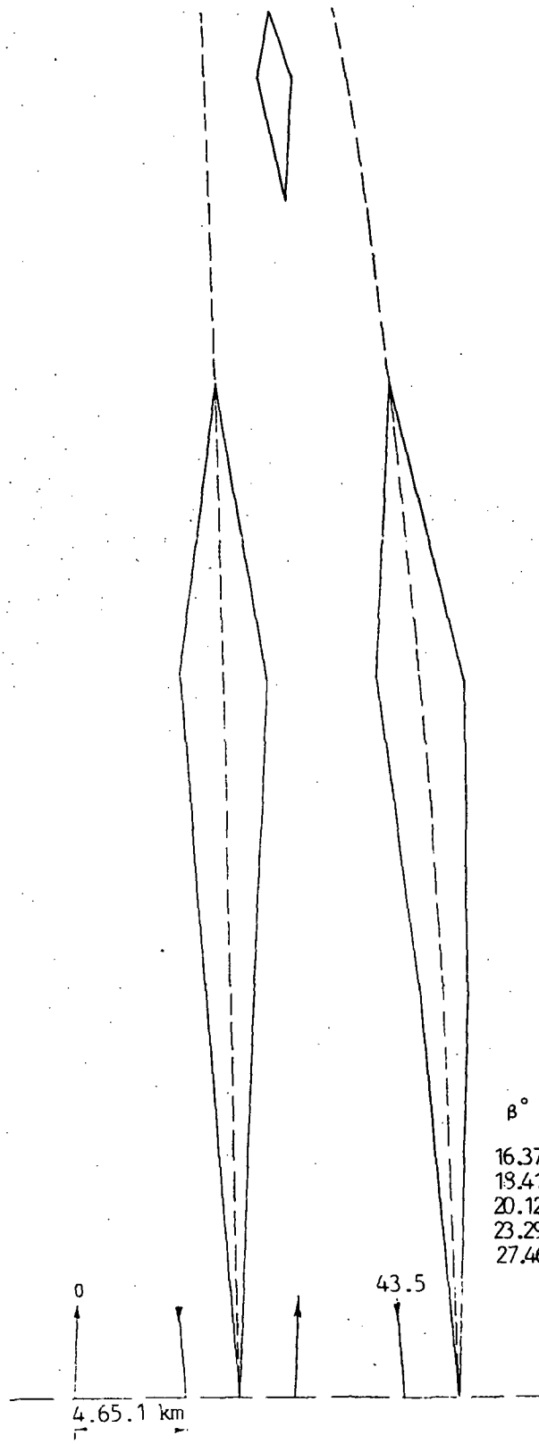
Figure 3.5 - Geometry of ground traces for k = 44 h = 678.62 \text{ km} , i = 90^\circ .
