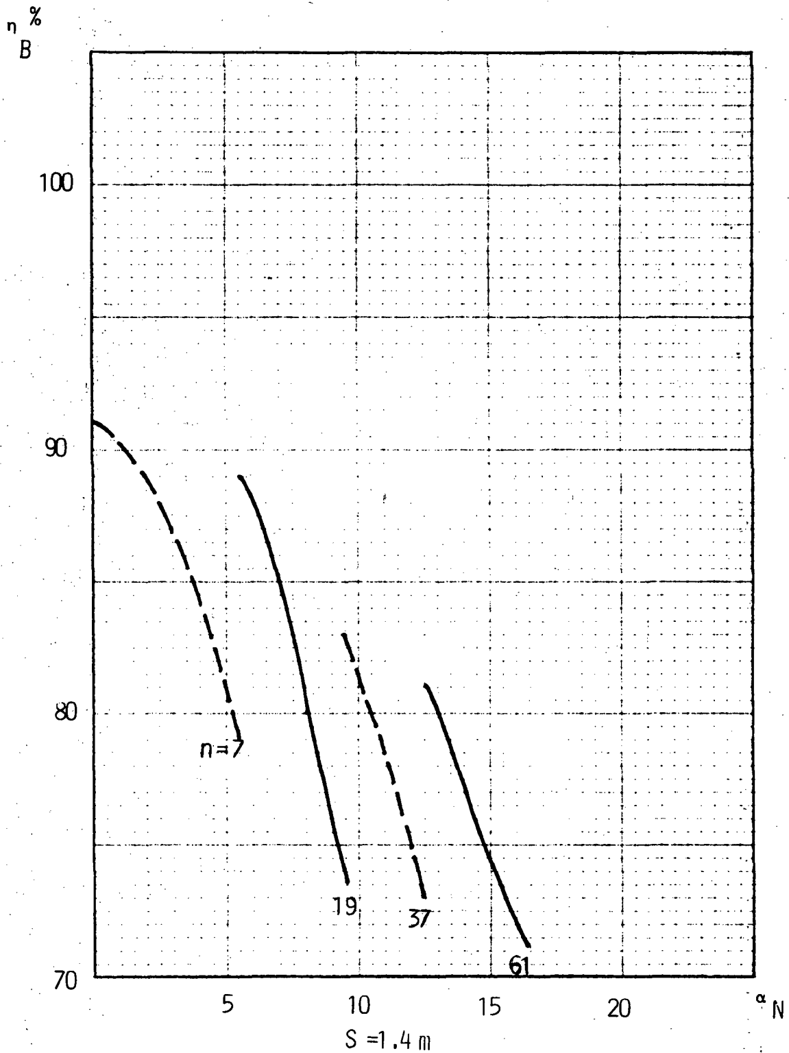
Figure 4.11(b) - Variation of beam scan efficiency and feed cluster size to cover \beta = 11.18^\circ with N = 33 beam for S = 1.4 \text{ m} .
