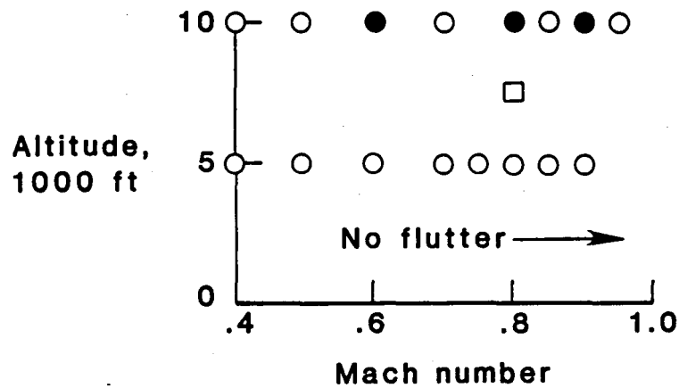
(c) Modified decoupler pylon.
