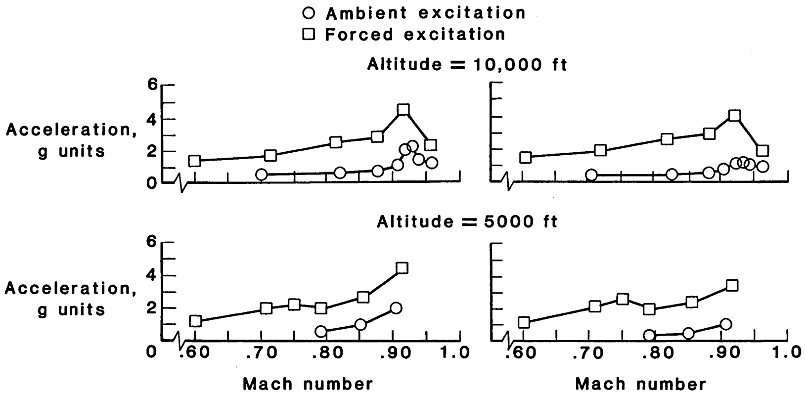
(a) Right wingtip launcher forward accelerometer (A5).
