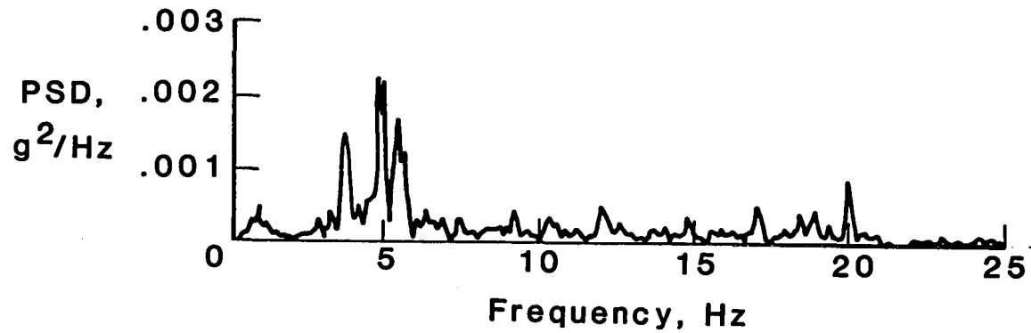
(a) Configuration with initial decoupler pylons.
