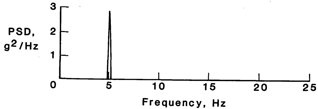
(b) Configuration with standard pylons.
