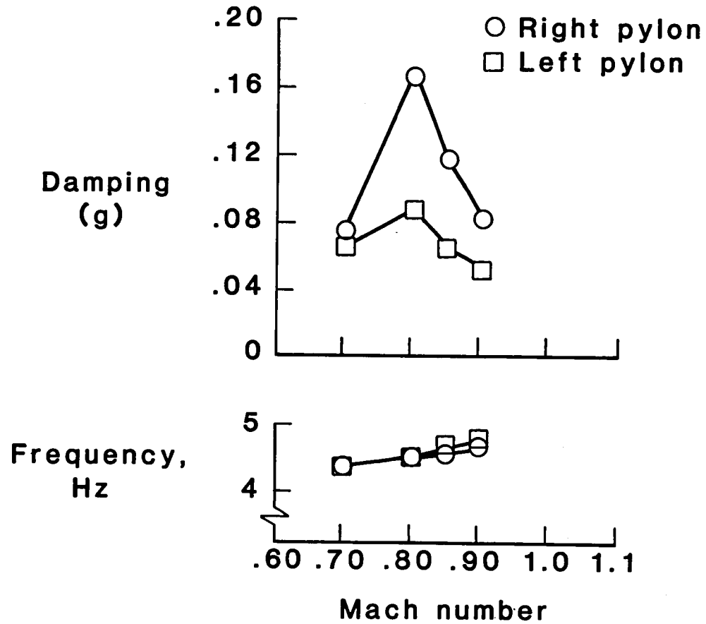
Figure 9. - Variation of frequency and damping of pylon pitch mode for control system burst excitation. Initial decoupler pylon, Altitude = 10,000 feet.
