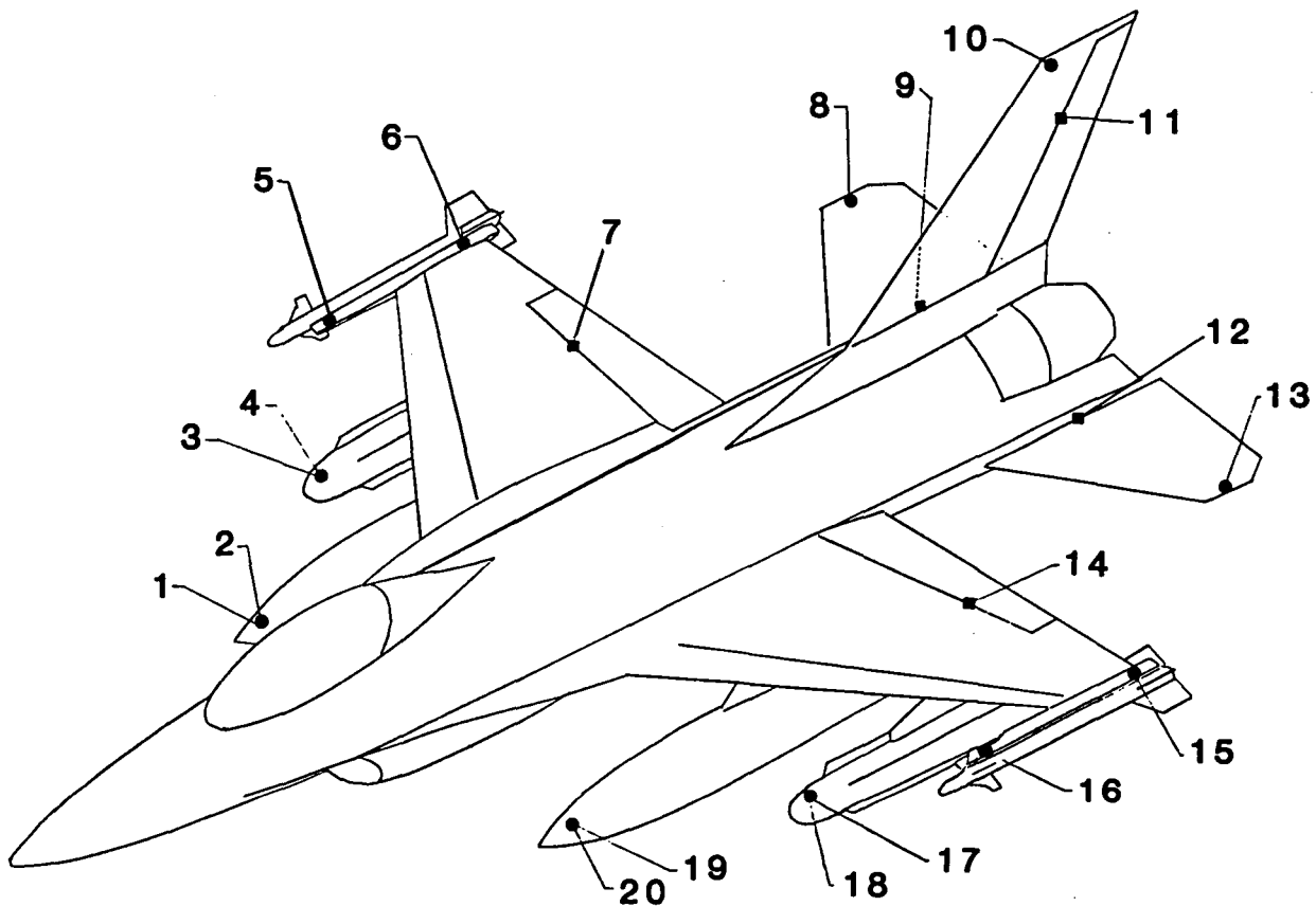
Figure 2. - Airplane flutter instrumentation.
