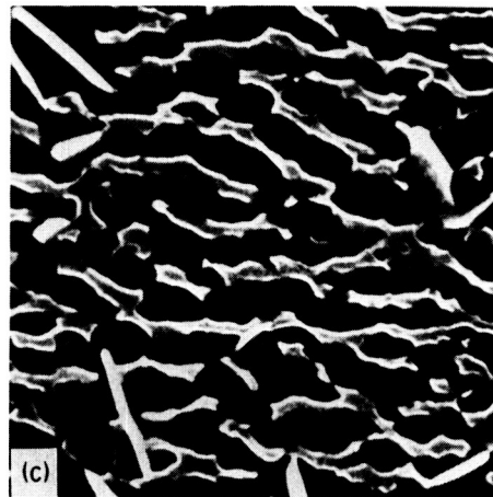
Figure 5. - Lamellar structures which developed in Alloy 143 after 50 hours of creep testing at 982 °C/234 MPa in the (a) oil quenched, (b) air quenched, and (c) aged conditions. From reference 8.
