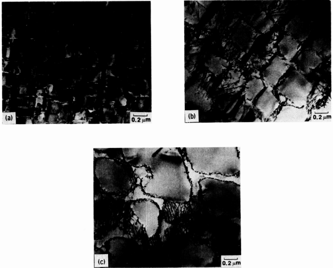
Figure 3. - The \gamma' precipitate and dislocation structure in Alloy 143 single crystals after solution treatment plus (a) oil quenching, \gamma' size=0.15 \mu\text{m} , (b) air quenching, \gamma' size=0.33 \mu\text{m} , and (c) air quenching plus aging at 982 °C/115 hours, \gamma' size=0.44 \mu\text{m} . From reference 8.
