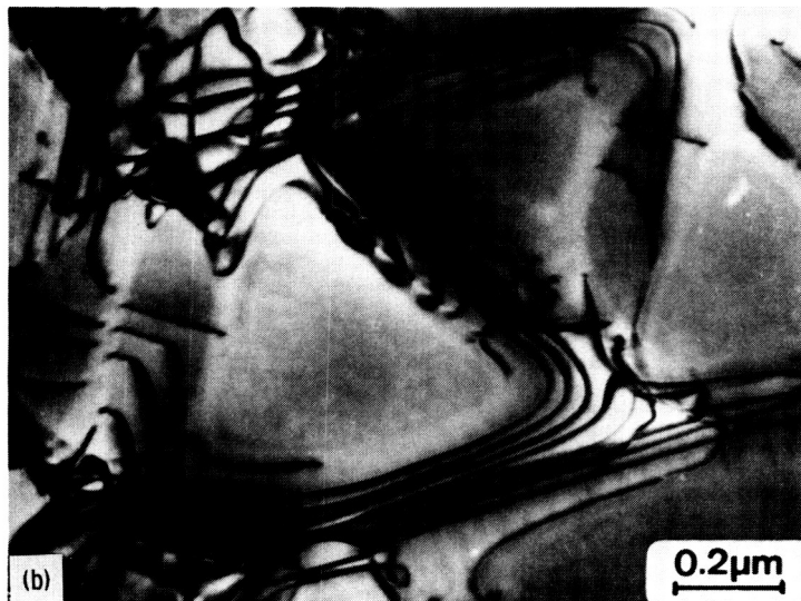
Figure 9. - Typical deformation structures observed during primary creep at 760^{\circ}\text{C} . (a) \gamma' particle shearing by intrinsic/extrinsic stacking faults. (b) Orowan looping around \gamma' particles. (c) Homogeneous dislocation distribution associated with the looping process. From references 11 and 37.
