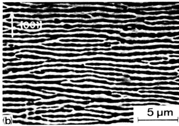
Figure 6. - Lamellar structures which developed in CMSX-2 single crystals after 20 hours of creep testing at 1050 °C/120 MPa having initial \gamma' sizes of (a) 0.30 \mu\text{m} and (b) 0.45 \mu\text{m} . From reference 11.
