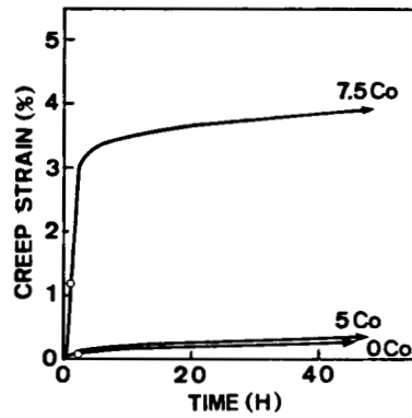
Figure 11. - Influence of Co level on primary creep behavior of MXON single crystals at 760°C/750 MPa. From reference 37.
