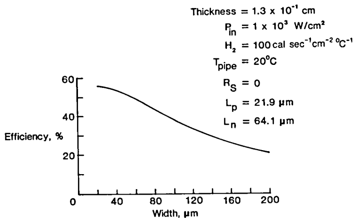
Figure 5 - Converter efficiency vs. converter width
