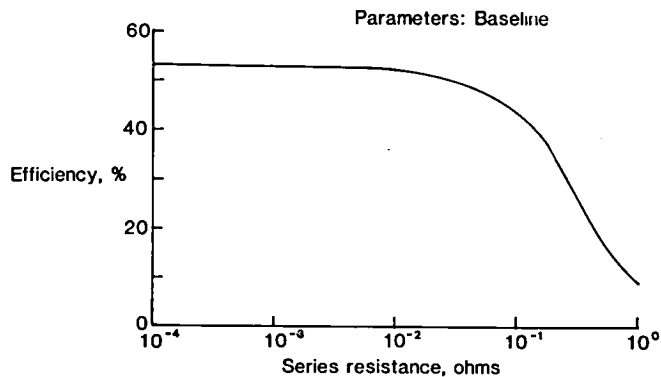
Figure 10 - Converter efficiency vs. series resistance
