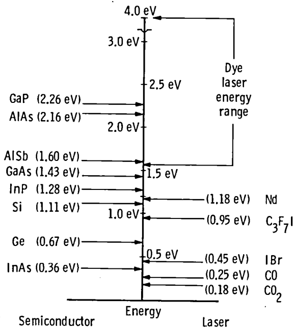
Figure 1 - Semiconductor bandgap energy - laser photon energy relationship
