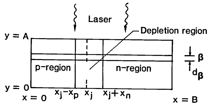
Figure 2 - Converter geometry
