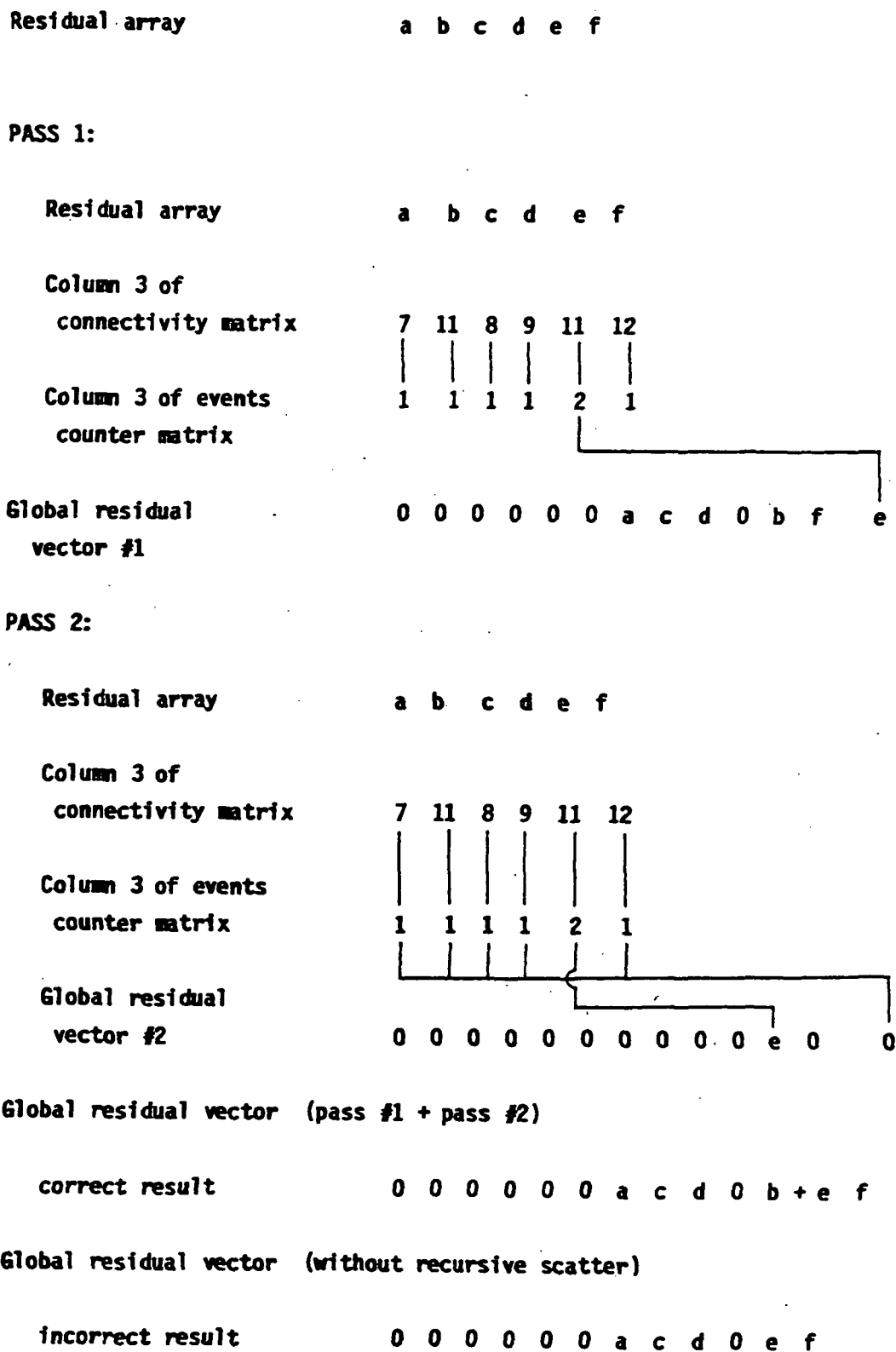
Fig. 3.7 Assembly process using recursive scatter.
