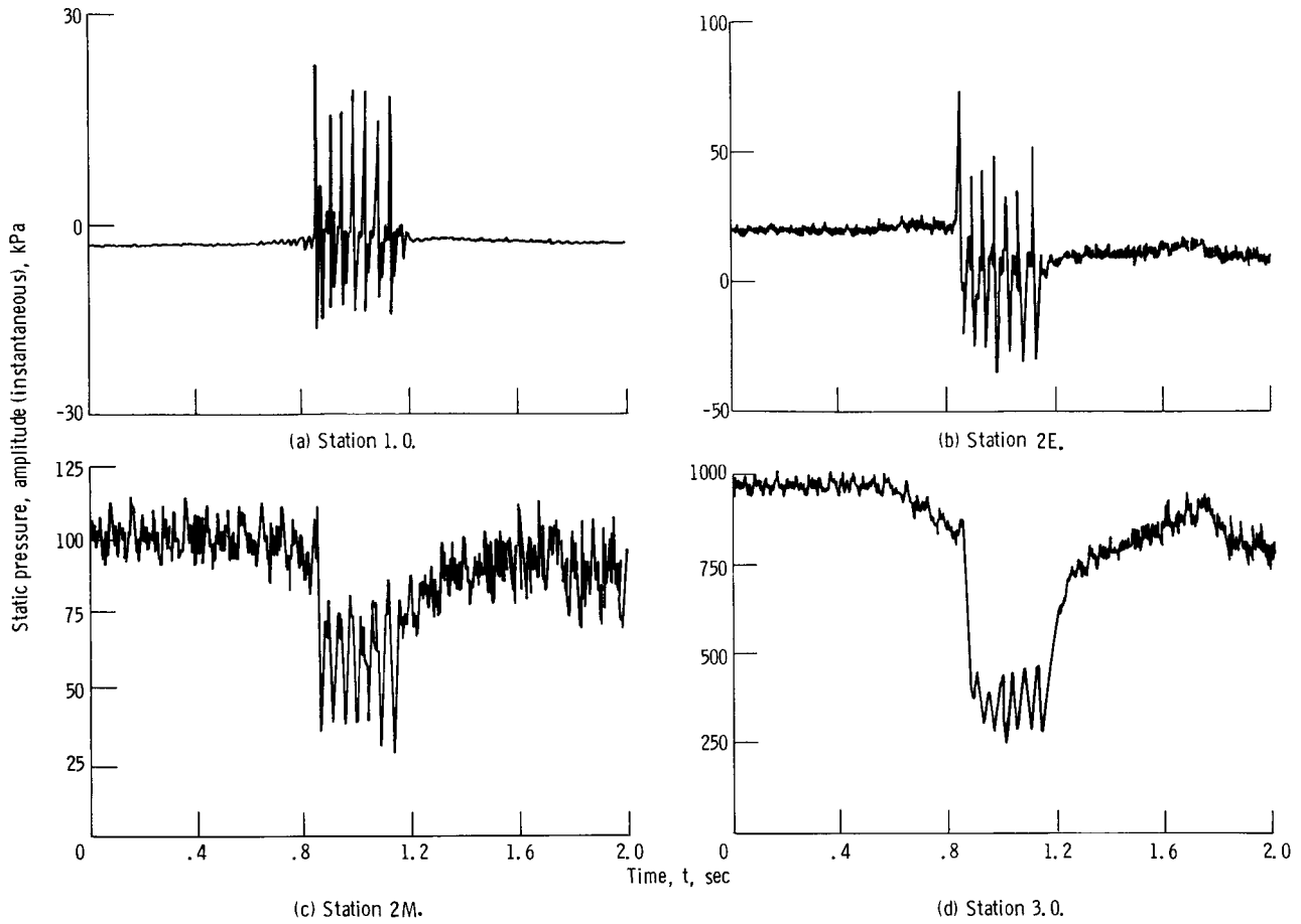
Figure 9. - Instantaneous time history of compressor response.
