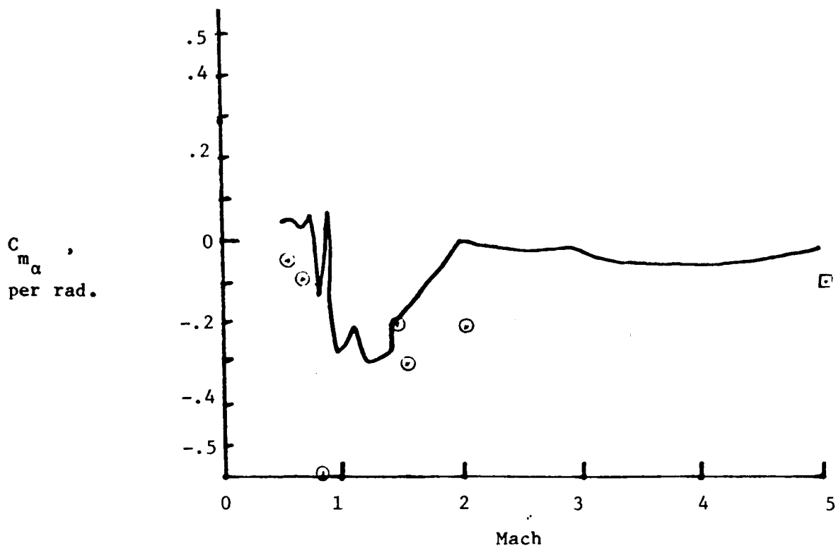
Figure 3.- Static stability versus Mach number.
