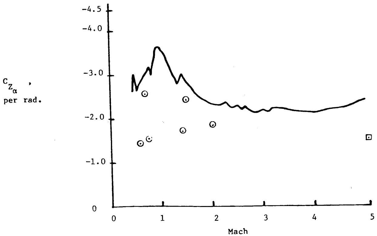
Figure 2.- Change in normal force with alpha versus Mach number.
