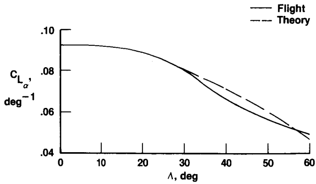
Figure 7. Variation in lift curve slope with wing sweep; \alpha = 4^\circ .
