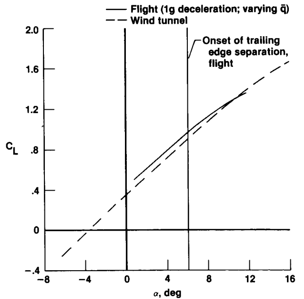
Figure 5. Untrimmed lift coefficient results.
