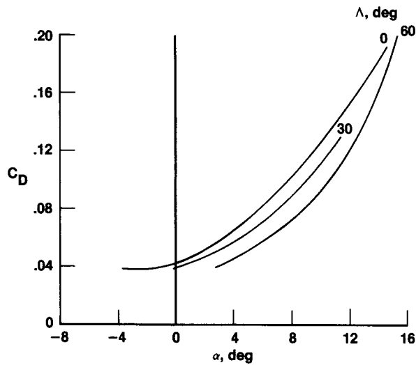
Figure 10. Flight data showing variation of drag with wing sweep; \Lambda = 0^\circ, 30^\circ, \text{ and } 60^\circ .
