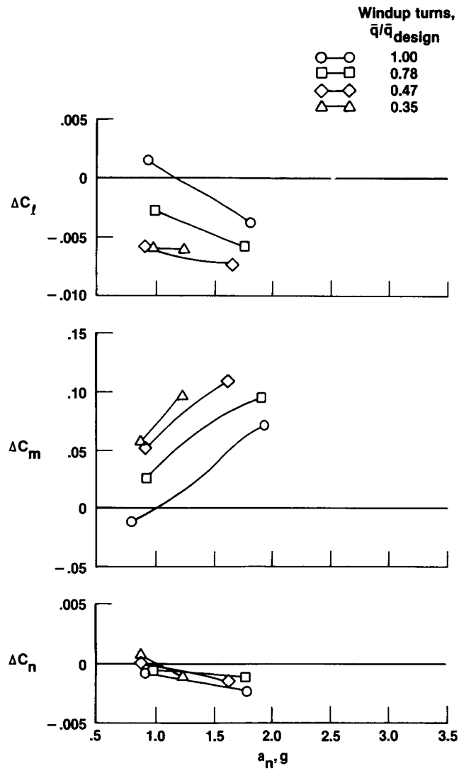
Figure 20. Moment increments at various \bar{q}/\bar{q}_{design} ratios; \Lambda = 35^\circ .
