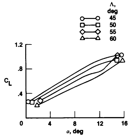
Figure 6. Untrimmed lift coefficient at high wing sweeps in flight.
