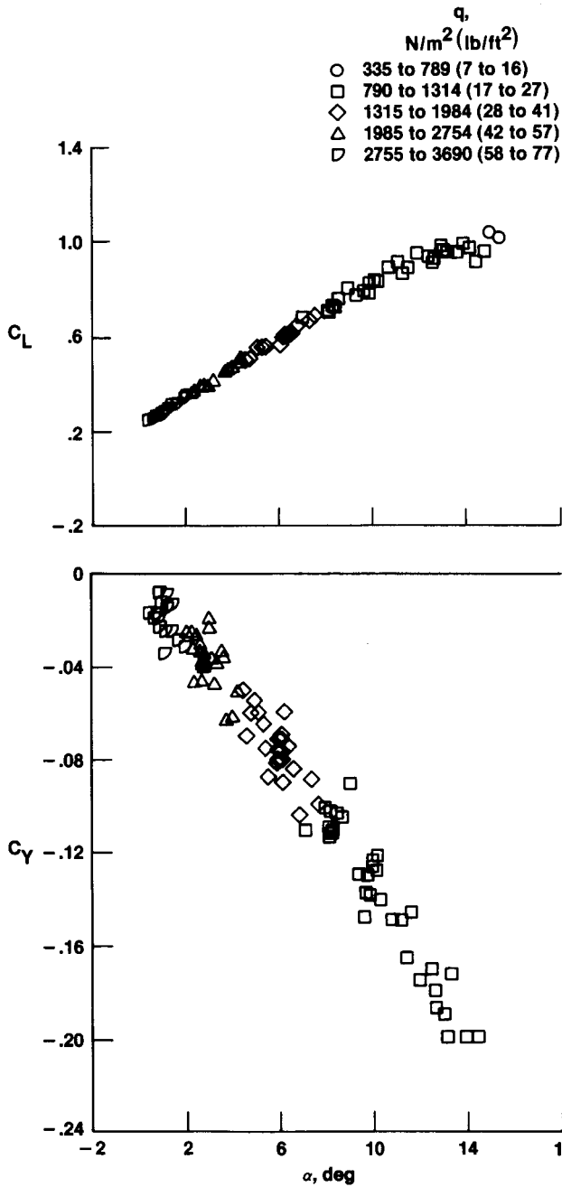
Figure 4. Example of unfaired flight sideforce data from a deceleration maneuver; \Lambda = 45^\circ .
