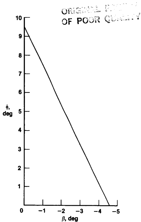
Figure 15. Flight estimates of the AD-1 airplane trim requirements at \Lambda = 60^\circ and C_L = 0.3 and with right wing down.
