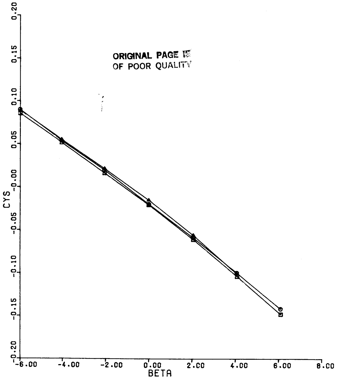
Figure 68(c). CY5 vs BETA Configuration 6, ALPHA = 10, MACH = 0.6
