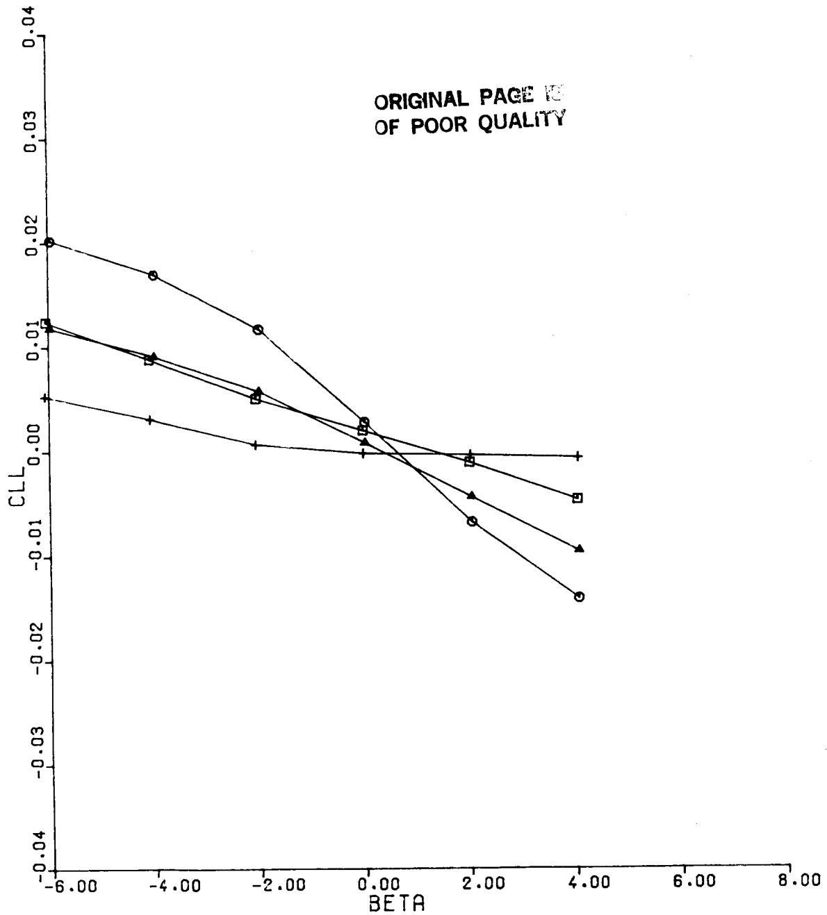
Figure 40(a). CLL vs BETA, DS = 10, Configuration 2, MACH = 0.9
