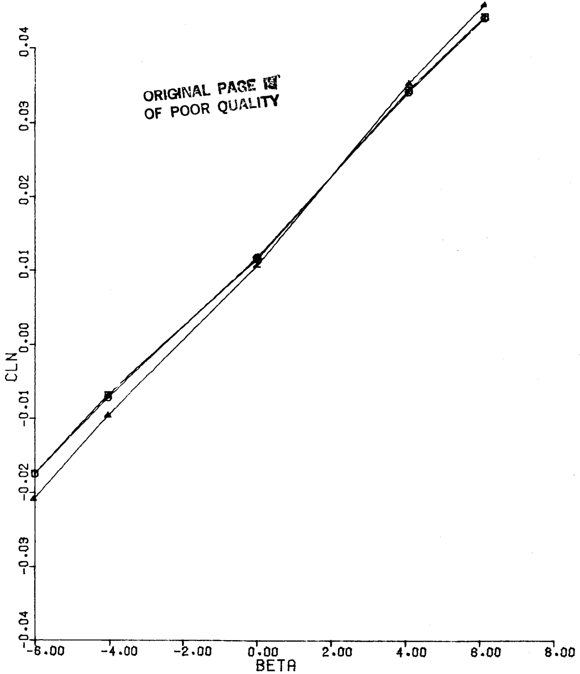
Figure 51(b). CLN vs BETA Configuration 4, ALPHA = 10, MACH = 0.6
