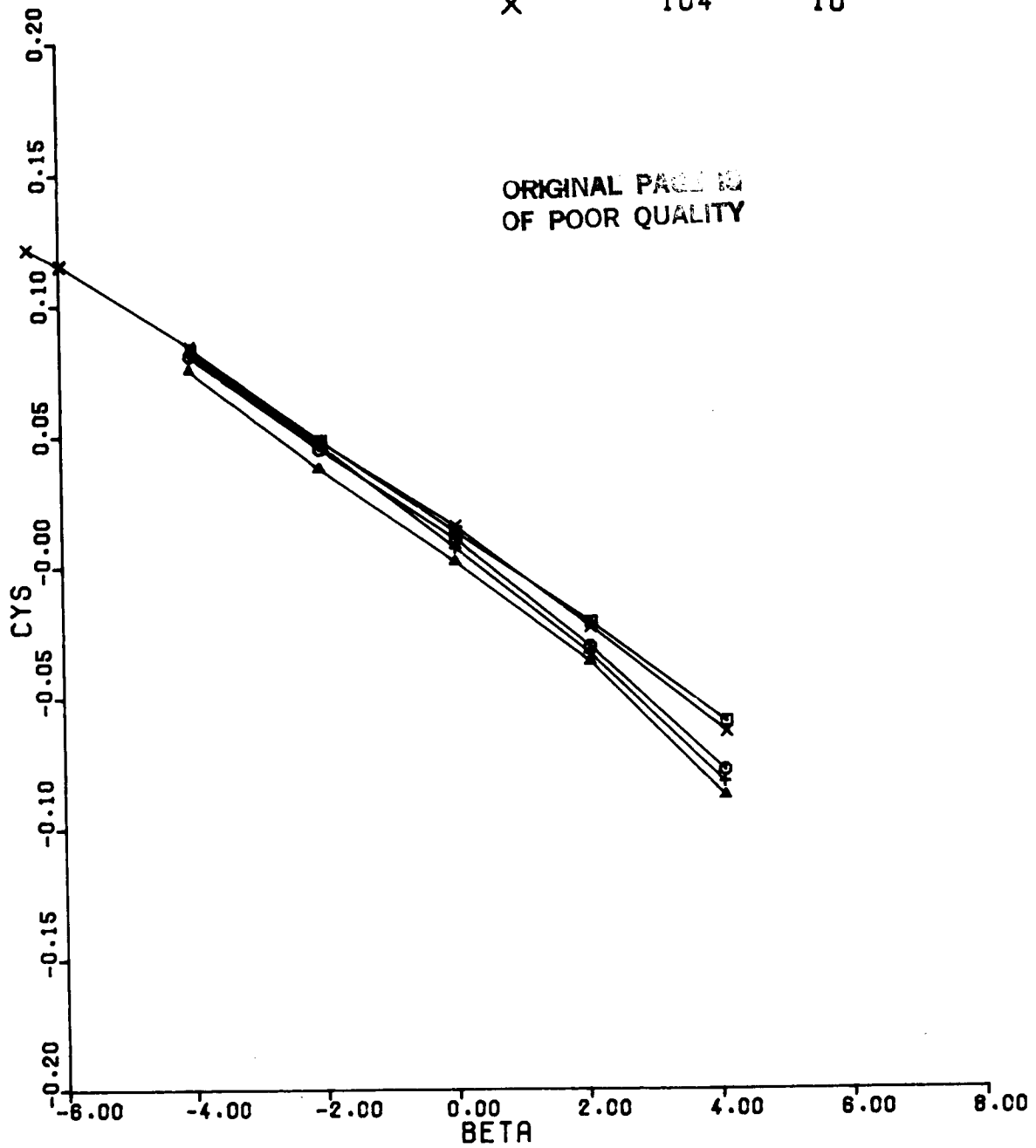
Figure 24(c). CY5 vs BETA, DCR = 0, Configuration 1, ALPHA = 16, MACH = 1.2
