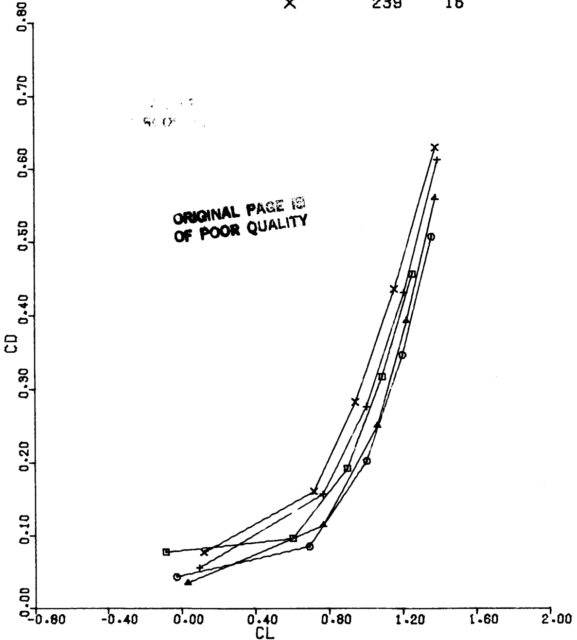
Figure 65(b). CD vs CL Configuration 6, BETA = 0, MACH = 0.6
