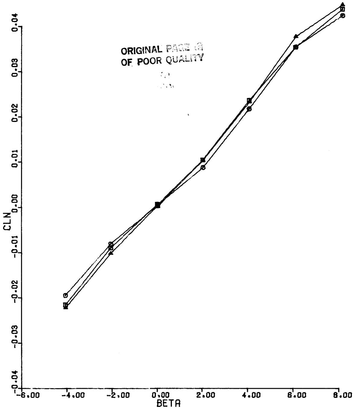
Figure 12(b). CLN vs BETA Configuration 1, ALPHA = 10.9, MACH = 1.2
