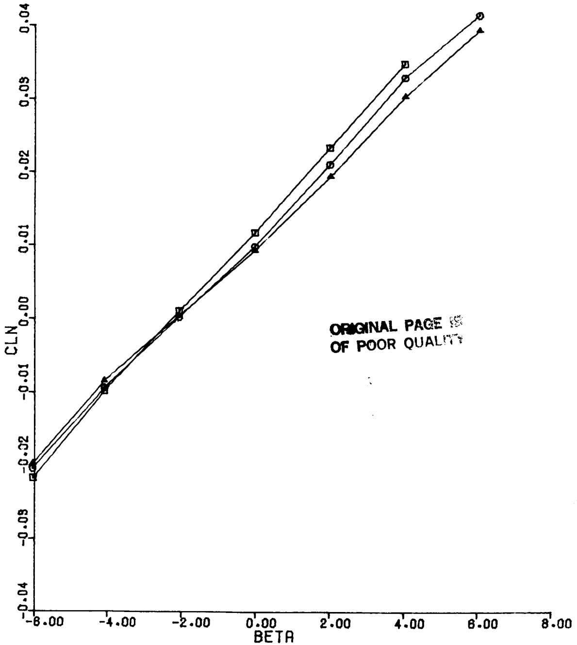
Figure 67(b). CLN vs BETA Configuration 6, ALPHA = 11, MACH = 0.9
