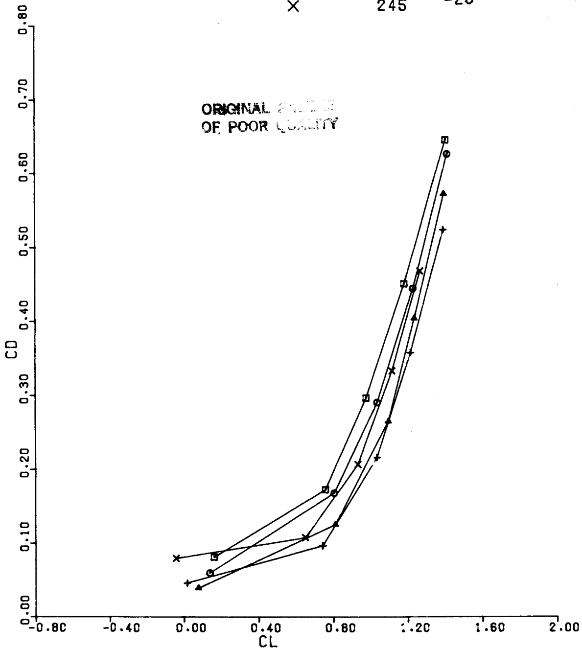
Figure 71(b). CD vs CL Configuration 7, BETA = 0, MACH = 0.6
