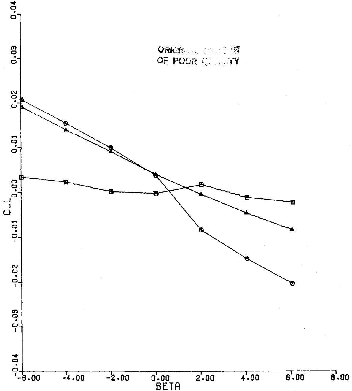
Figure 80(a). CLL vs BETA Configuration 8, ALPHA = 16, MACH = 0.9
