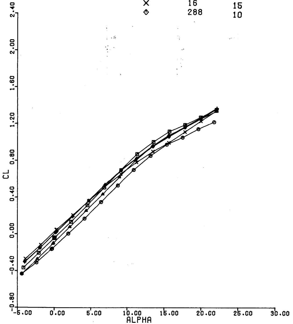
Figure 1(a). CL vs ALPHA Configuration 1, MACH = 0.6, BETA = 0
