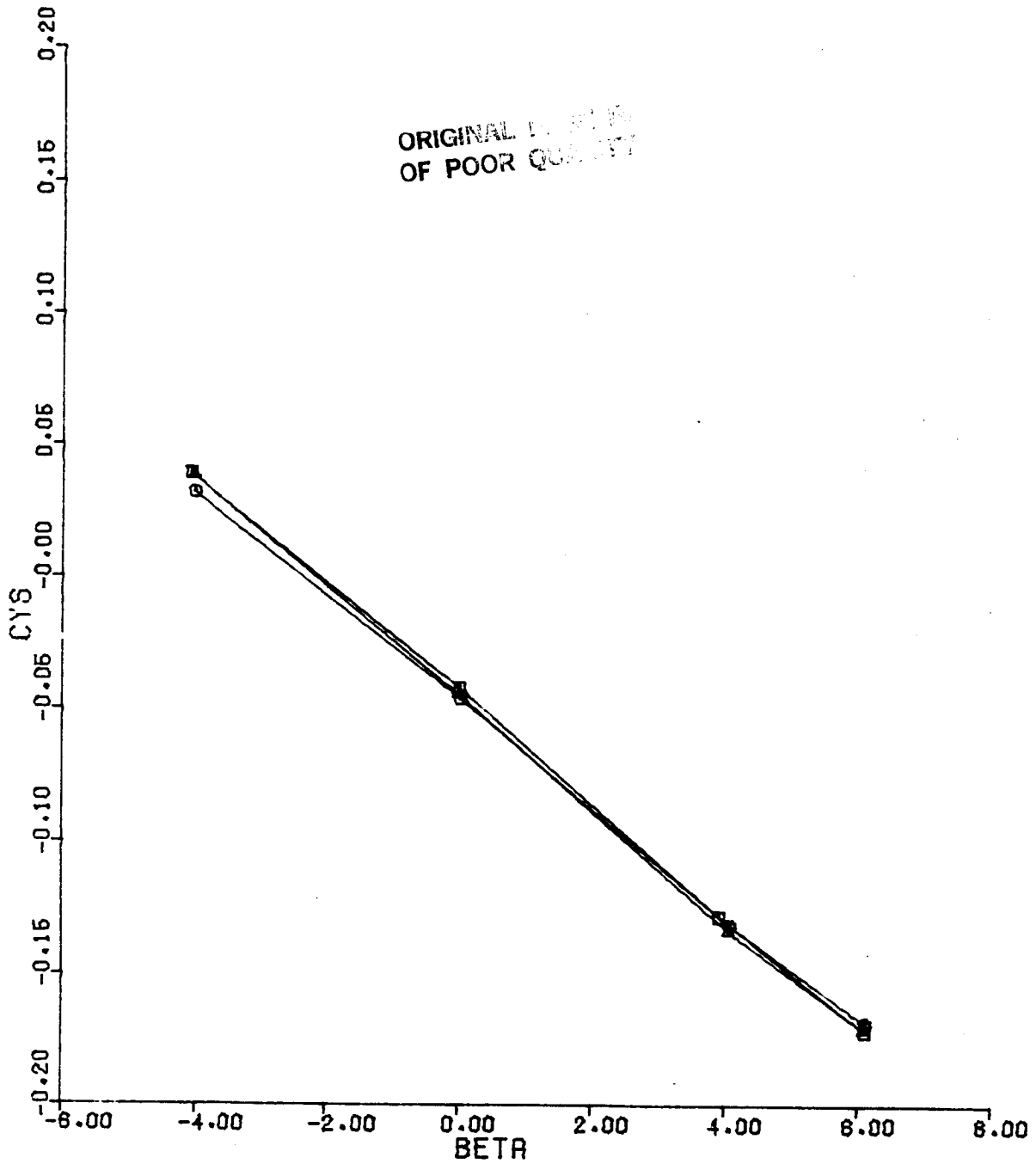
Figure 52(c). CY5 vs BETA Configuration 4, ALPHA = 11, MACH = 0.9
