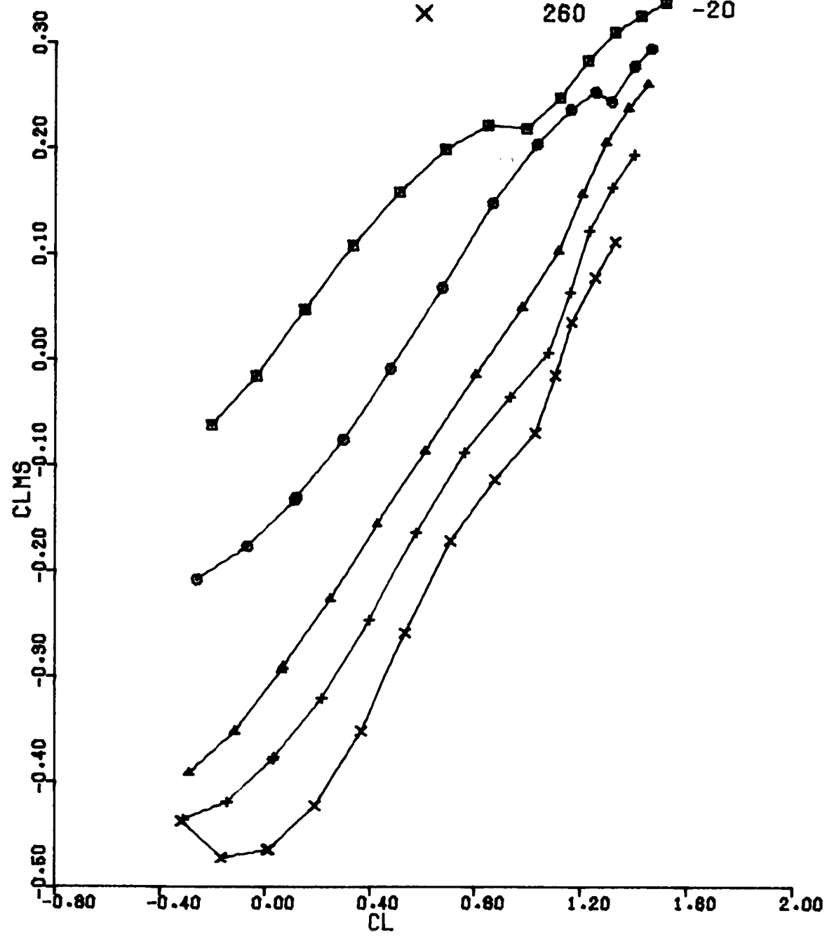
Figure 73(c). CLMS vs CL Configuration 8, BETA = 0, MACH = 0.6
