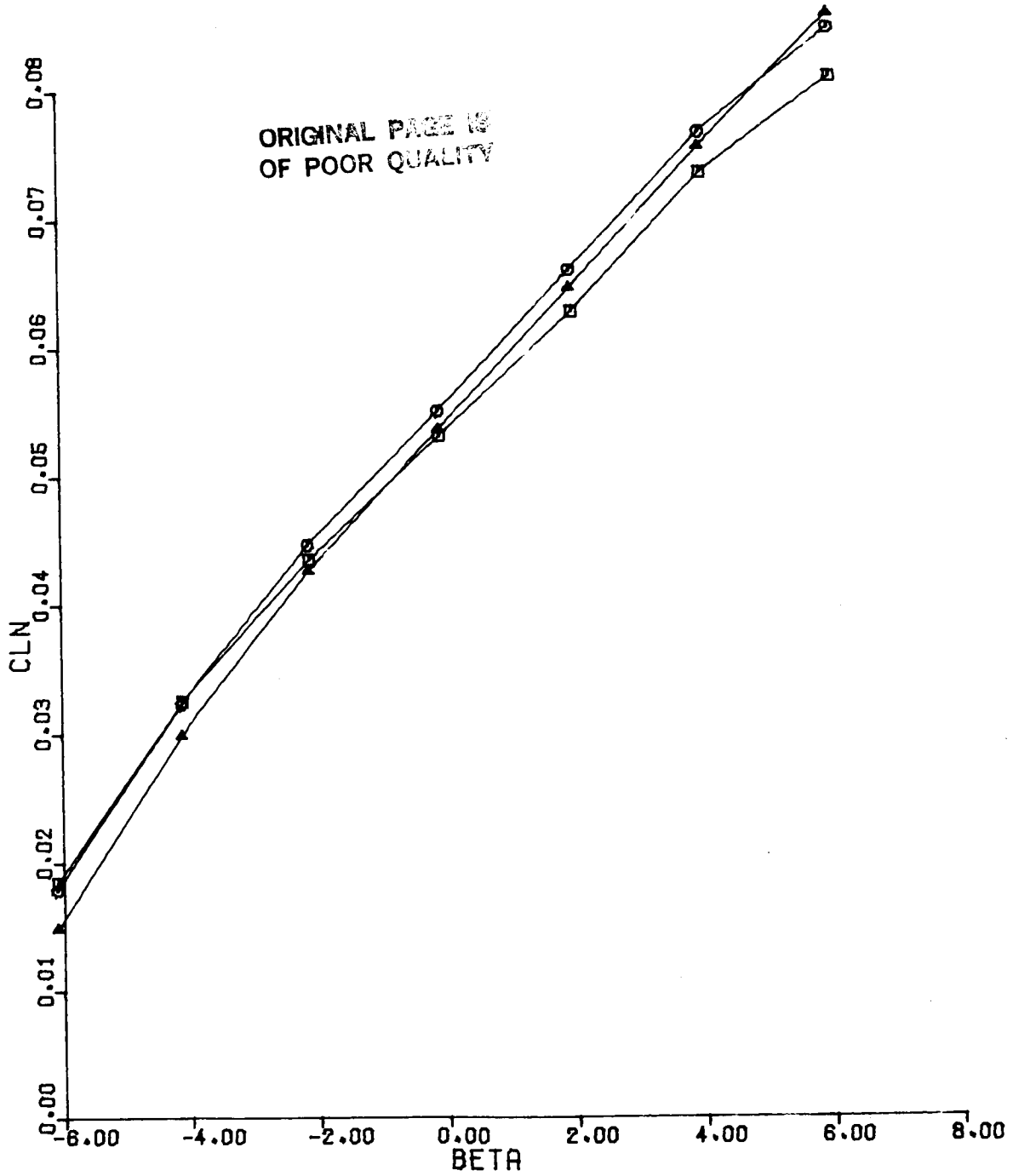
Figure 89(b). CLN vs BETA Configuration 9, ALPHA = 10, MACH = 0.6
