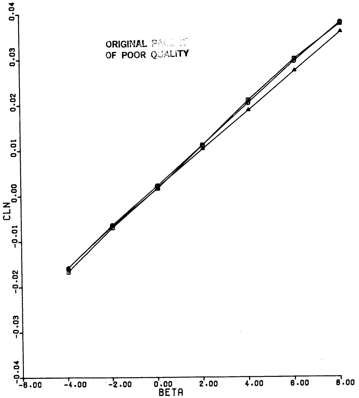
Figure 7(b). CLN vs BETA Configuration 1, MACH = 0.6, ALPHA = 15
