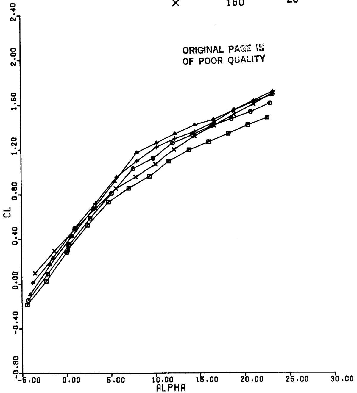
Figure 45(a). CL vs ALPHA, DS = 5, Configuration 3, BETA = 0, MACH = 0.9
