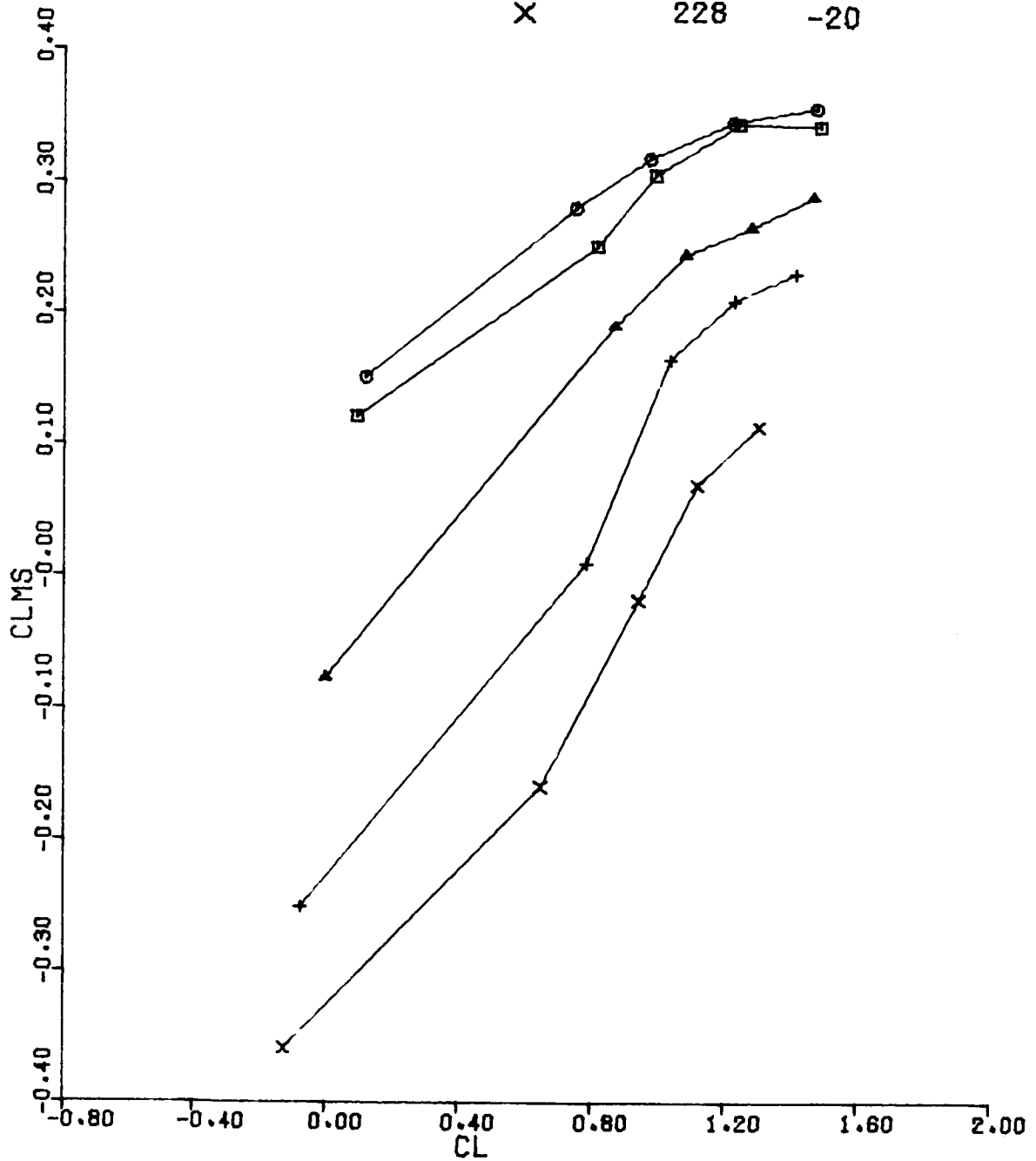
Figure 64(c). CLMS vs CL Configuration 6, BETA = 0, MACH = 0.9
