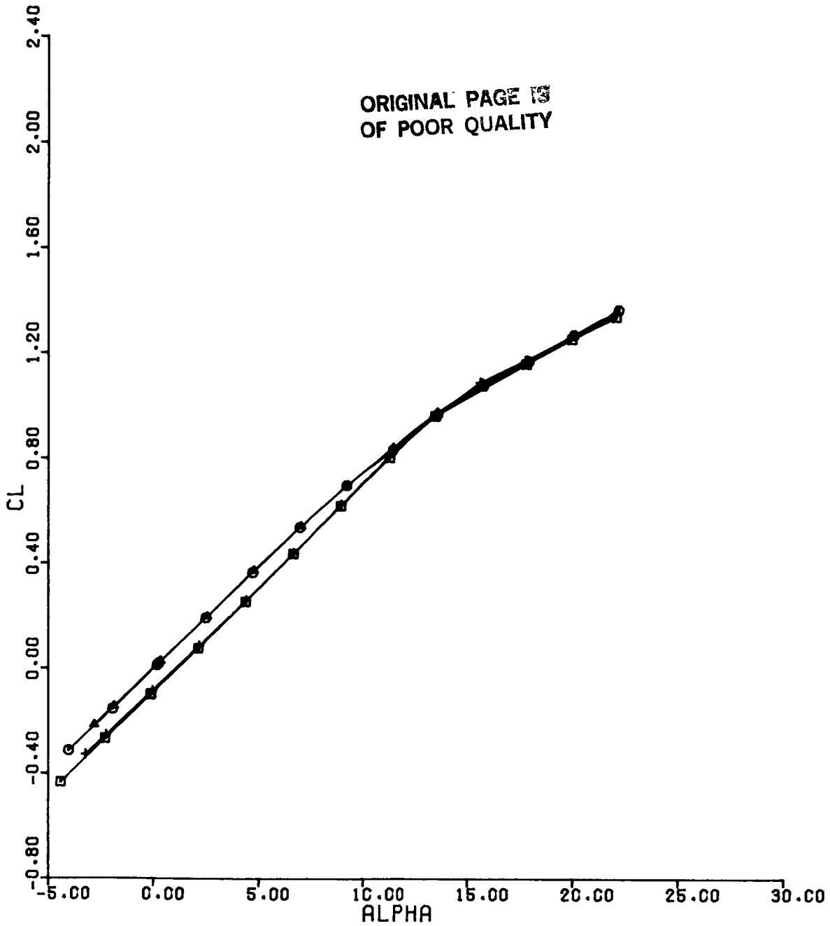
Figure 5(a). CL vs ALPHA Configuration 1, MACH = 0.6
