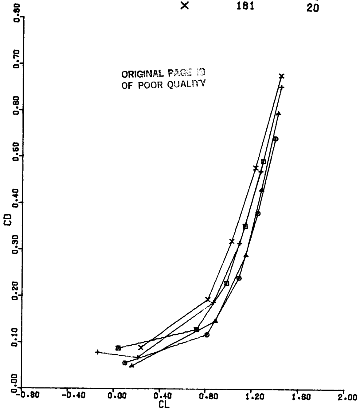
Figure 50(b). CD vs CL Configuration 4, BETA = 0, MACH = 0.6
