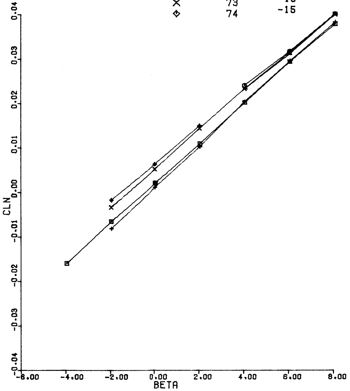
Figure 20(b). CLN vs BETA, DCR = 0, Configuration 1, ALPHA = 15, MACH = 0.6
