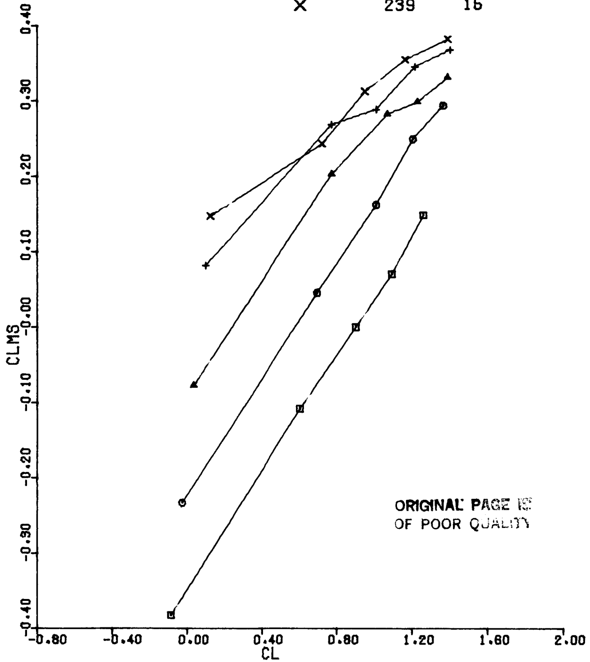
Figure 65(c). CLMS vs CL Configuration 6, BETA = 0, MACH = 0.6
