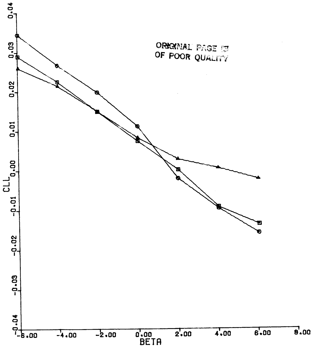
Figure 62(a). CLL vs BETA Configuration 5, ALPHA = 15, MACH = 0.9
