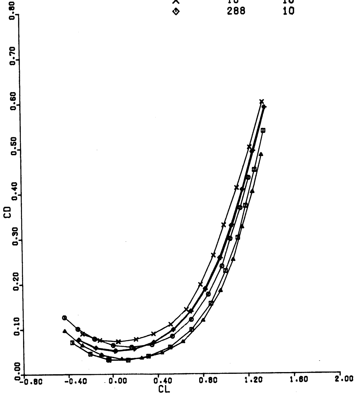
Figure 1(b). CD vs CL Configuration 1, MACH = 0.6, BETA = 0
