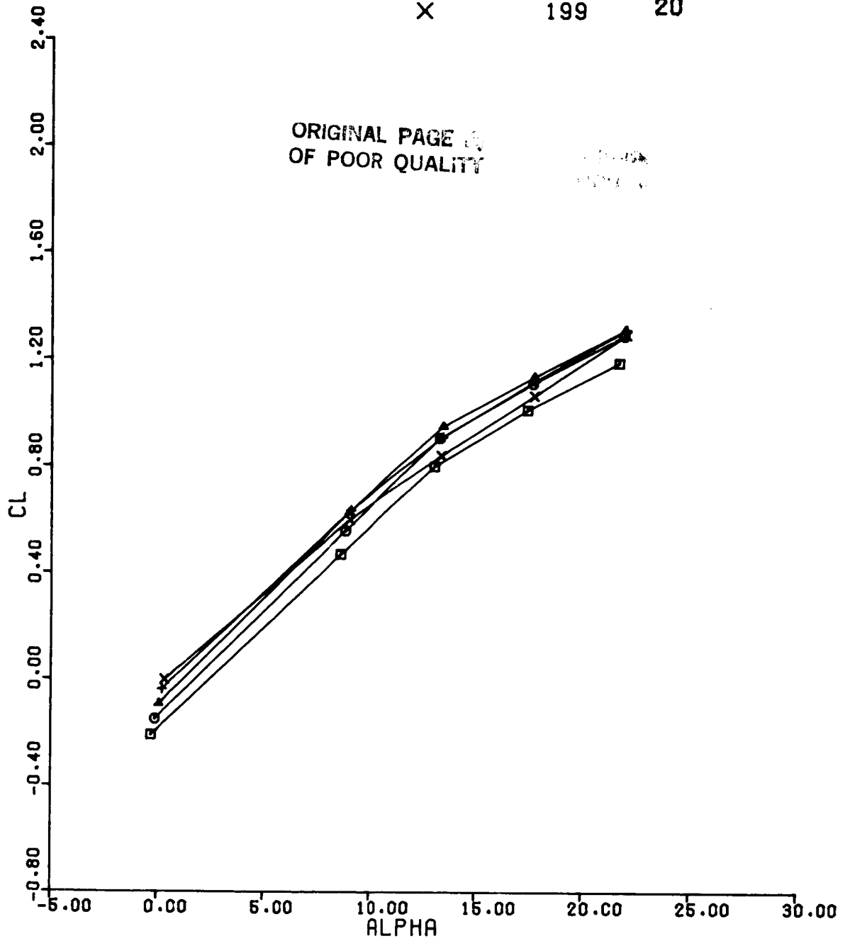
Figure 55(a). CL vs ALPHA Configuration 5, BETA = 0, MACH = 0.6
