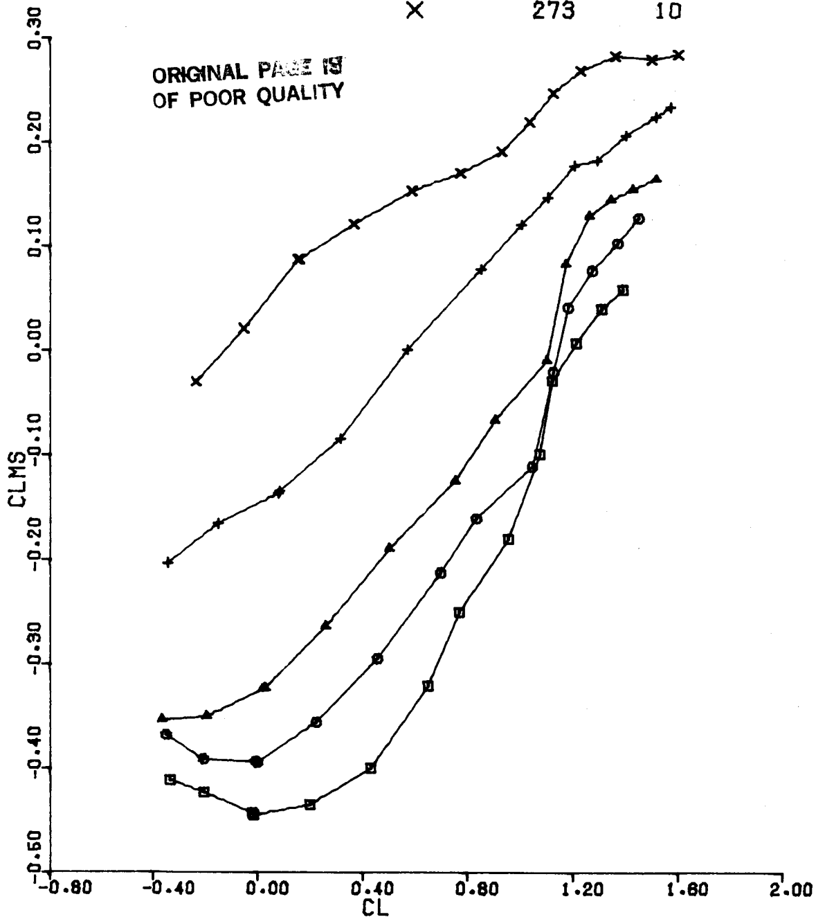
Figure 74(c). CLMS vs CL Configuration 8, BETA = 0, MACH = 0.9
