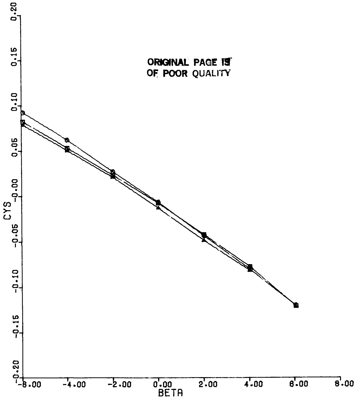
Figure 70(c). CYS vs BETA Configuration 6, ALPHA = 15, MACH = 0.6
