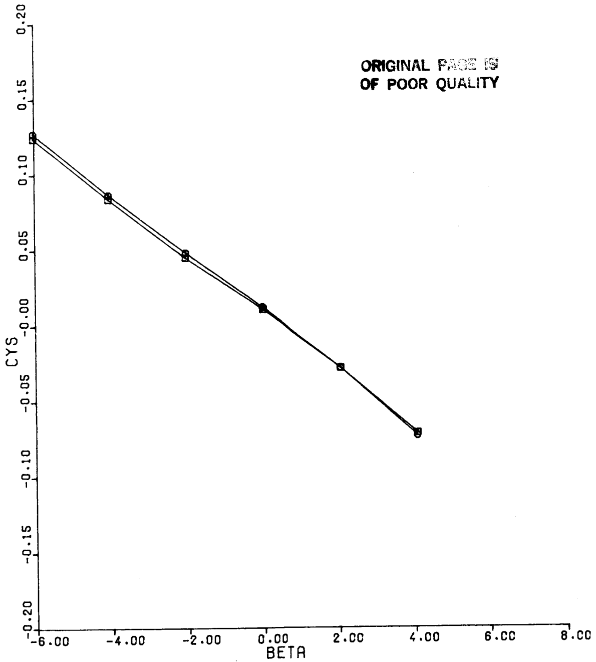
Figure 35(c). CY5 vs BETA, DC = 10, Configuration 2, ALPHA = 10, MACH = 0.6
