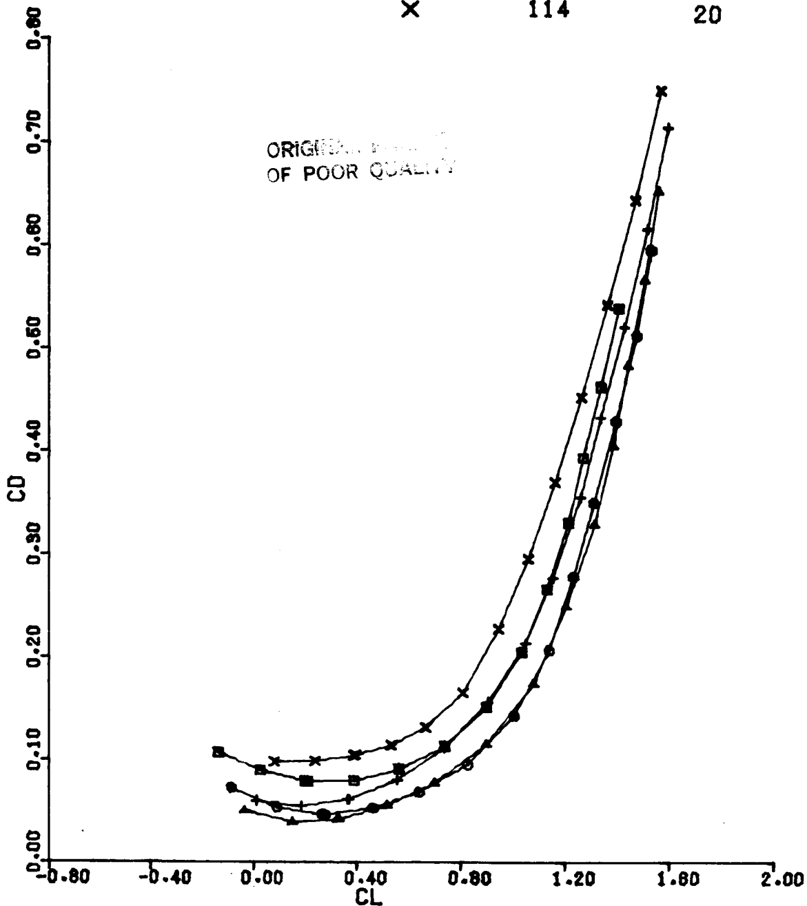
Figure 27(b). CD vs CL, DS = 5, Configuration 2, BETA = 0, MACH = 0.6
