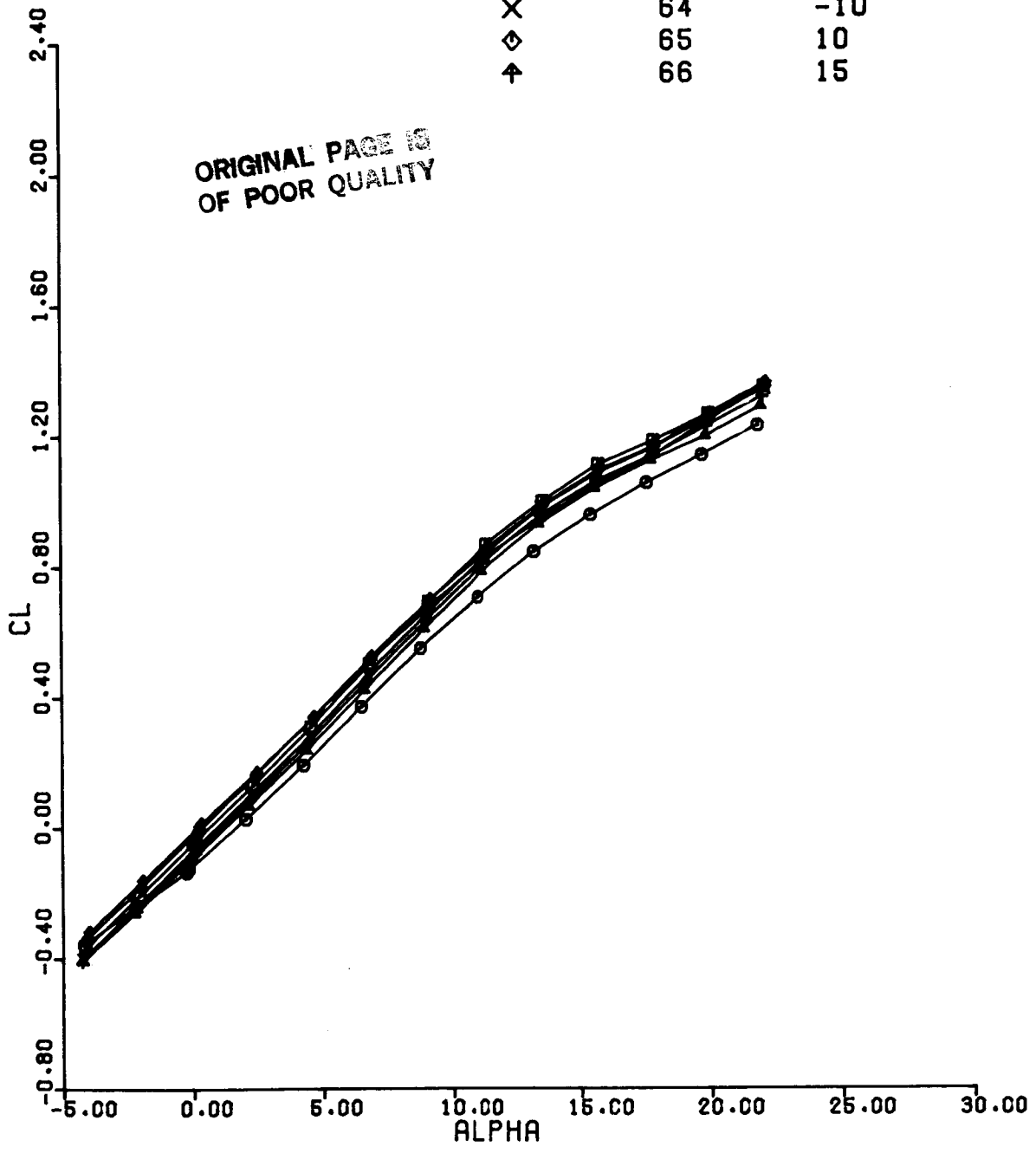
Figure 15(a). CL vs ALPHA, DCR = 0, Configuration 1, MACH = 0.6, BETA = 0
