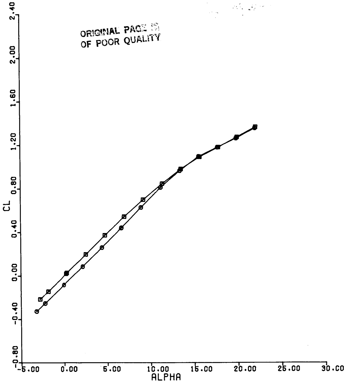
Figure 2(a). CL vs ALPHA Configuration 1, MACH = 0.6, BETA = 4
