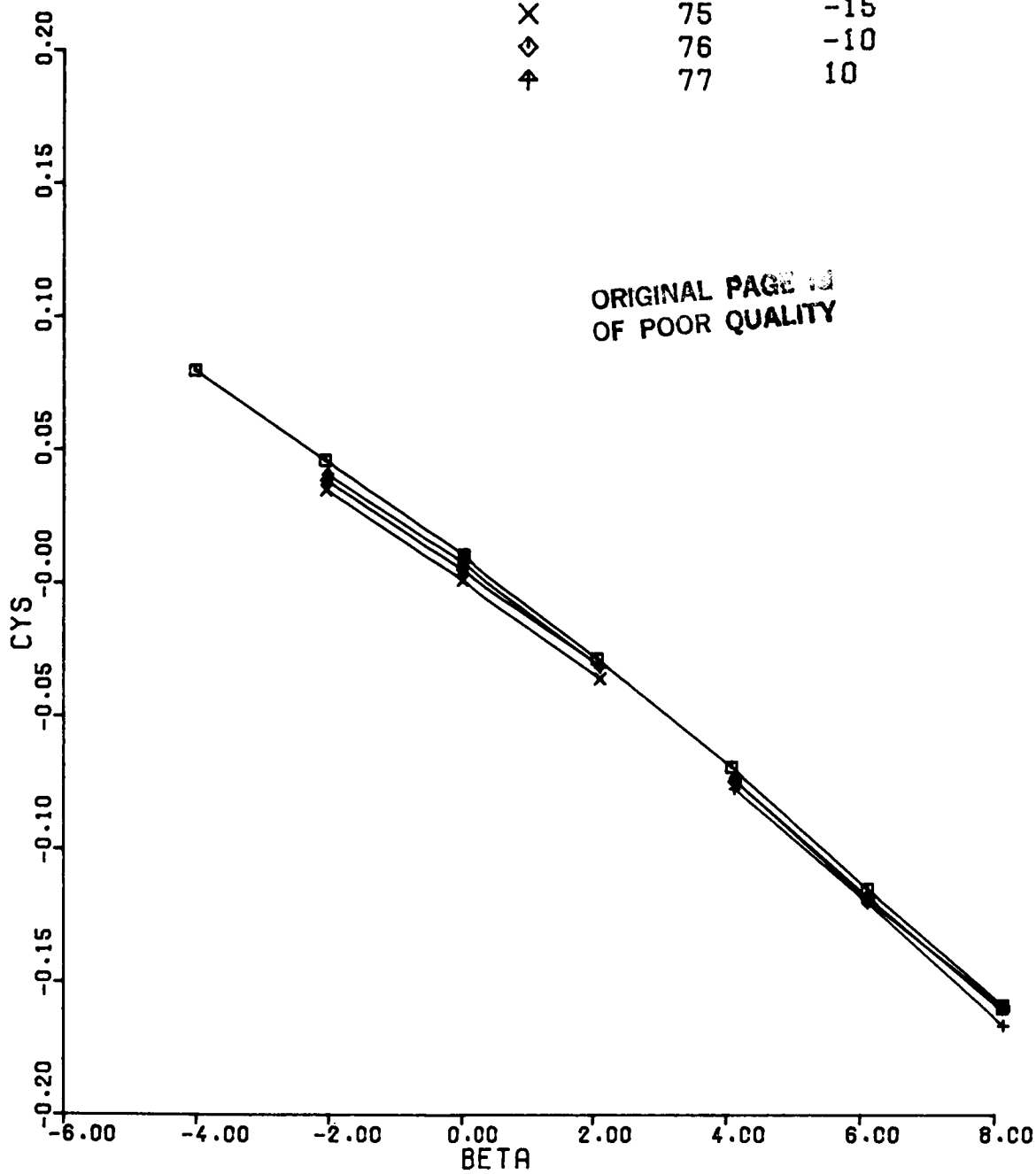
Figure 19(c). CYS vs BETA Configuration 1, ALPHA = 10, MACH = 0.6
