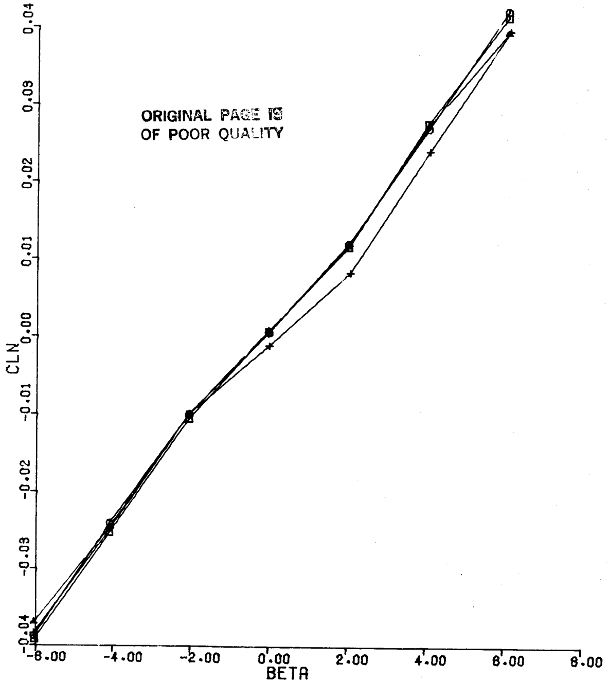
Figure 81(b). CLN vs BETA Configuration 8, ALPHA = 11, MACH = 1.2
