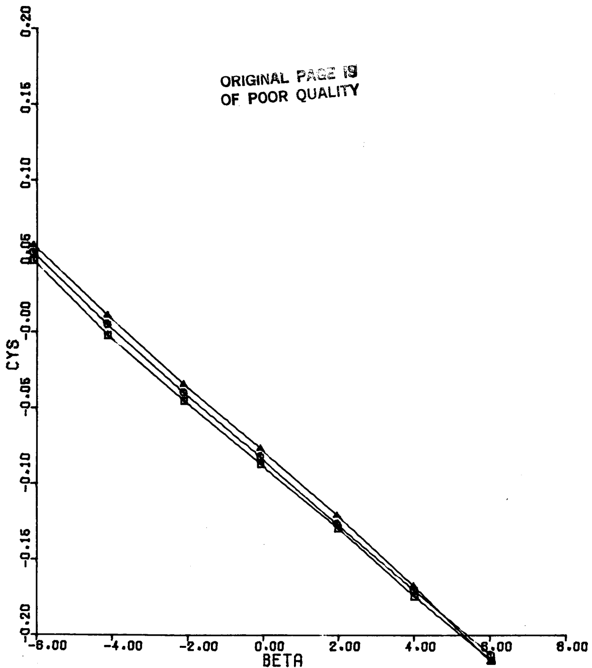
Figure 89(c). CYS vs BETA Configuration 9, ALPHA = 10, MACH = 0.6
