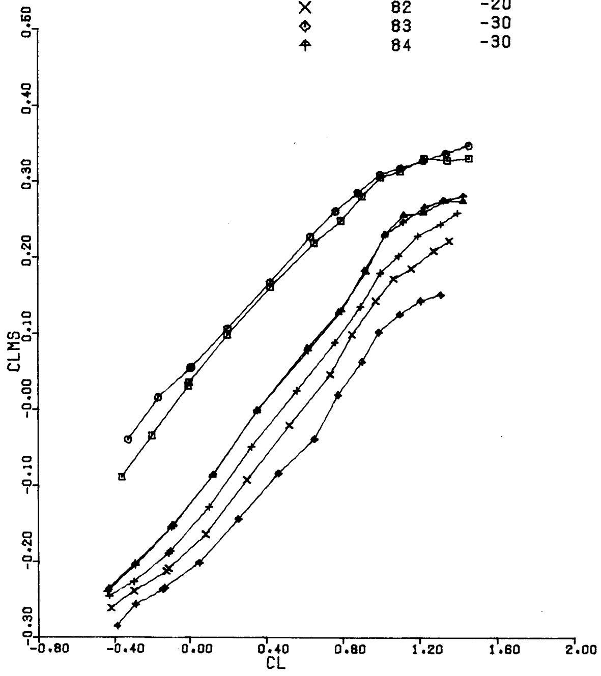
Figure 16(c). CLMS vs CL Configuration 1, MACH = 0.9, BETA = 0
