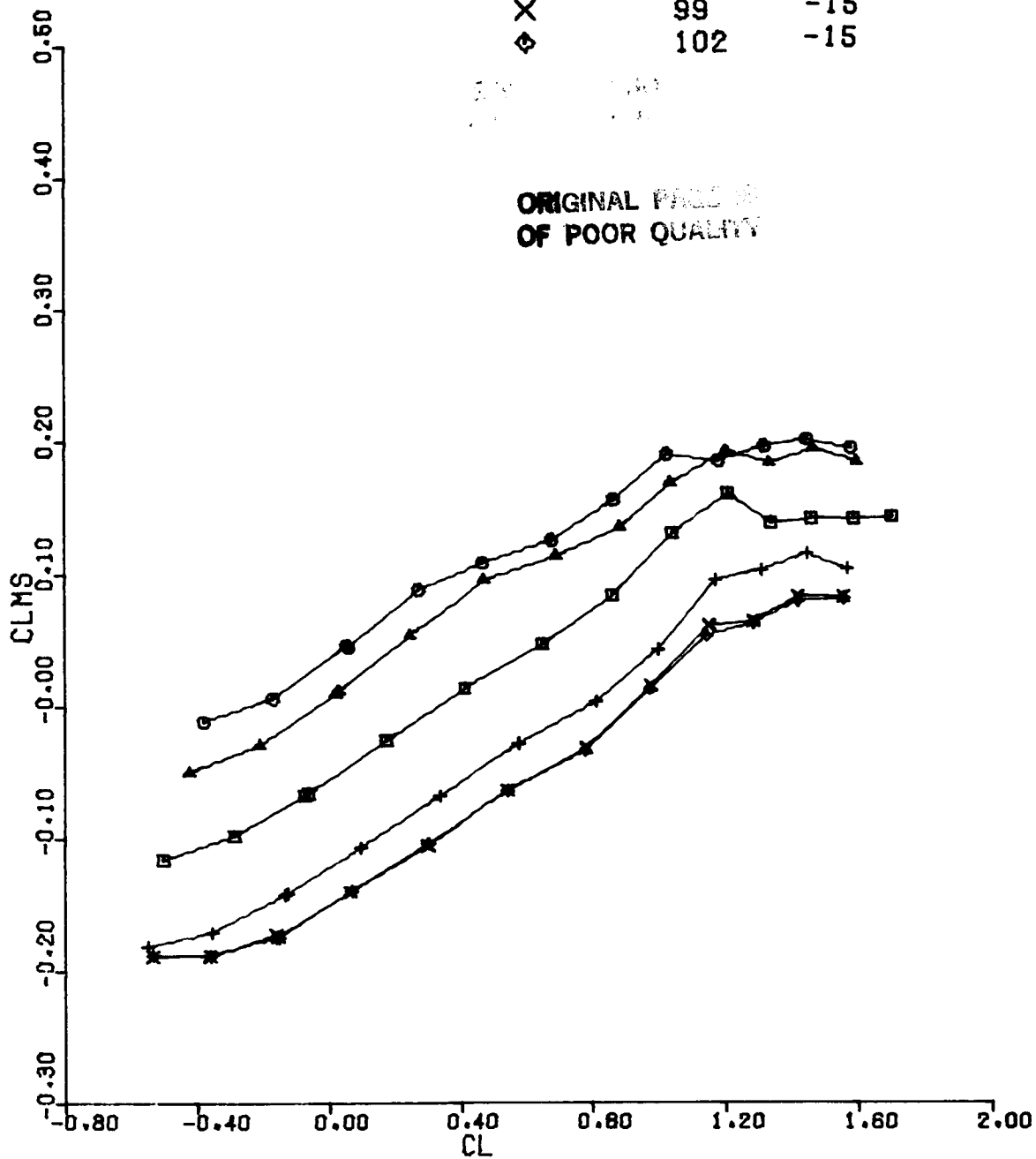
Figure 17(c). CLMS vs CL, DCR = 0, Configuration 1, MACH = 1.2, BETA = 0
