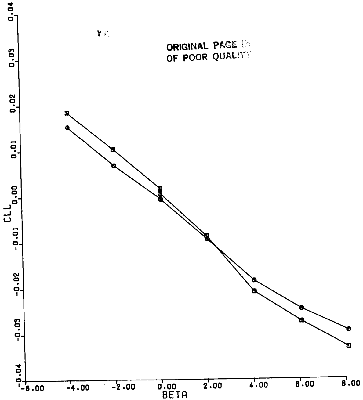
Figure 8(a). CLL vs BETA Configuration 1, MACH = 0.6, DC = 0
