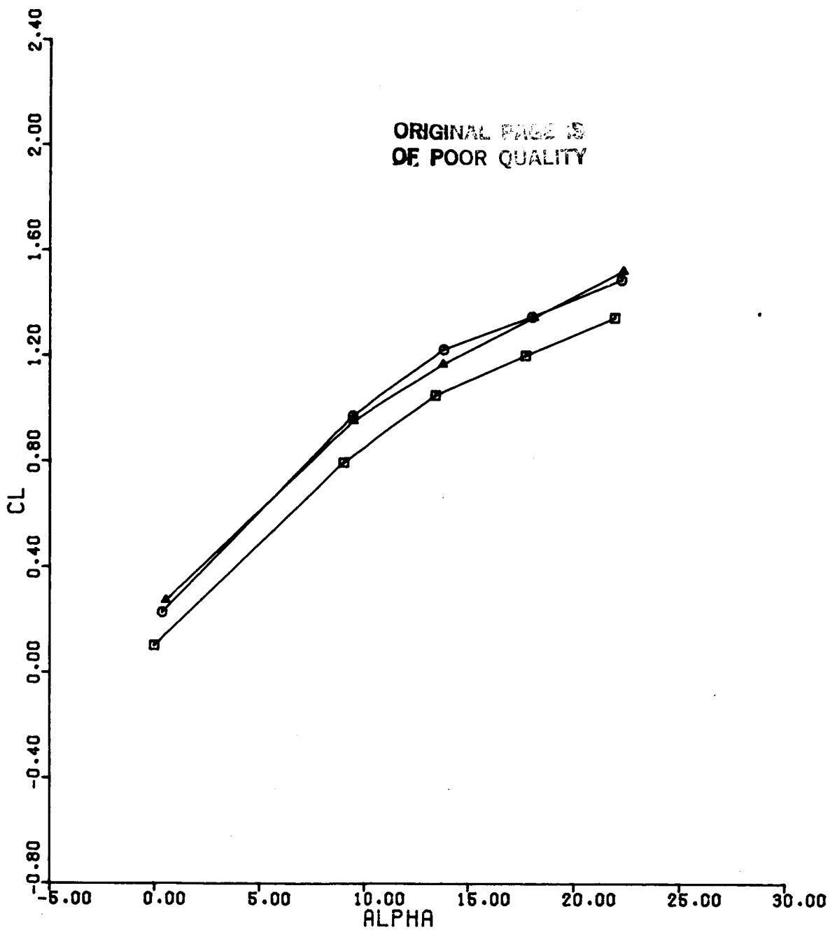
Figure 85(a). CL vs ALPHA Configuration 9, BETA = 0, MACH = 0.6
