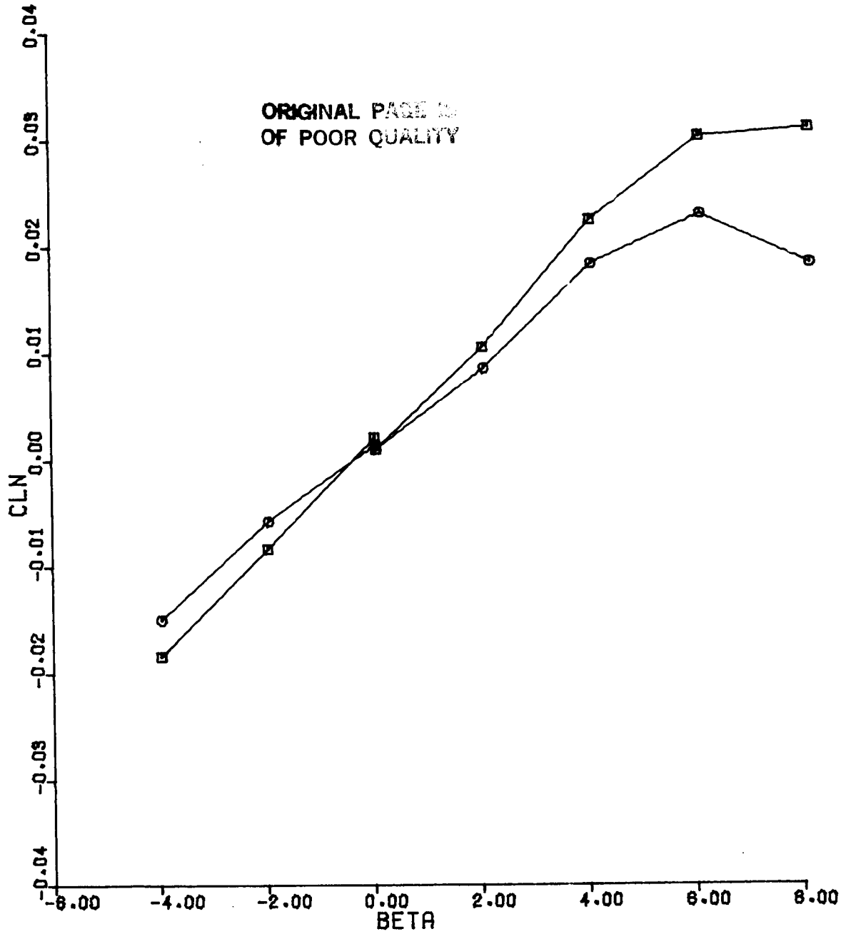
Figure 25(b). CLN vs BETA Configuration 1, MACH = 0.9, DC = 0
