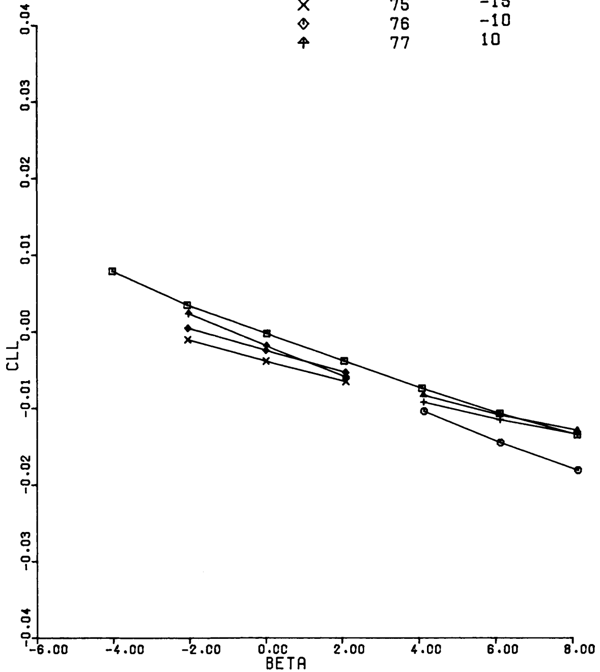
Figure 19(a). CLL vs BETA, DCR = 0, Configuration 1, ALPHA = 10, MACH = 0.6
