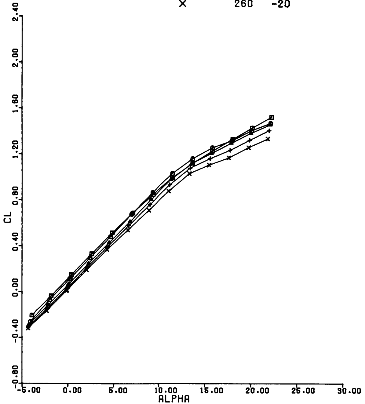
Figure 73(a). CL vs ALPHA Configuration 8, BETA = 0, MACH = 0.6
