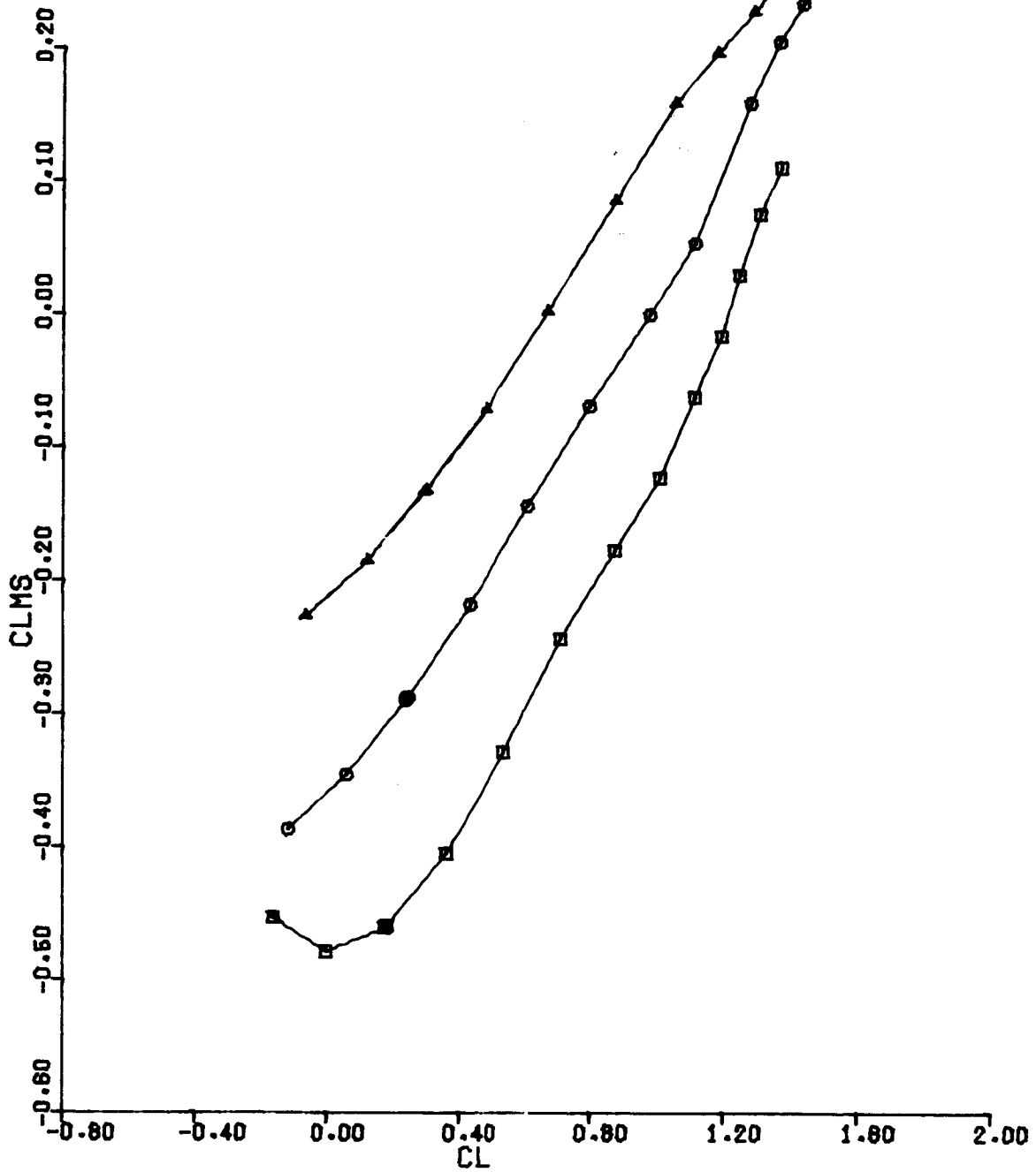
Figure 29(c). CLMS vs CL, DS = -5, Configuration 2, BETA = 0, MACH = 0.6
