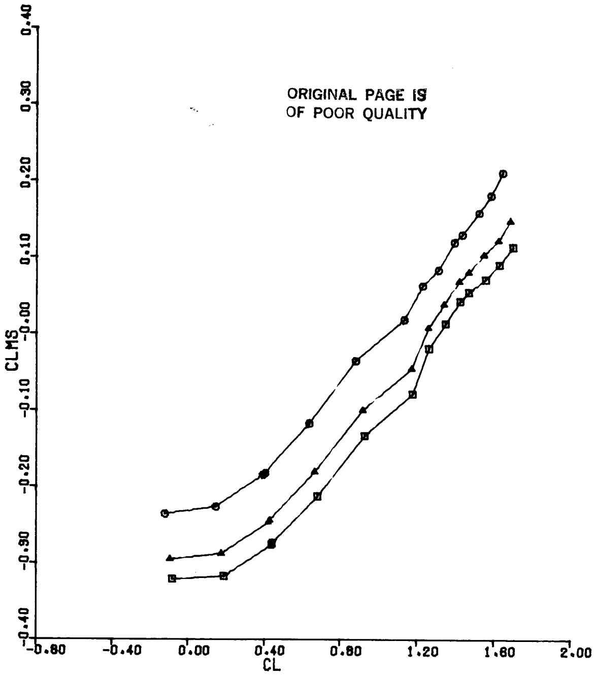
Figure 49(c). CLMS vs CL, DC = 0, Configuration 3, BETA = 0, MACH = 0.9
