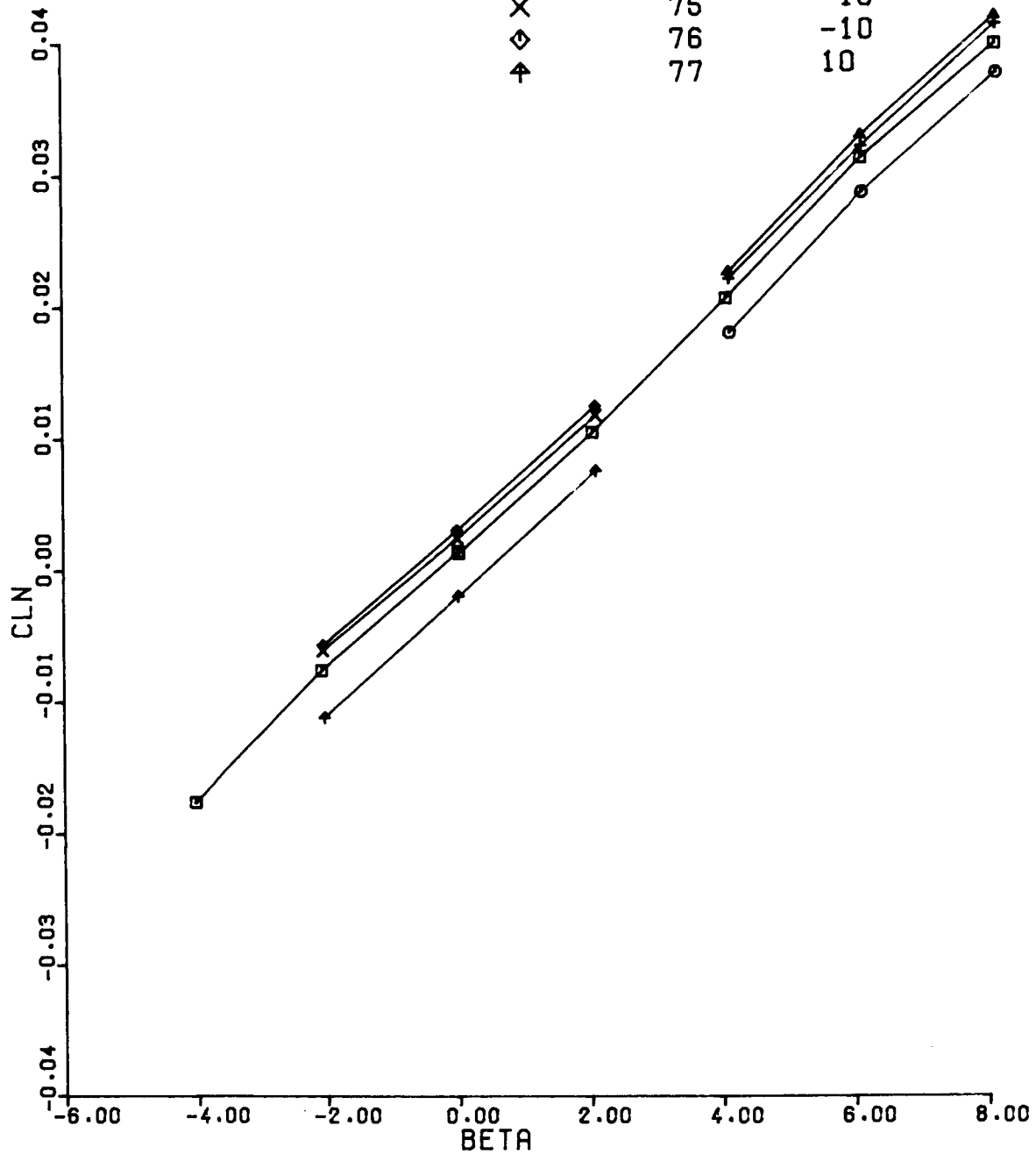
Figure 19(b). CLN vs BETA, DCR = 0, Configuration 1, ALPHA = 10, MACH = 0.6
