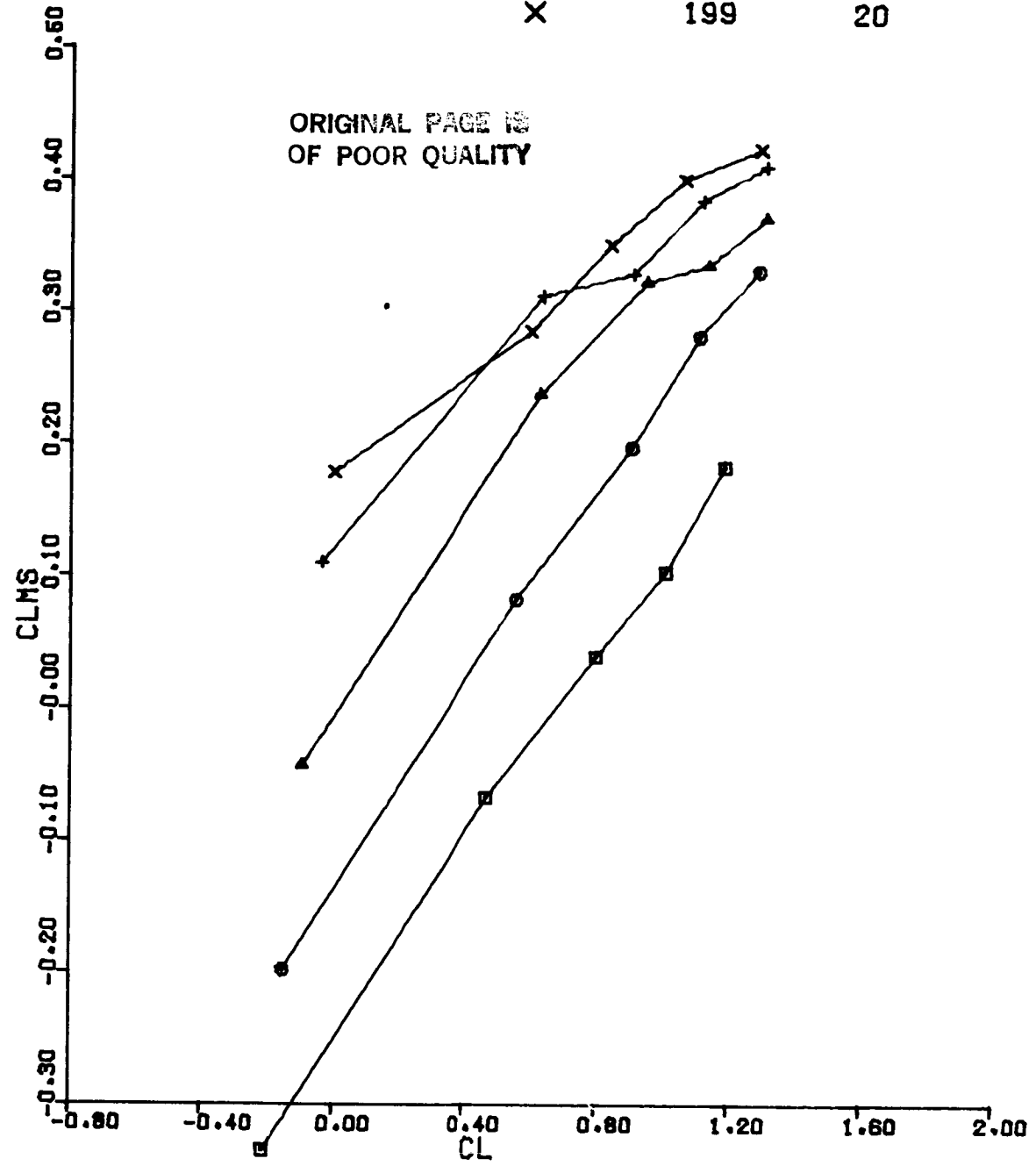
Figure 55(c). CLMS vs CL Configuration 5, BETA = 0, MACH = 0.6
