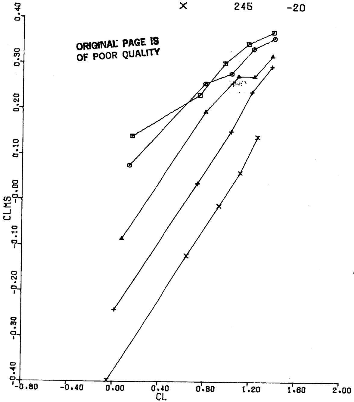
Figure 71(c). CLMS vs CL Configuration 7, BETA = 0, MACH = 0.6
