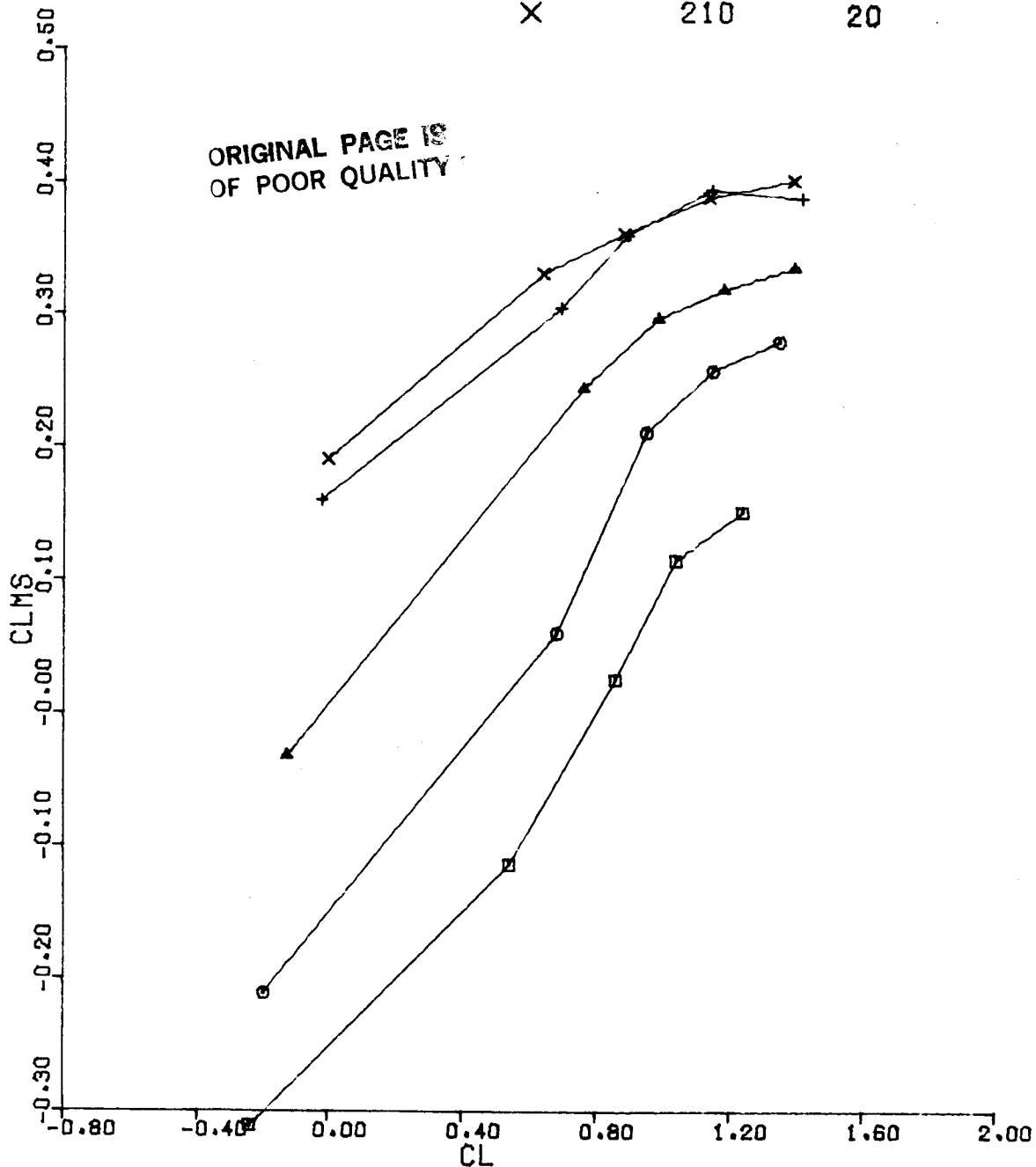
Figure 56(c). CLMS vs CL Configuration 5, BETA = 0, MACH = 0.9
