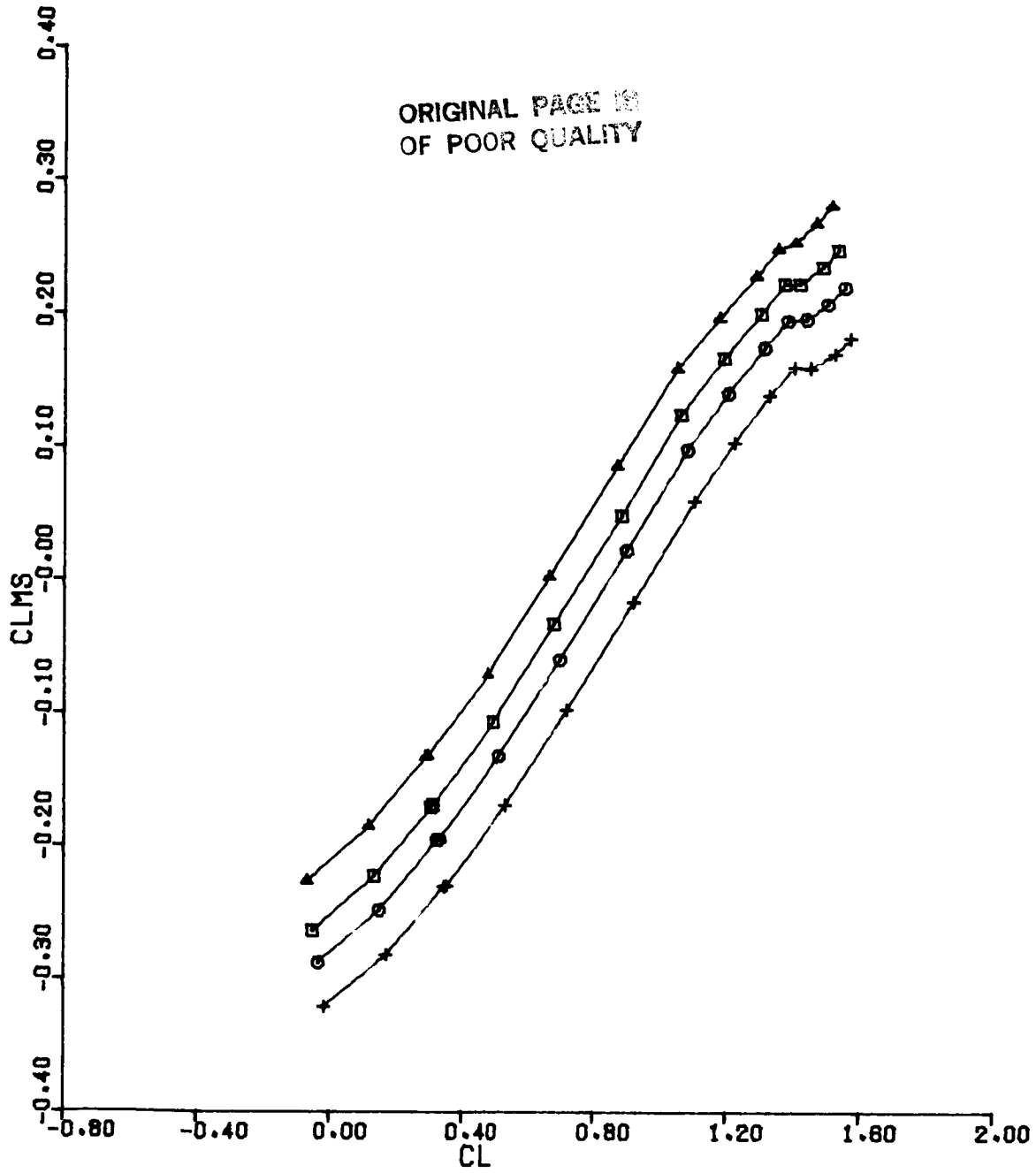
Figure 33(c). CLMS vs CL, DC = 0, Configuration 2, BETA = 0, MACH = 0.6
