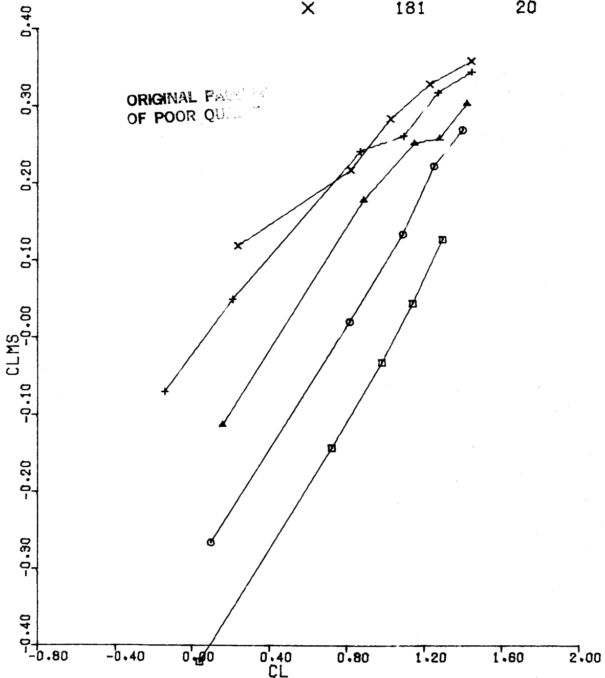
Figure 50(c). CLMS vs CL Configuration 4, BETA = 0, MACH = 0.6
