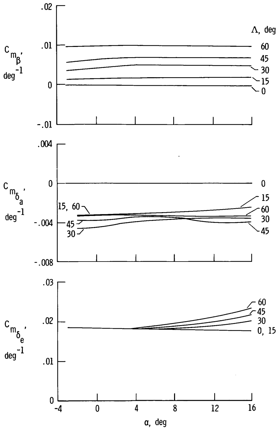
(b) C_{m\beta} , C_{m\delta_a} , and C_{m\delta_e} .
