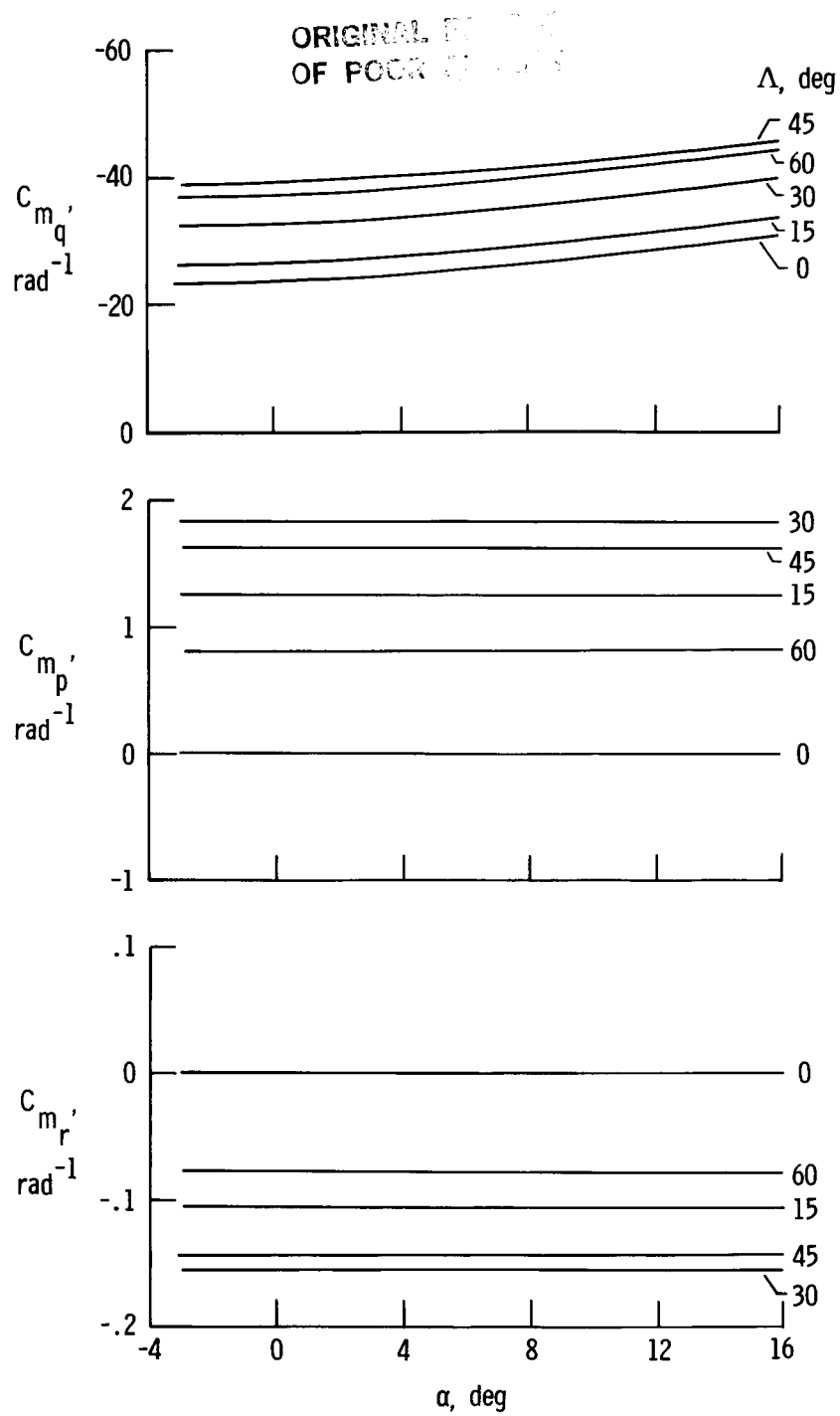
(c) C_{m_q}' , C_{m_p}' , and C_{m_r}' .
