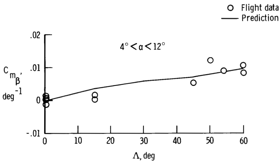
Figure 7. Estimates of C_{m_\beta} as obtained from sideslip variation analysis.
