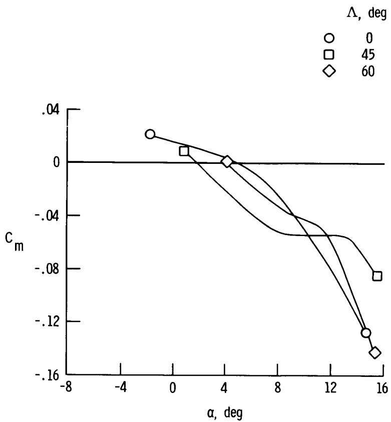
Figure 4. Pitching moment as a function of angle of attack for lg flight (from ref. 4). Controls zeroed, cg = 0.4c_r .
