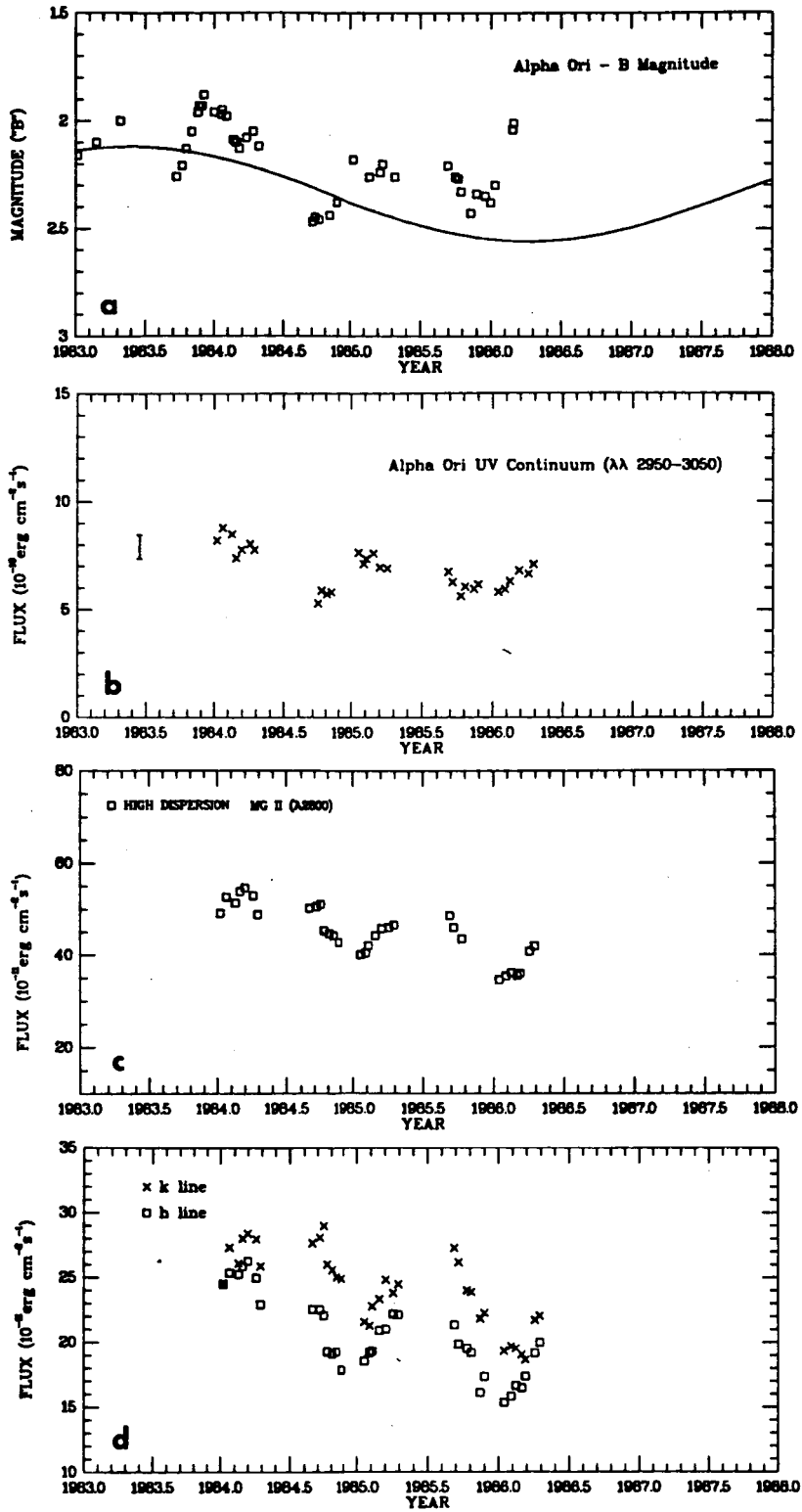
Figure 1. - B magnitude (a), ultraviolet continuum ( 3000 \pm 50 \text{ \AA} ) flux (b), total Mg II h and k line flux (c), and Mg II h and k line fluxes plotted separately (d) obtained during the 1984-1986 Alpha Ori monitoring program. The ultraviolet continuum flux \pm 2 -sigma error bar is shown in (b). The error in the Mg II fluxes is estimated to be less than four percent.
