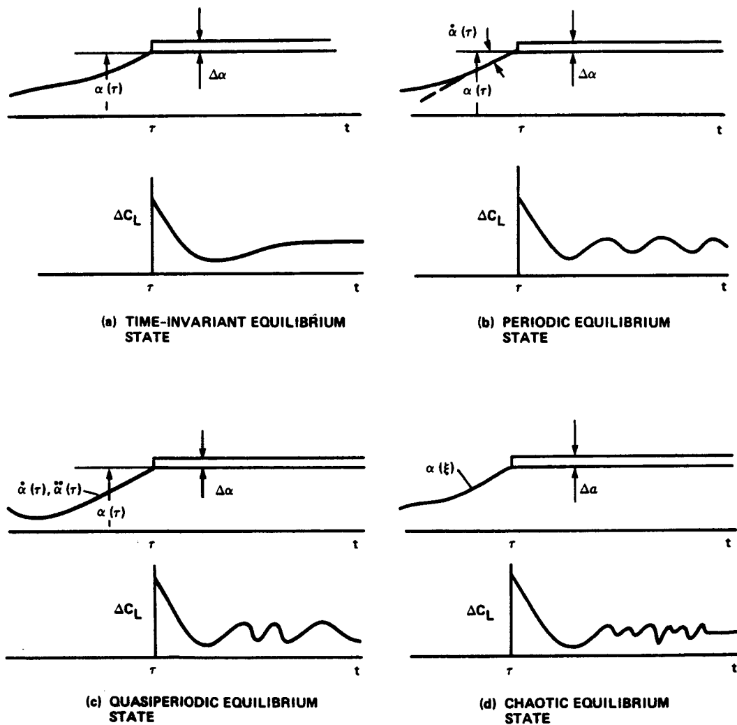
Fig. 6 Memory effects.
