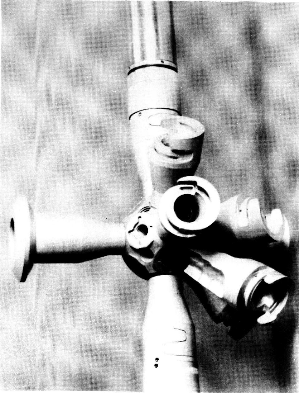
Fig. 7. 3-D Quick attachment erectable node.
