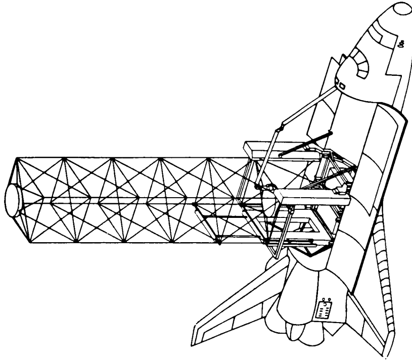
Five bays of erected truss
