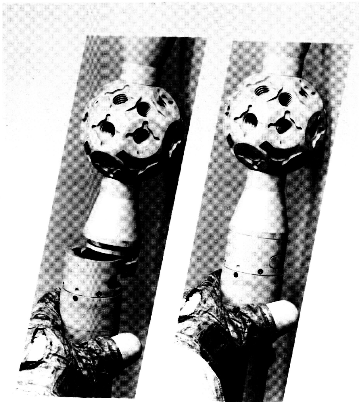
Fig. 15. Quick-attachment joints designed for astronaut glove handling.
