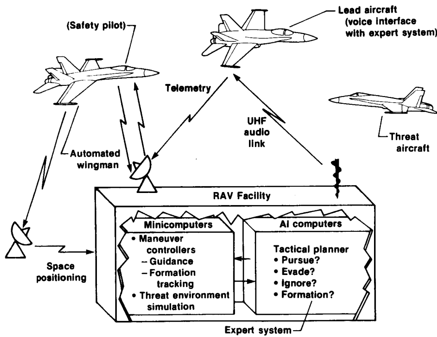
Figure 5. Flight evaluation system for automated wingman.
