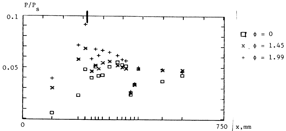
Fig. 65. P/X. Shock stabilised wall injection. 10^\circ shock. H_s = 4.2 MJ/kg, M_I = 3.5
