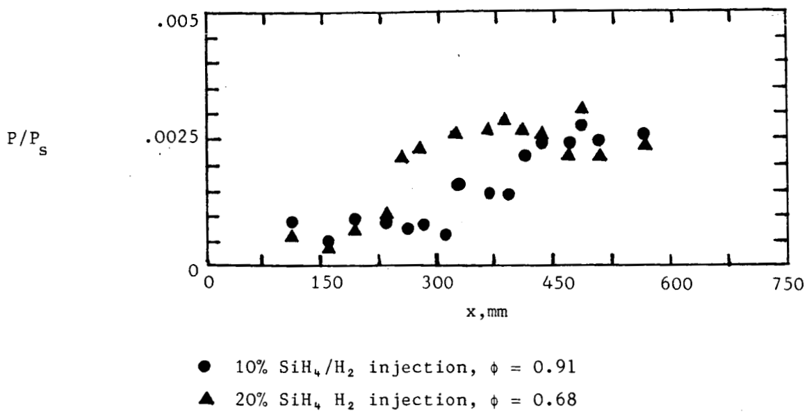
Fig. 15. Effect of concentration of silane on combustion at Mach 5, H_s = 2.65 MJ/kg, P_I = 20 kPa, T_I = 410 K.
