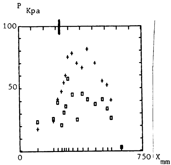
■ \phi = 0 + \phi = 6.1 A. H_s = 8.7 MJ/kg
