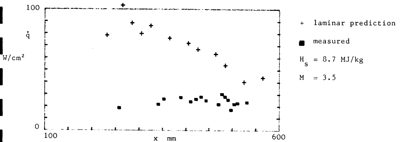
Fig. 34b. Predicted and measured values of the heat transfer rate for a 15^\circ diverging duct with injector.
