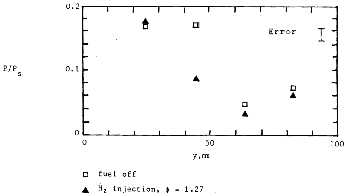
Fig. 25. Pitot profiles across an open duct with 15 degrees divergence, H_s = 8.7 MJ/kg, M_I = 3.5 , T_I = 2500 K, P_I = 160 kPa
