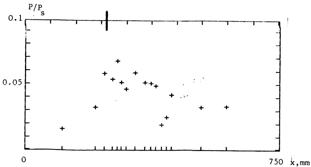
Fig. 63. P/X. Shock stabilised wall injection. 10^0 shock. M_I = 3.5 . H_s = 8.7 MJ/kg. \phi = 0.91 .
