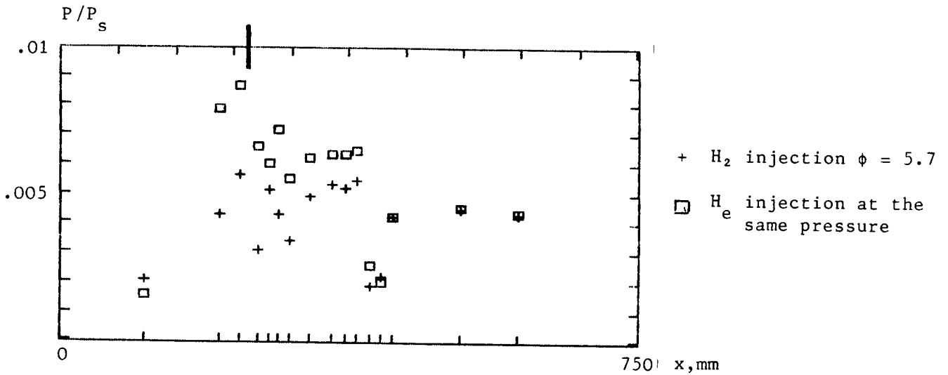
Fig. 62. P/X shock stabilised wall injection. 10^0 shock. M_I = 5 , H_s = 8.7 MJ/kg. Comparison at H_e and H_2 injection.
