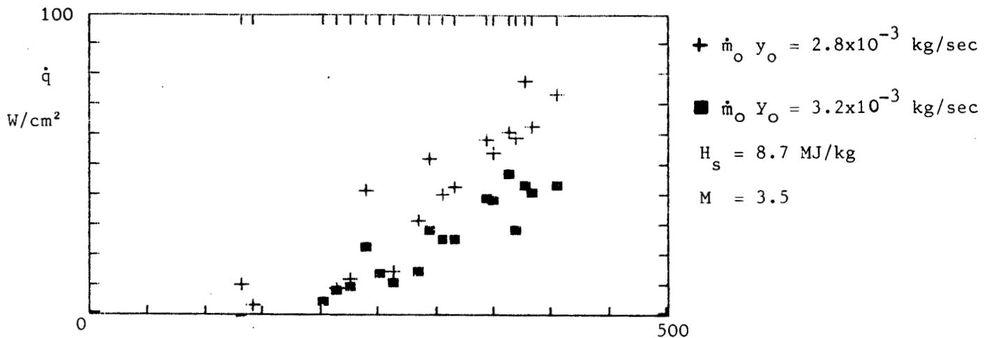
Fig. 45. Heat transfer rates for the injection of nitrogen into air and hydrogen into nitrogen at similar values of \dot{m}_0 y_0 .
