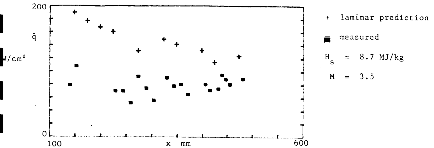
Fig. 34a. Predicted and measured values of the heat transfer rate for a constant area duct with injector.
