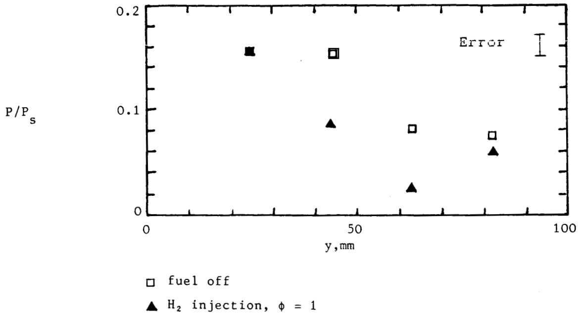
Fig. 24. Pitot profiles across an open duct with 15 degrees divergence, H_s = 6.1 MJ/kg, M_I = 3.5 , T_I = 1700 K, P_I = kPa
