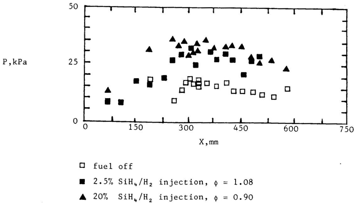
Fig. 12. Effect of concentration of silane on combustion at Mach 5, H_s = 6.1 MJ/kg, P_I = 20 kPa, T_I = 1000 K (Note: Pressure is absolute due to lack of stagnation pressure information)
