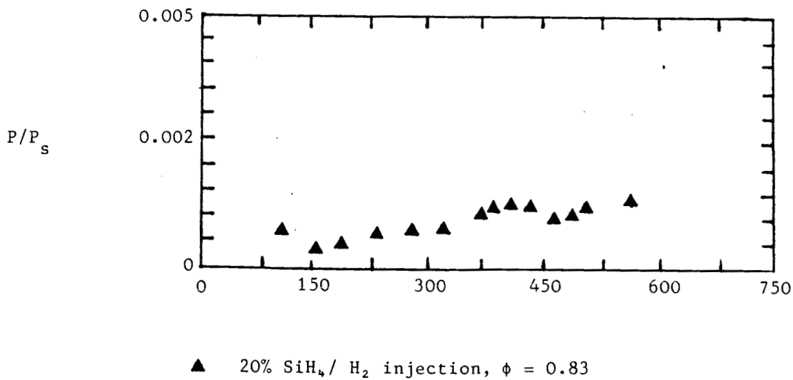
Fig. 16. Combustion limit of 20% SiH 4 /H 2 at Mach 5, H_s = 1.90 MJ/kg, T_I = 350 K.
