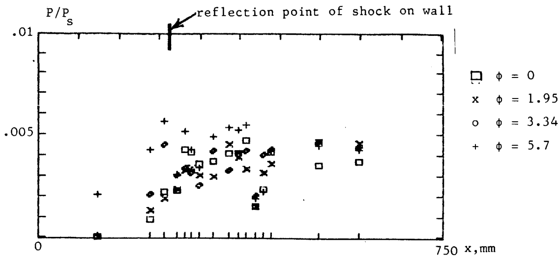
Fig. 61 P/X shock stabilised wall injection. 10^0 shock. H_s = 8.7 MJ/kg, M_I = 5
