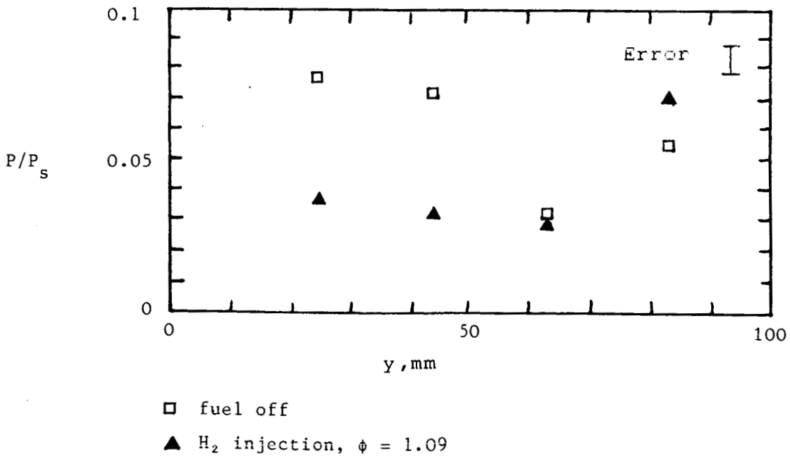
Fig. 27. Pitot profiles across a symmetrical duct, 15 degree divergence, H_s = 8.7 \text{ MJ/kg} , M_I = 3.5 , T_I = 2500 \text{ K} , P_I = 160 \text{ kPa}
