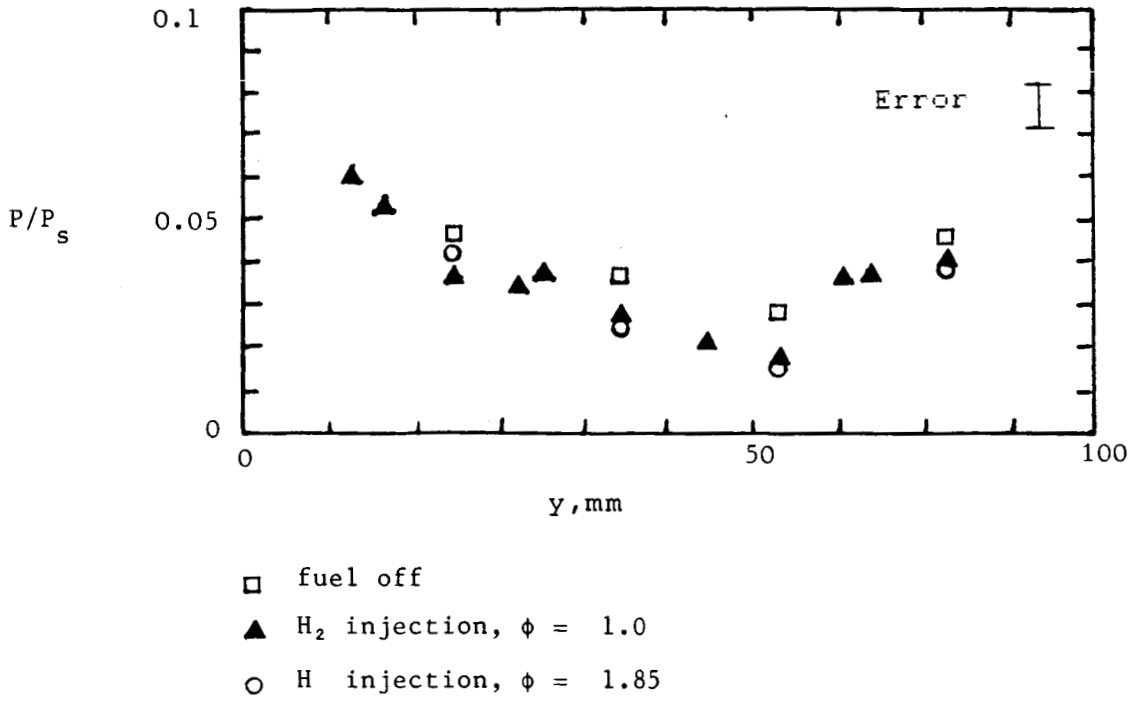
Fig. 26. Pitot profiles across a closed duct with 15 degrees with divergence, H_s = 8.7 \text{ MJ/kg} , M_I = 3.5 , T_I = 2500 \text{ K} , P_I = 160 \text{ kPa}
