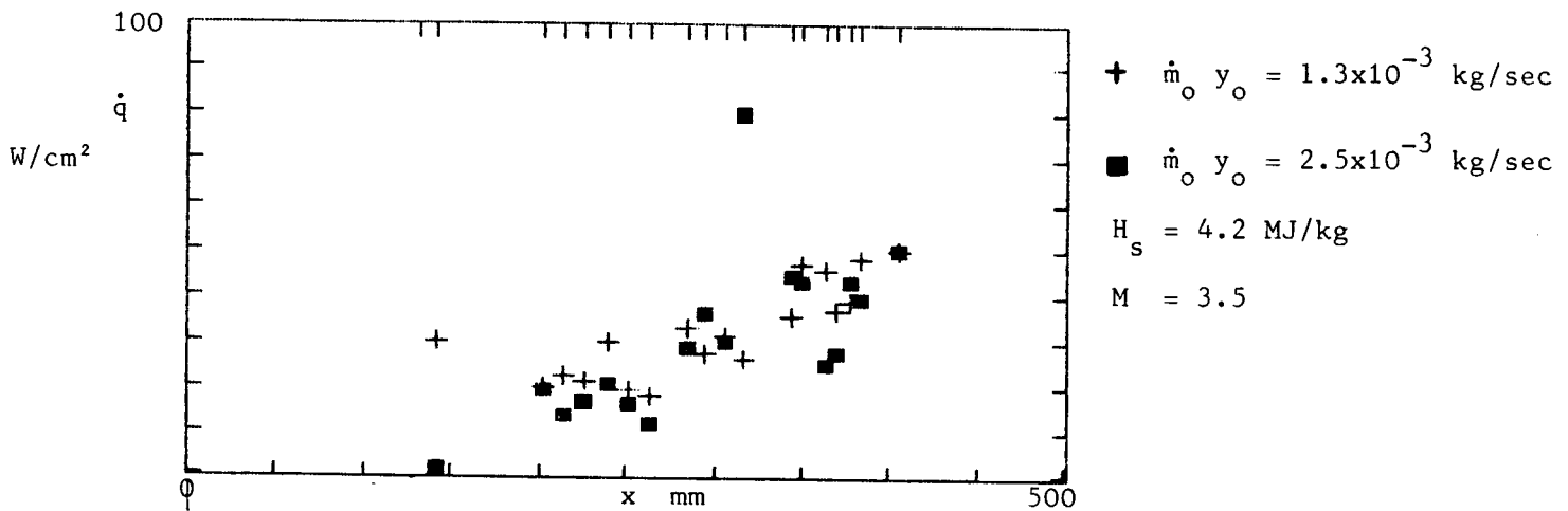
Fig. 39. Heat transfer rates in a constant area duct when dydeogen is injected into a nitrogen test gas with different injectors.
