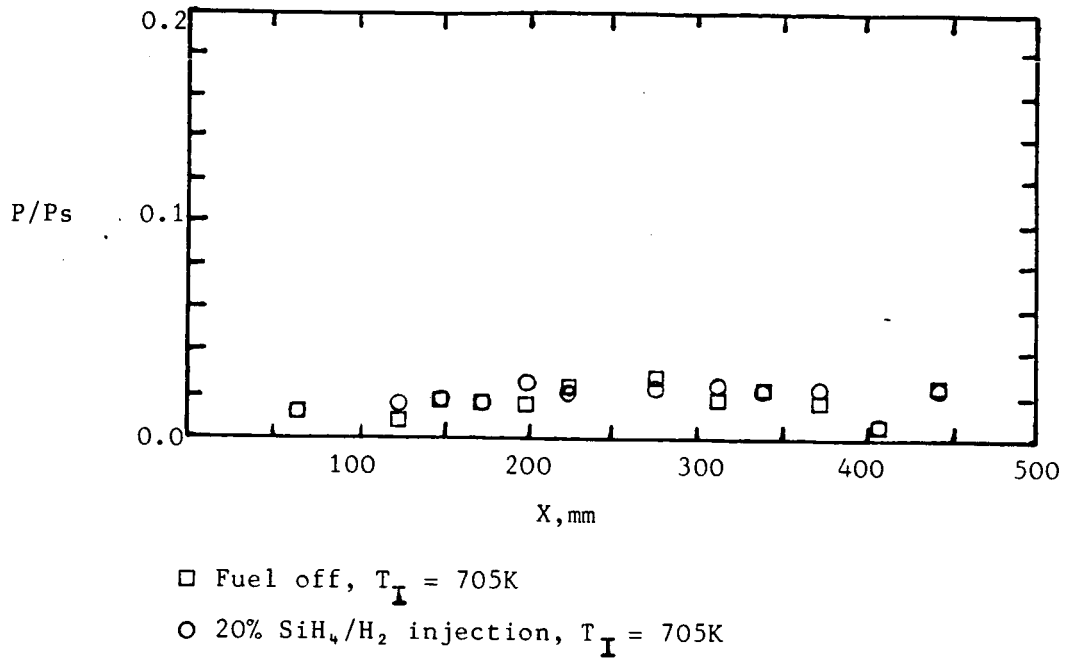
Fig. 5. Ignition limit of 20% SiH_4/H_2 mixture at mach 3.3, P_I = 15kPa , \phi = 0.78
