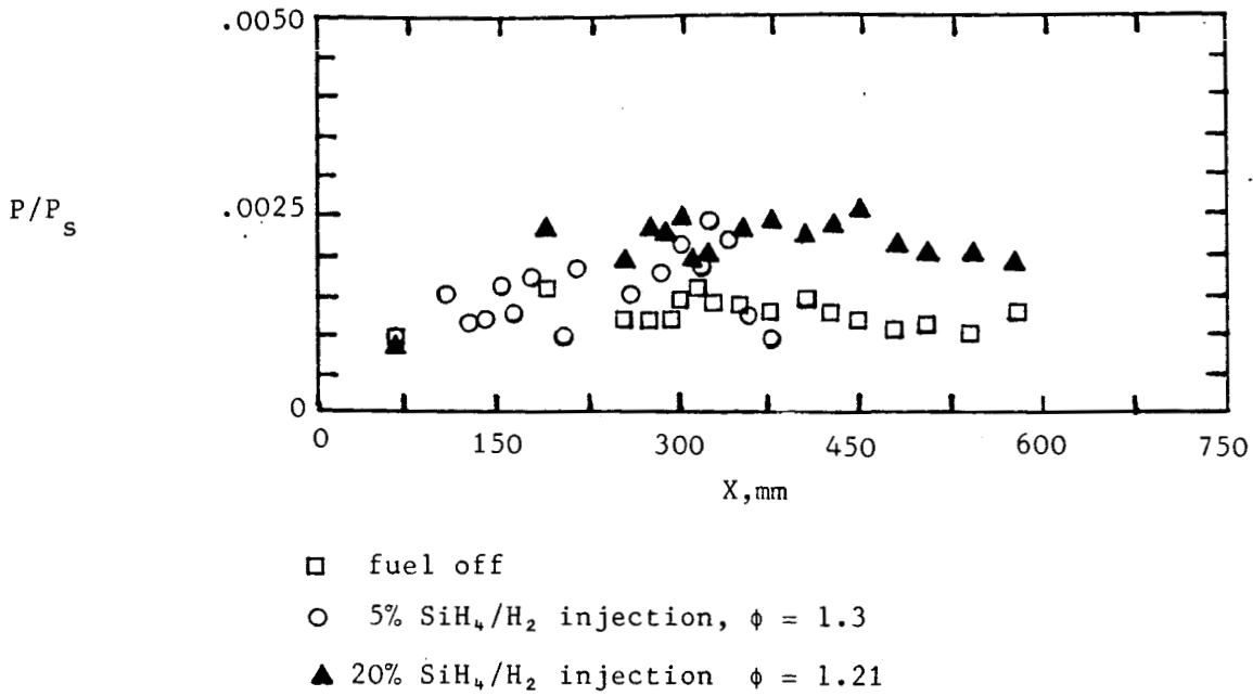
Fig. 11. Effect of concentration of silane on combustion at Mach 5, H_s = 8.7 MJ/kg, P_I = 20 kPa, T_I = 1500 K
