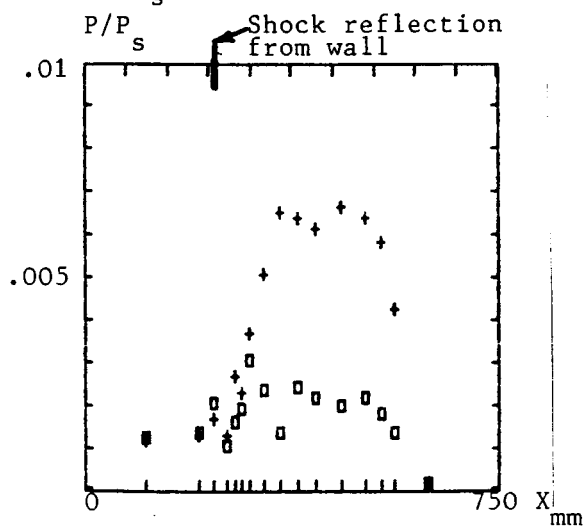
■ \phi = 0 + \phi = 3.8 E. H_s = 2.3 MJ/kg, fuel on
