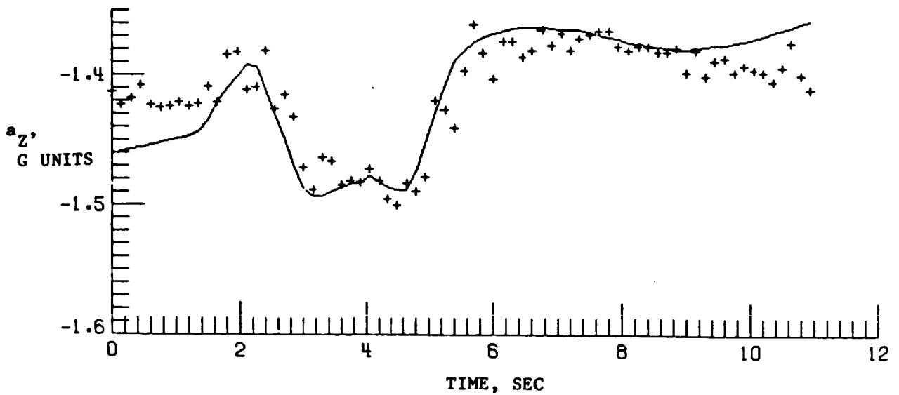
Figure 6. - Prediction of vehicle motion using linear model (only C_{m\delta e} included in model).
