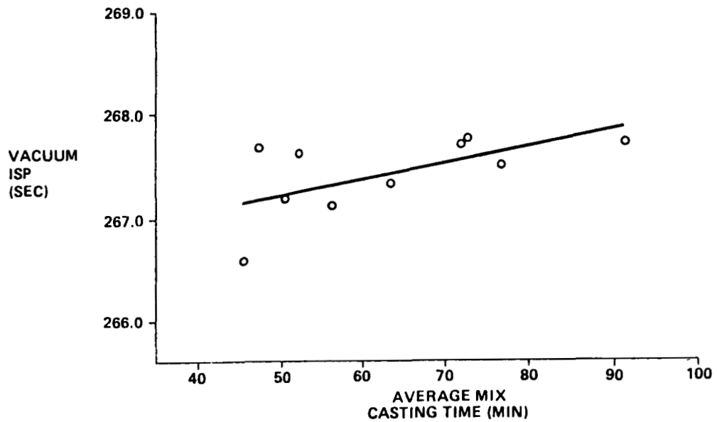
Figure 11. Flight average burn rate scale factors for SRMs manufactured with Pacific Engineering AP.
