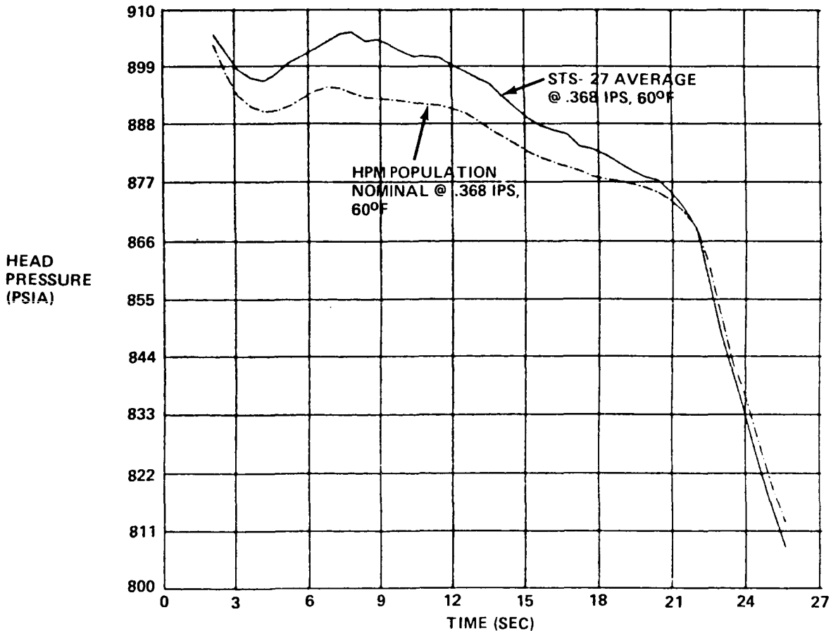
Figure 3. Comparison of average head pressure of STS-27 left/right SRM to population nominal at burn rate of 0.368 IPS and PMBT = 60°F.
