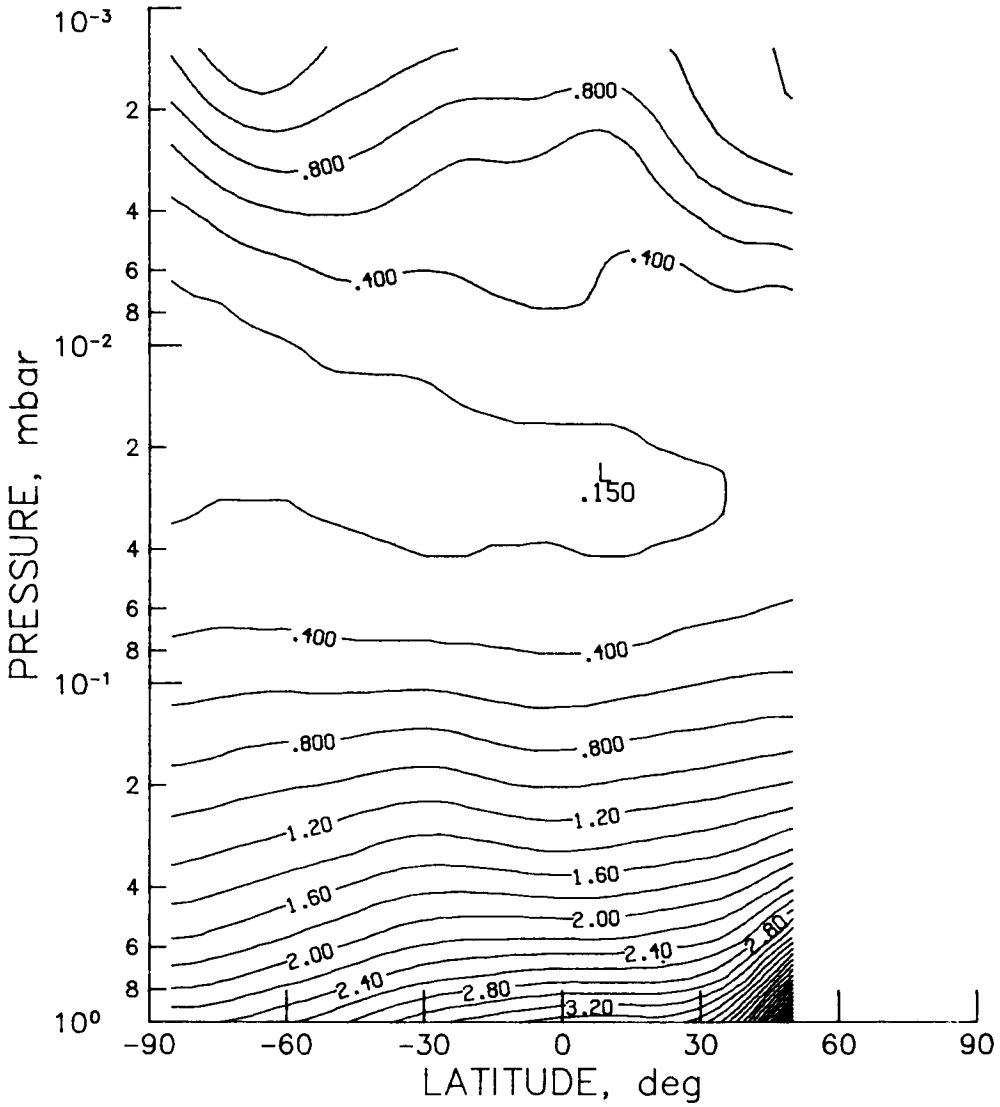
Figure O 3 -120 - SME monthly zonal mean ozone cross section for December 1982 using IR measurements (contour interval is 0.2 ppbv).
