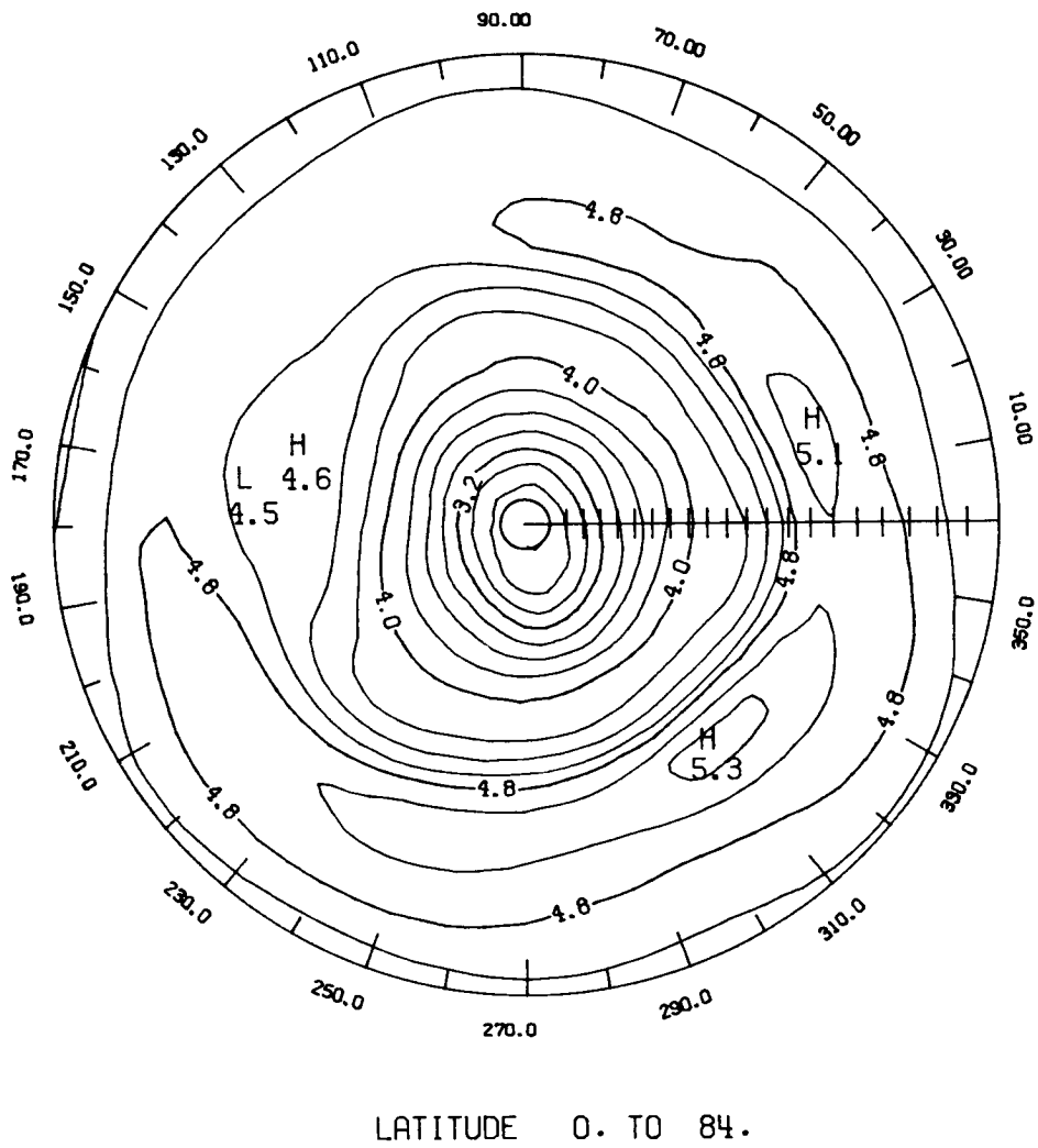
Figure O3-24 - LIMS ozone monthly mean polar stereographic projection at 30 mb for November 1978 (contour interval is 0.2 ppbv).
