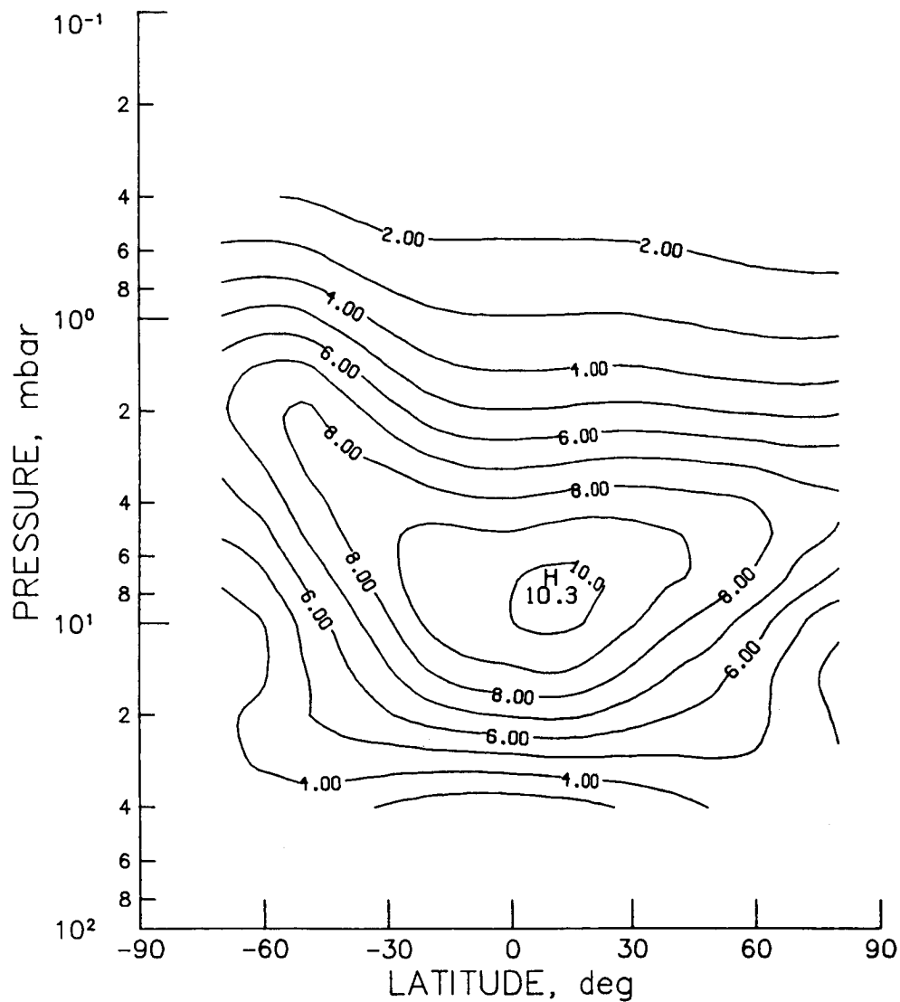
Figure O3-37 - SBUV monthly zonal mean ozone cross section for May 1979 (contour interval is 1.0 ppmv).
