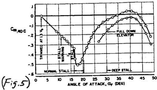
第5図 Pitching-moment coefficients for DC-9-10 configuration. Flaps 50°
