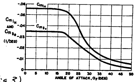
第3図 Stabilizer and elevator effectiveness
