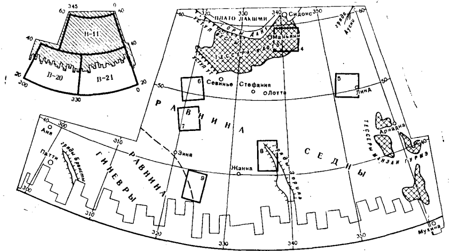
Fig. 3. Scheme of geographic names and location of map sheets. Shaded territory is shown in Fig. 2.
