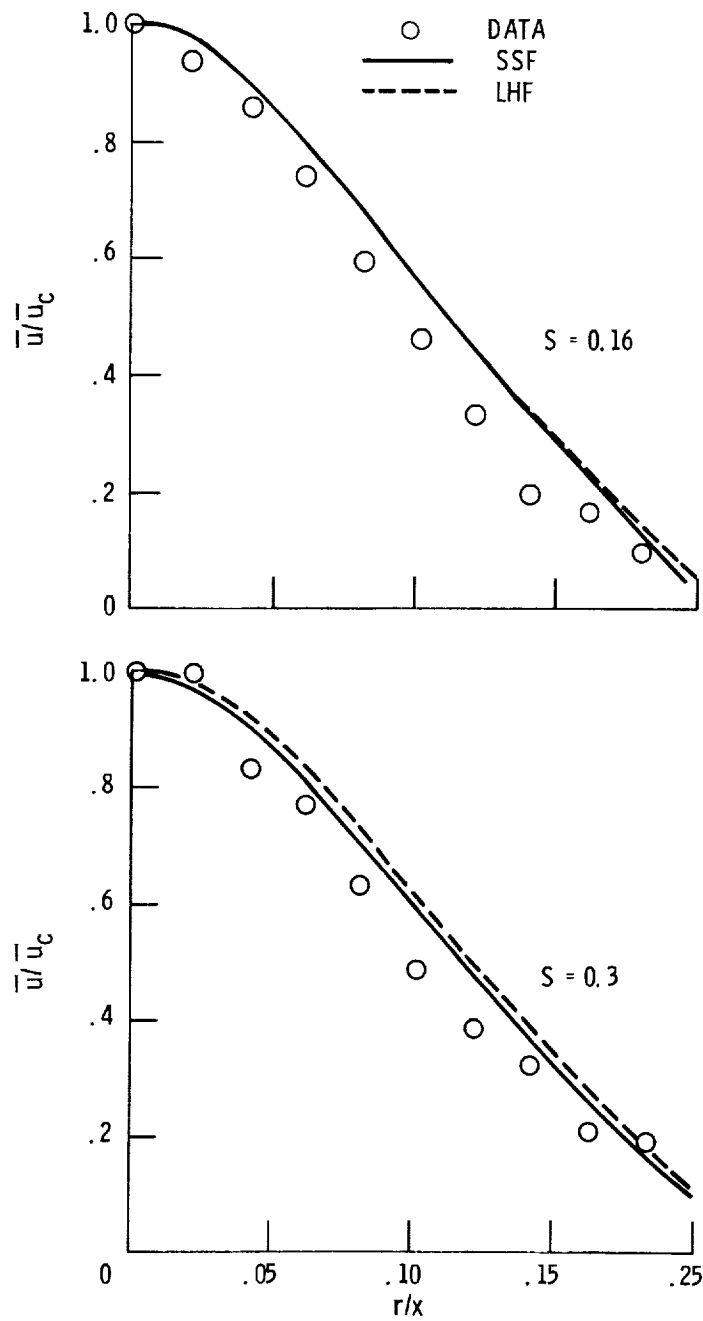
Figure 12. - Radial profiles of gas properties in swirling particle-laden jets at x/d = 20 .
