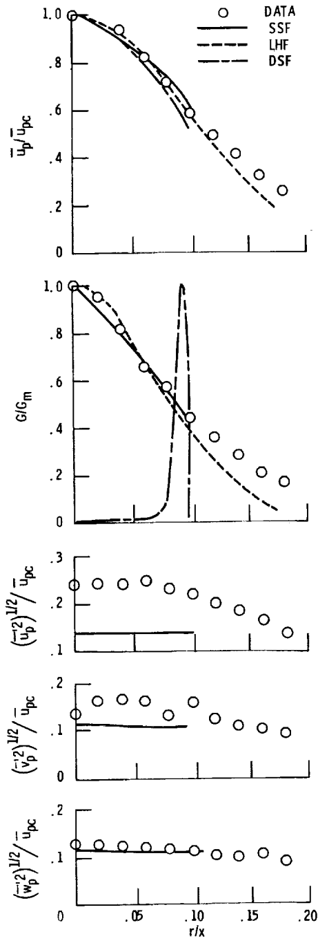
Figure 13. - Radial profiles of particle properties in swirling particle-laden jets at x/d = 20 .
