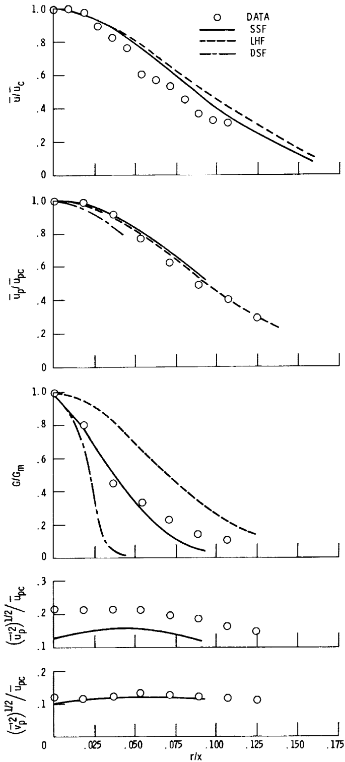
Figure 9. - Radial variation of flow properties in the nonswirling particle-laden jet at x/d = 30 .
