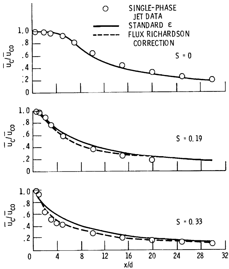
(a) Streamwise velocities.
