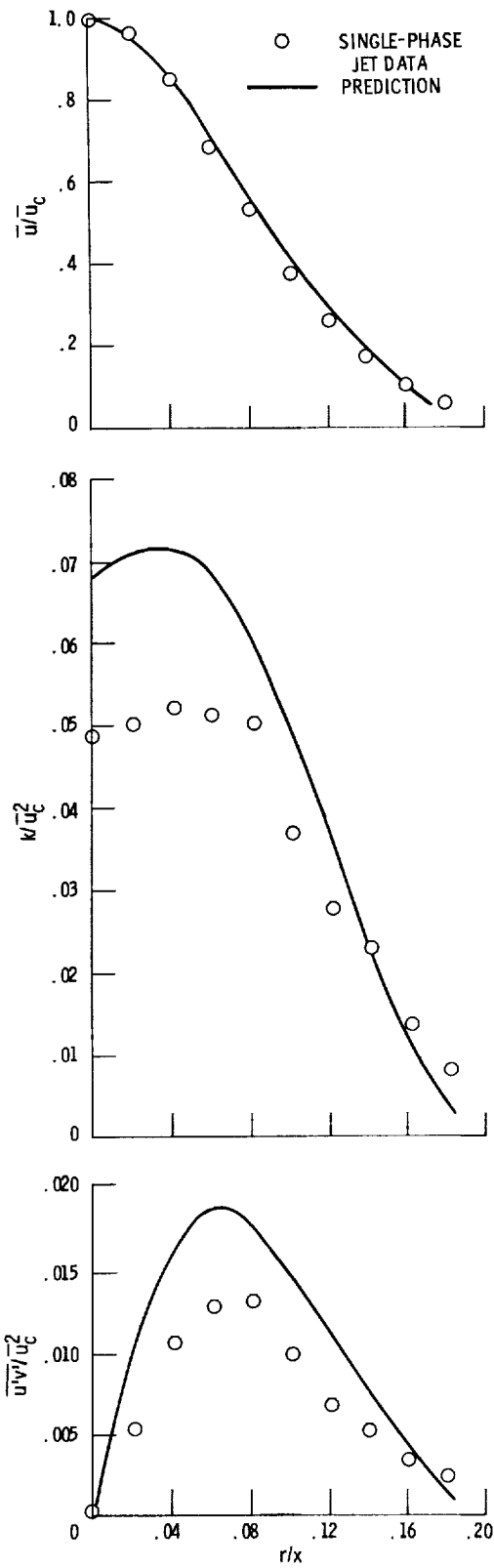
Figure 2. - Radial profiles of flow properties in the single-phase nonswirling jet at x/d = 15 .
