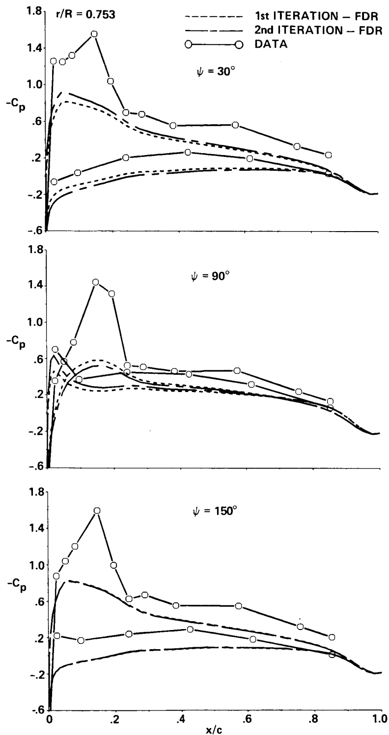
(a) r/R = 0.753 : azimuth = 30, 90, 150 degrees.
