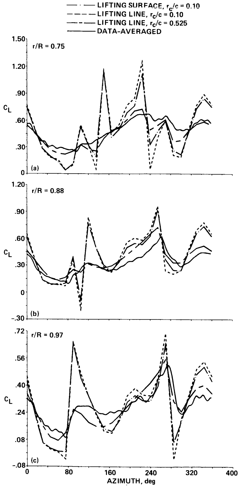
Fig. 12. Effect of lifting surface correction on lift - Condition 1. (a) r/R = 0.75 . (b) r/R = 0.88 . (c) r/R = 0.97 .
