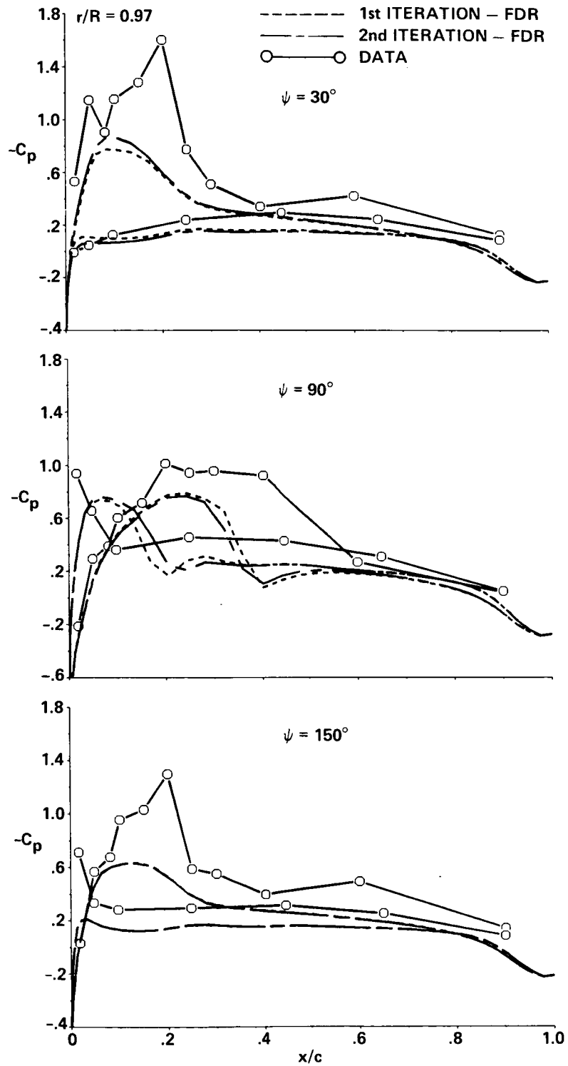
(c) r/R = 0.97 : azimuth = 30, 90, 150 degrees.
