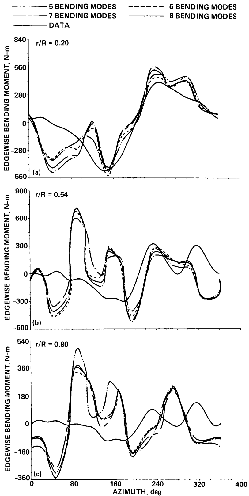
Fig. 19. Effect of number of bending modes on edgewise bending moment - Condition 2. (a) r/R = 0.20 . (b) r/R = 0.54 . (c) r/R = 0.80 .
