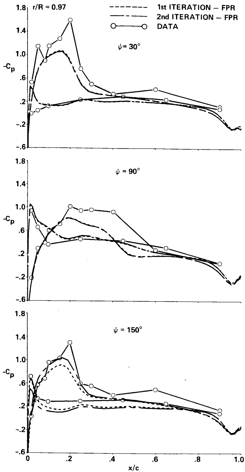
(c) r/R = 0.97 : azimuth - 30, 90, 150 degrees.
