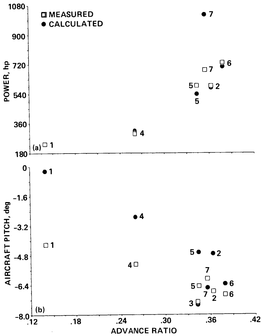
Fig. 9. Trimmed aircraft characteristics (numbers correspond to flight condition). (a) Performance. (b) Aircraft attitude.
