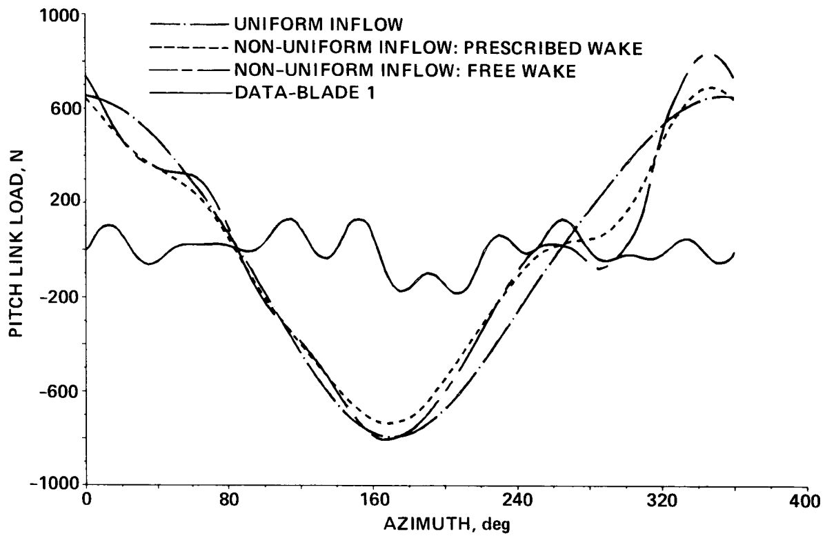
Fig. 16. Effect of wake geometry on pitch-link loads - Condition 1.
