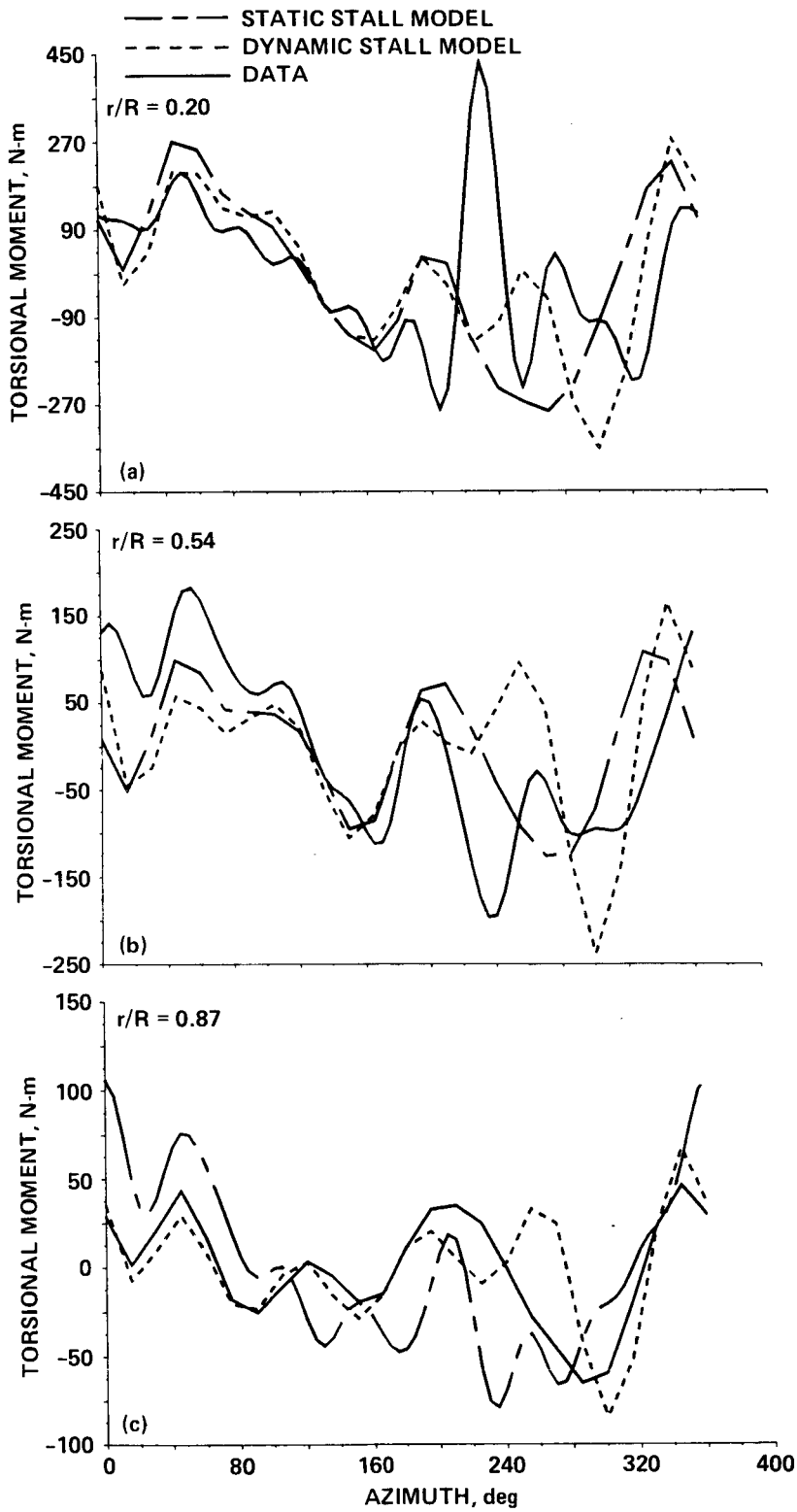
Fig. 29. Effect of stall model on torsional moment - Condition 3. (a) r/R = 0.20 . (b) r/R = 0.54 . (c) r/R = 0.87 .
