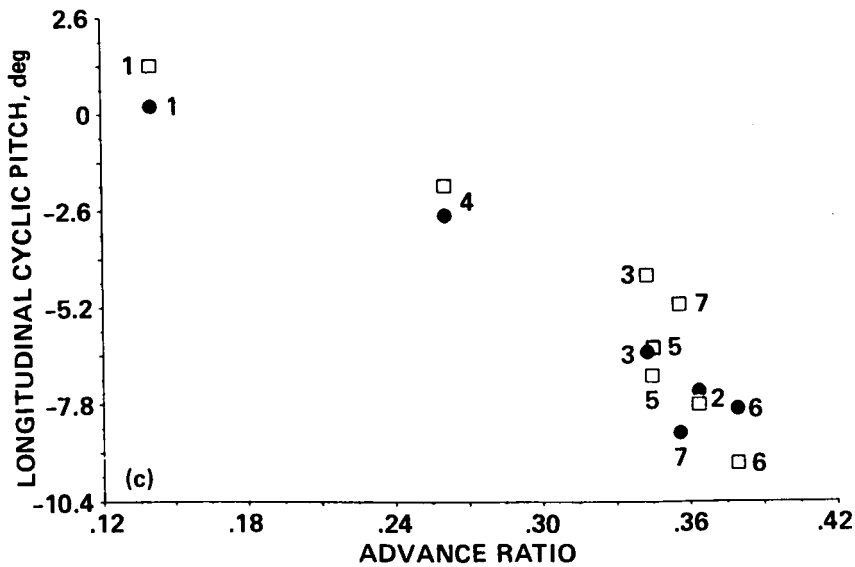
Fig. 8. Trimmed control inputs (numbers correspond to flight condition). (a) Collective. (b) Lateral cyclic. (c) Longitudinal cyclic.
