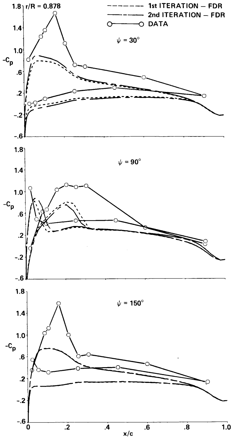
(b) r/R = 0.878 : azimuth = 30, 90, 150 degrees.
