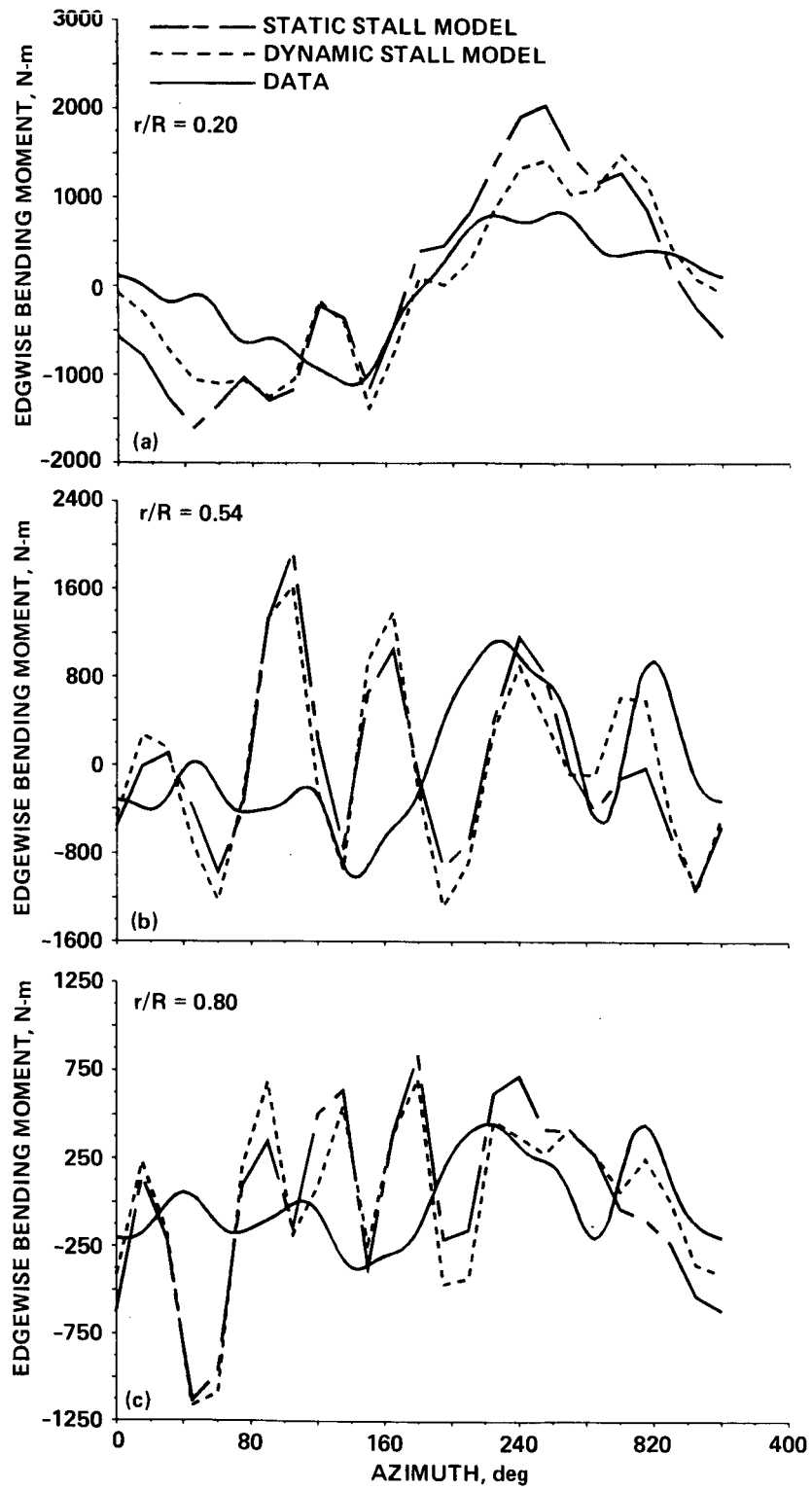
Fig. 28. Effect of stall model on edgewise bending moment - Condition 3. (a) r/R = 0.20 . (b) r/R = 0.54 . (c) r/R = 0.80 .
