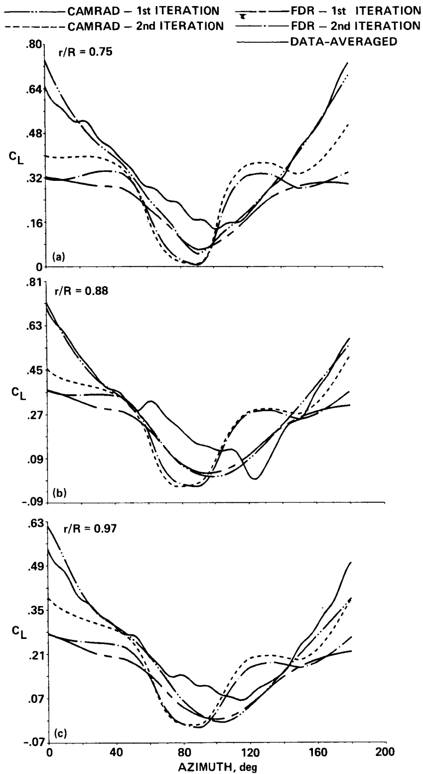
Fig. 23. Lift predictions using CAMRAD and CAMRAD/FDR - Condition 2. (a) r/R = 0.75 . (b) r/R = 0.88 . (c) r/R = 0.97 .
