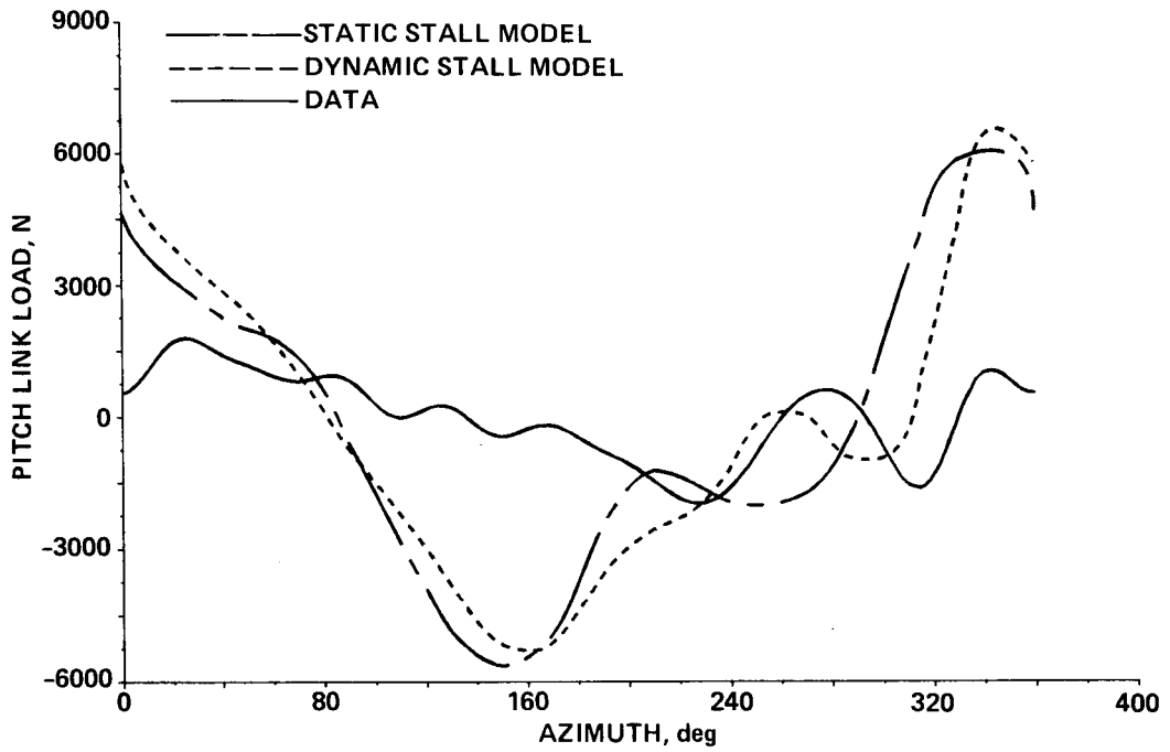
Fig. 30. Effect of stall model on pitch link loads - Condition 3.
