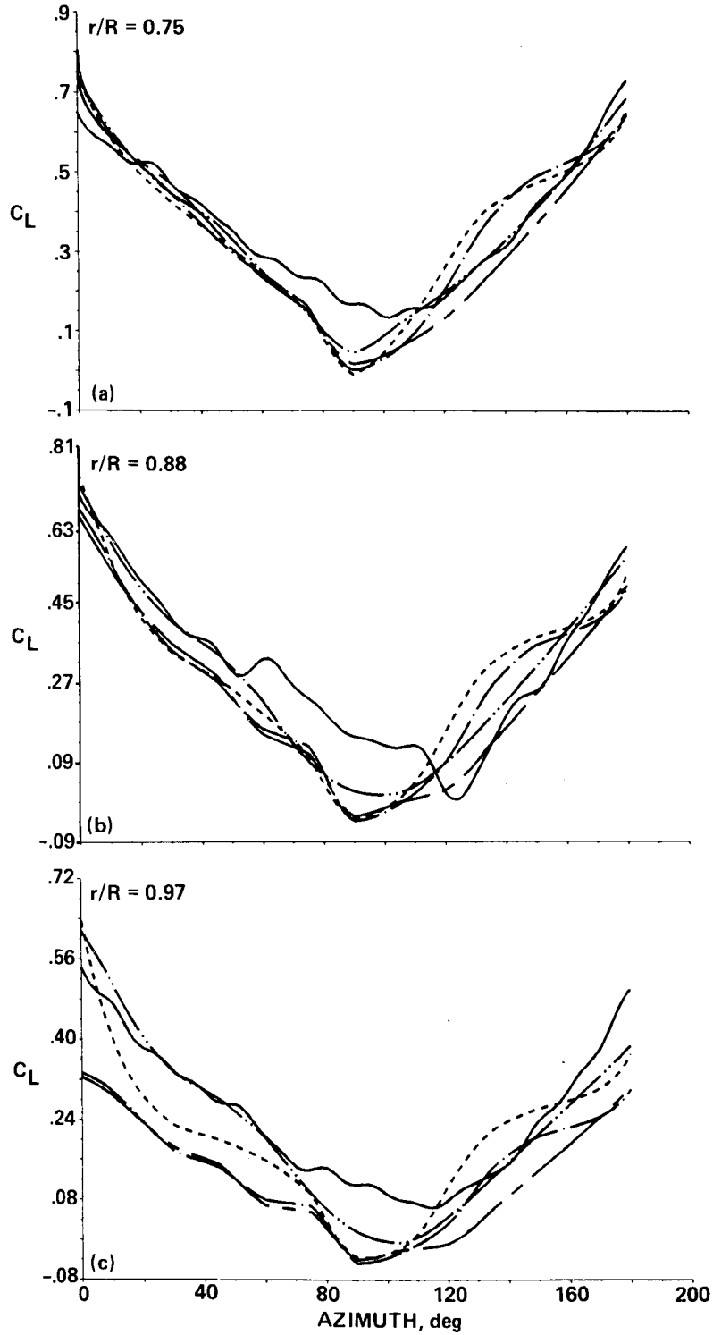
Fig. 22. Lift predictions using CAMRAD and CAMRAD/FPR - Condition 2. (a) r/R = 0.75 . (b) r/R = 0.88 . (c) r/R = 0.97 .
