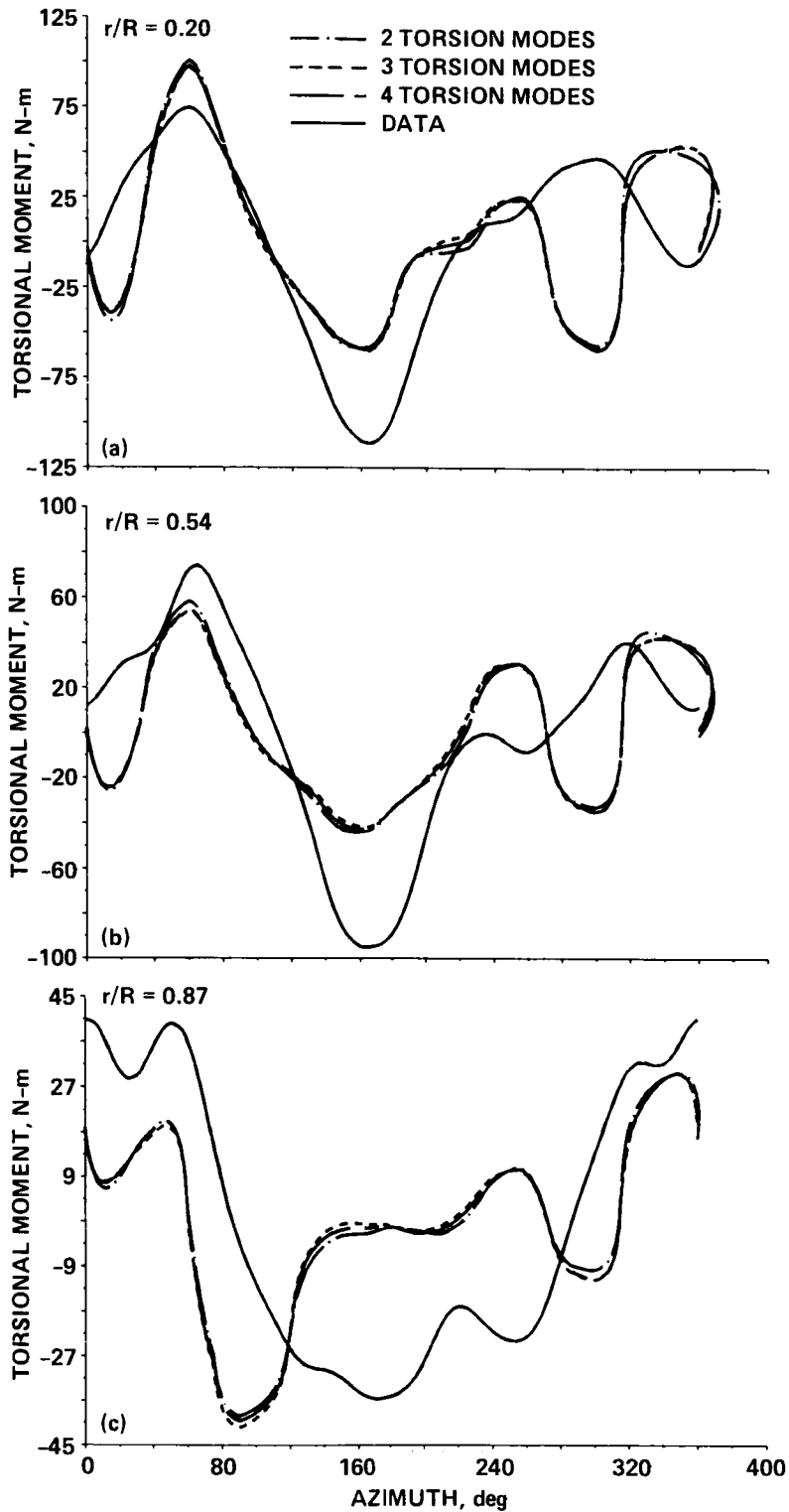
Fig. 21. Effect of number of torsion modes on torsional moment - Condition 2. (a) r/R = 0.20 . (b) r/R = 0.54 . (c) r/R = 0.87 .
