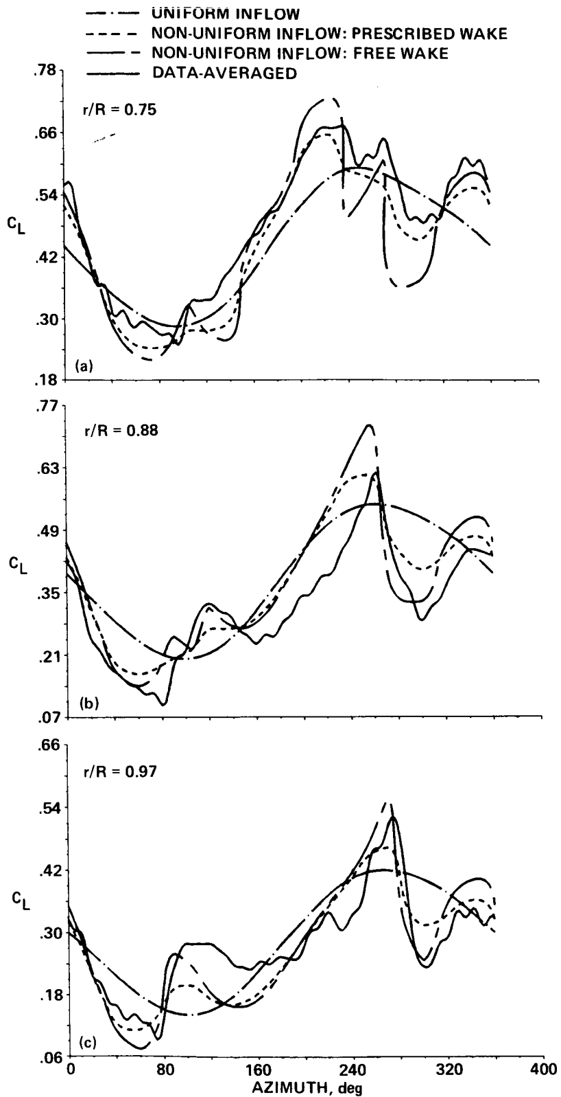
Fig. 10. Effect of wake geometry on lift - Condition 1. (a) r/R = 0.75 . (b) r/R = 0.88 . (c) r/R = 0.97 .
