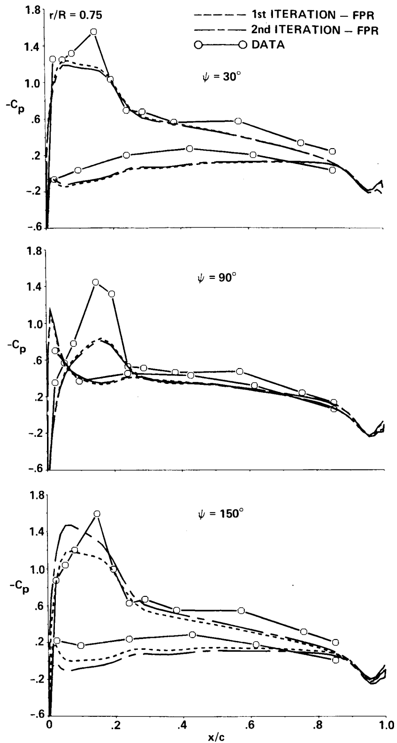
(a) r/R = 0.75 : azimuth = 30, 90, 150 degrees.
