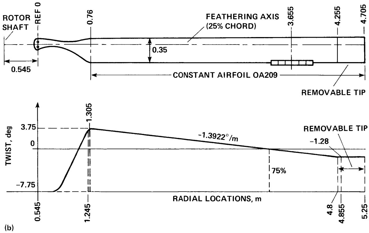
Fig. 3. Grande Vitesse (GV) blade characteristics. (a) OA209 airfoil profile. (b) Blade twist distribution.
