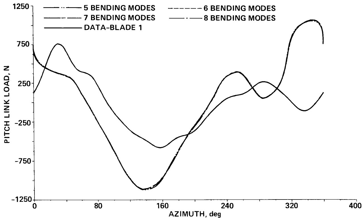
Fig. 20. Effect of number of bending modes on pitch-link loads - Condition 2.
