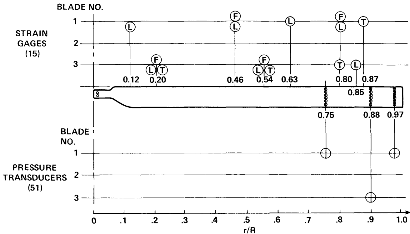
Fig. 4. Blade pressure transducer and strain gage locations.
