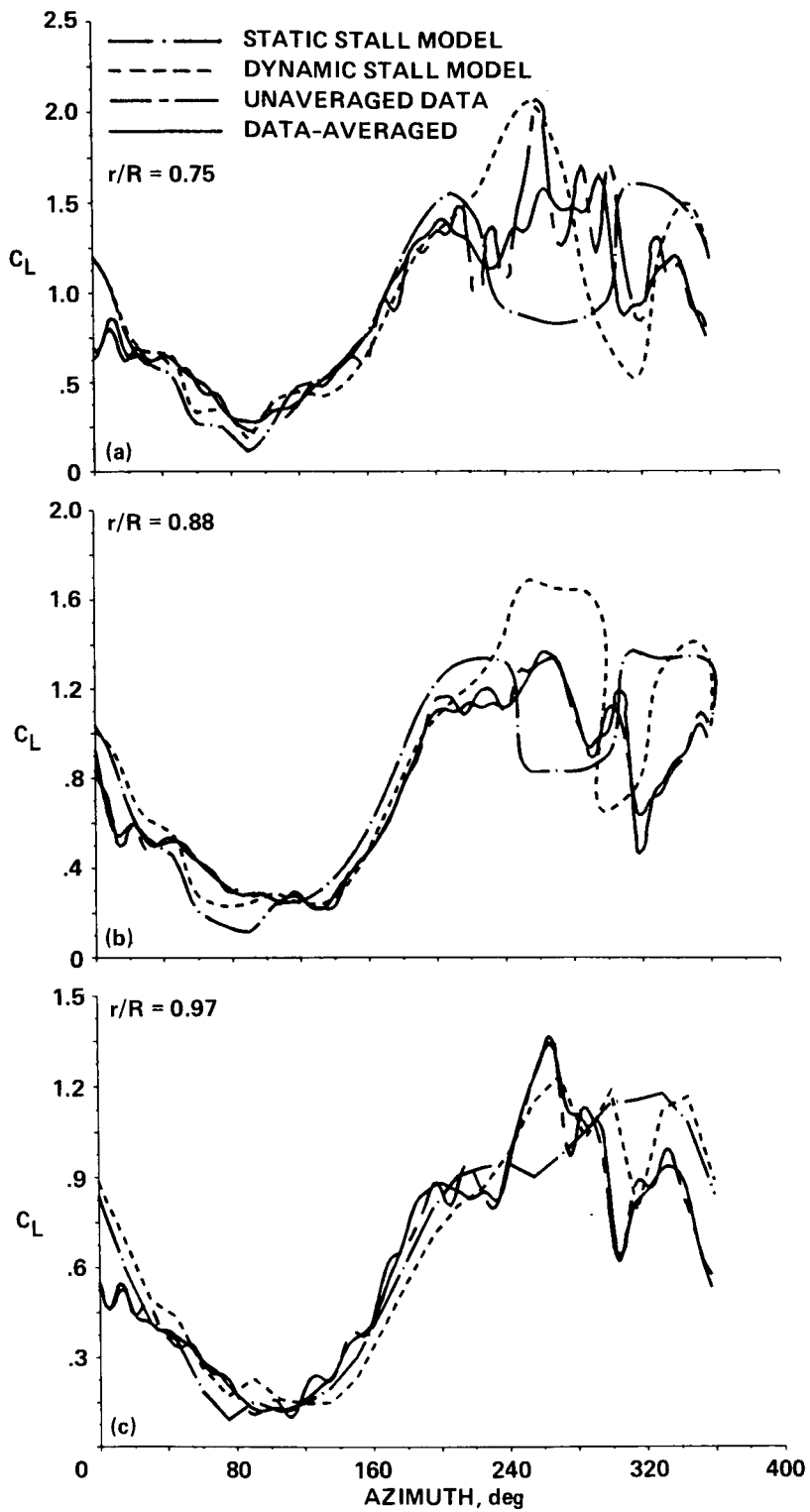
Fig. 26. Effect of stall model on lift - Condition 3. (a) r/R = 0.75 . (b) r/R = 0.88 . (c) r/R = 0.97 .
