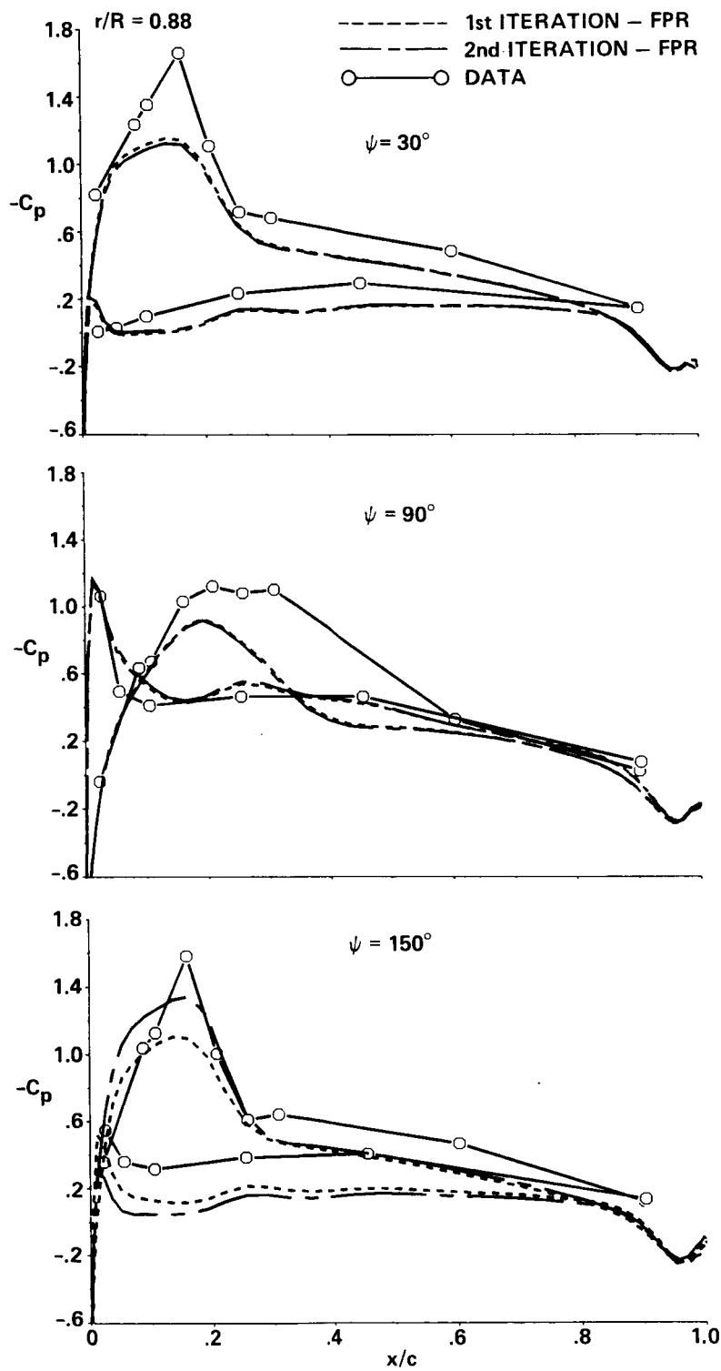
(b) r/R = 0.88 : azimuth = 30, 90, 150 degrees.
