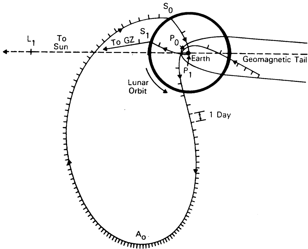
FIGURE 7 HYPERBOLIC DOUBLE LUNAR SWINGBY TRAJECTORY TO COMET GIACOBINI-ZINNER
