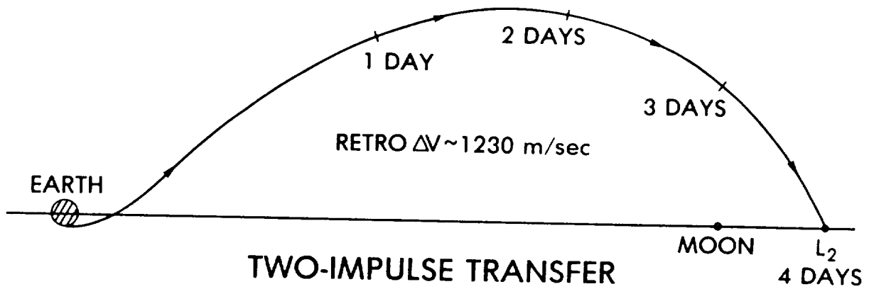
FIGURE 5 TRAJECTORIES TO VICINITY OF EARTH-MOON L_2 POINT
