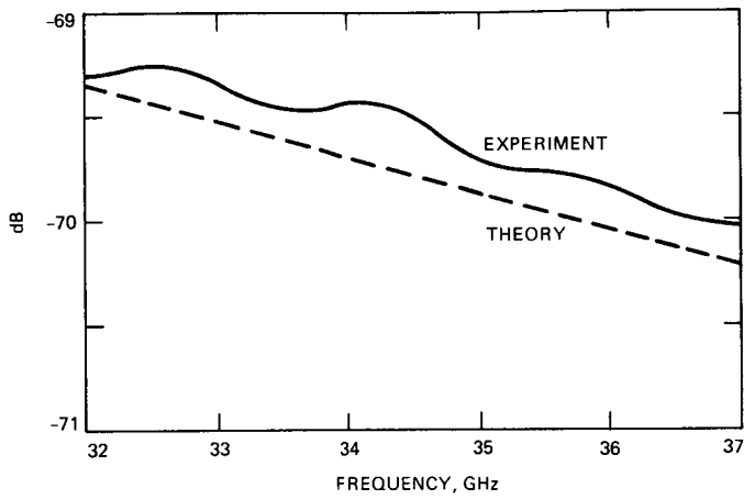
Fig. 4. The TE_{11} coupling measurement vs theoretical results
