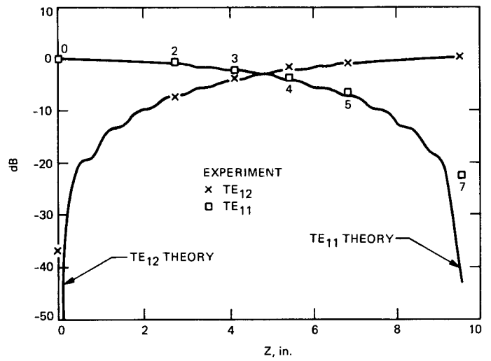
Fig. 6. Mode converter mode content vs distance
