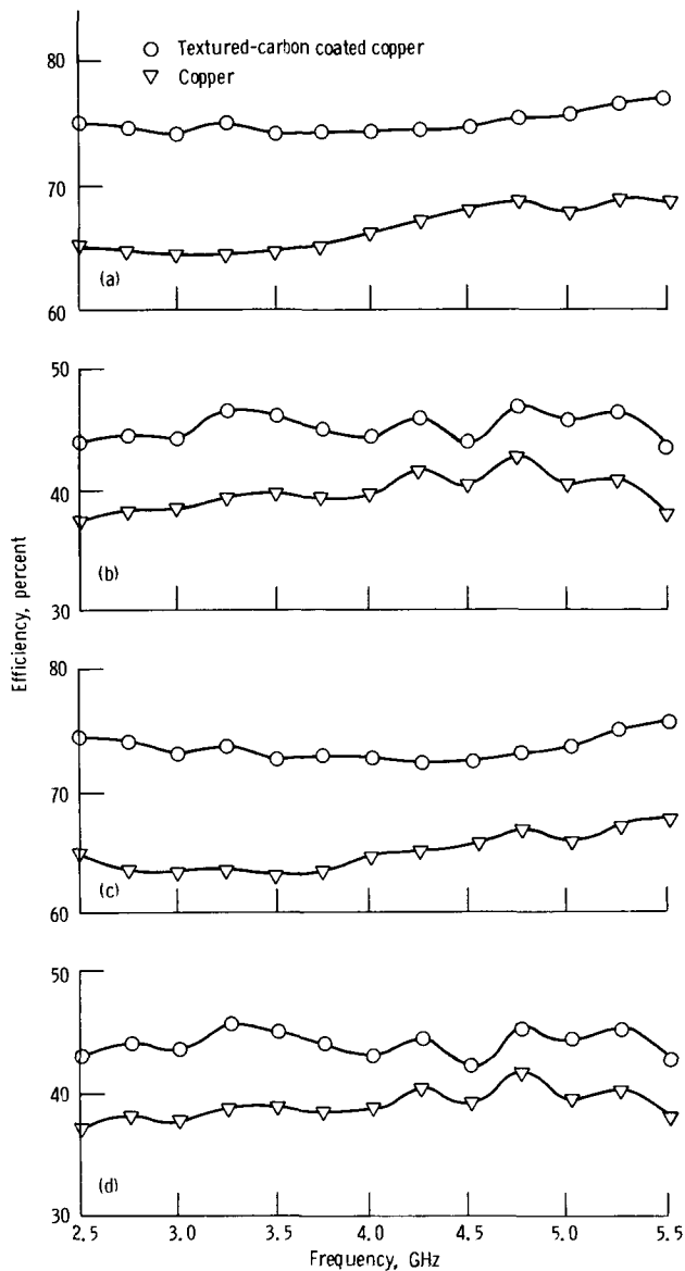
(a) Four-stage MDC; collector efficiency. (b) Four-stage MDC; overall efficiency. (c) Three-stage MDC; collector efficiency. (d) Three-stage MDC; overall efficiency.
