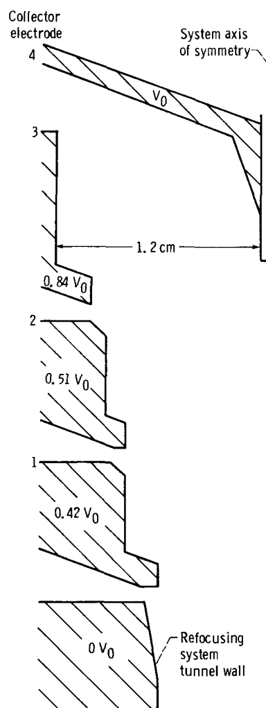
Figure 2.—Active electrode geometry and typical applied potentials for MDC 1.
