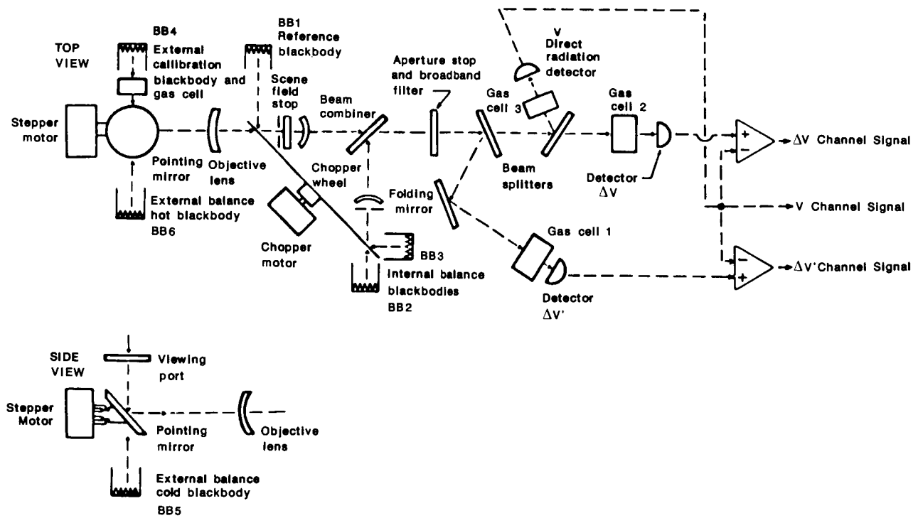
Figure 10.- MAPS instrument layout.
