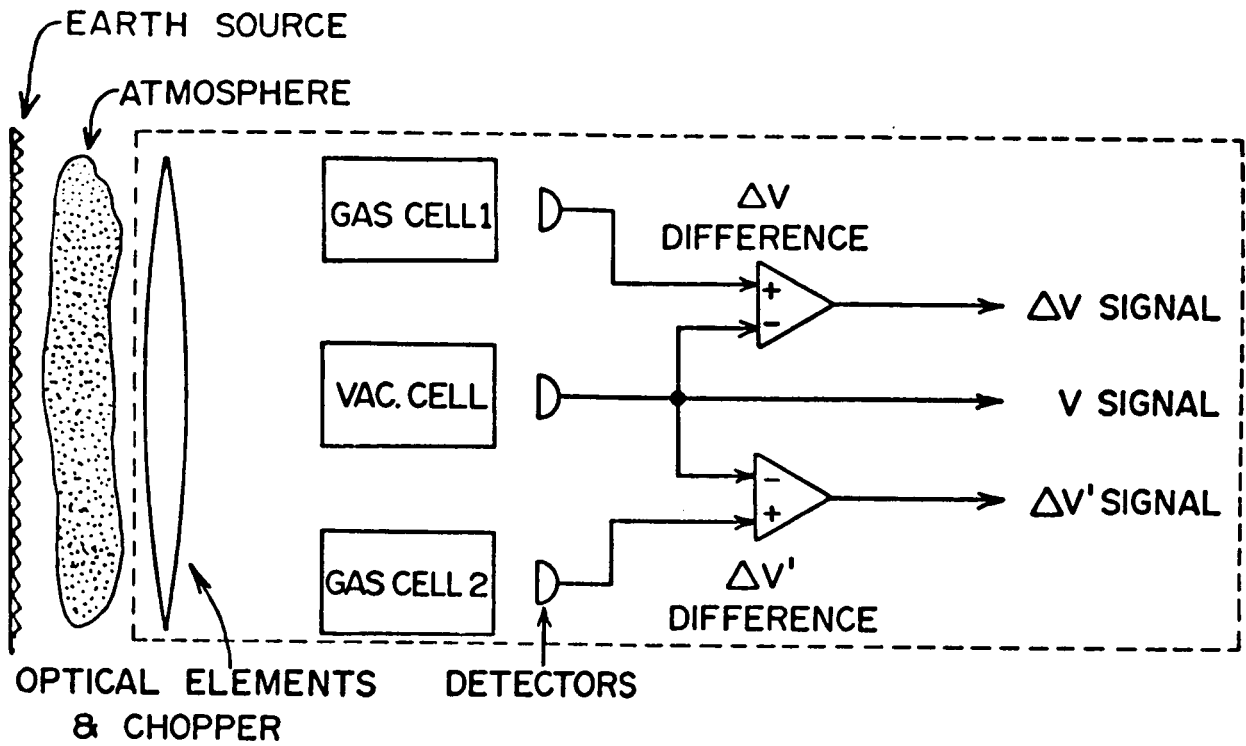
Figure 9.- GFR schematic.
