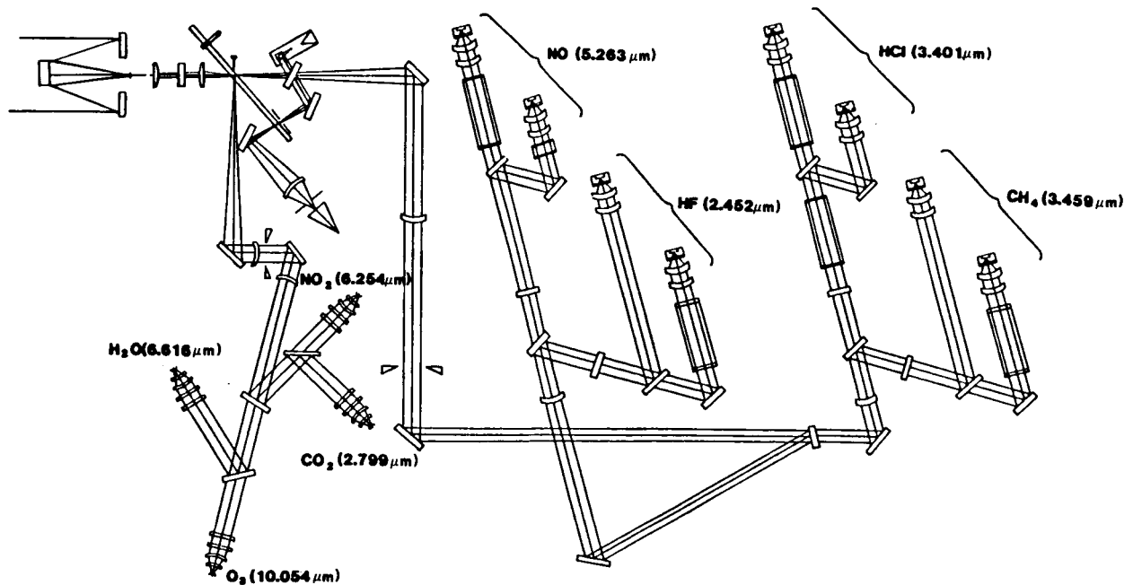
Figure 14.- HALOE schematic.
