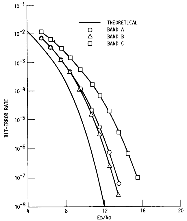
(B) BIT-ERROR RATE PERFORMANCE.
