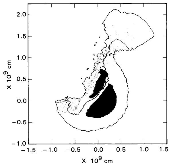
Figure 20. Results of two-dimensional computer simulations of the impact of a Mars-sized object with primitive Earth. Black areas are metallic iron, and stippled areas are silicates; stipple density is proportional to material density, which is initially that of molten silicate. Impact velocity is 12 km/s; calculation includes the effects of gravity. (a) About 250 seconds after impact; small jets are beginning to develop. (b) About 1500 seconds after impact; jet has expanded considerably and the most heated material (almost entirely vapor) will be lost, but the "neck" of the plume is likely to be trapped in Earth's orbit. (Courtesy of M. Kipp and H. J. Melosh).
