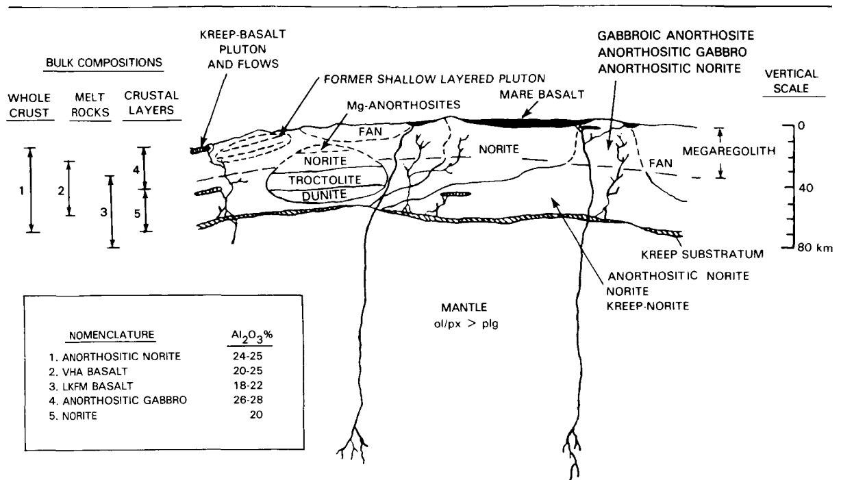
Figure 14. Schematic cross-section of the lunar crust showing possible geologic relations among lunar rock types. The provenance of bulk compositions is shown at the left. This reconstruction is one of several possible interpretations of a wide variety of lunar sample, remote-sensing, cratering, and geophysical data. FAN, ferroan anorthosite; VHA, very high alumina basalt; LKFM, low K Fra Mauro basalt; ol/px > plg, olivine and pyroxene greater than plagioclase.
