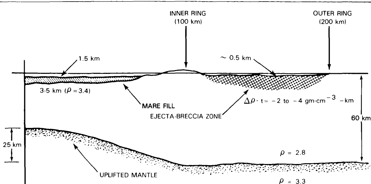
Figure 12. Schematic cross-section of lunar Grimaldi Basin determined from gravity data. The uplift of the mantle material near the basin center is at least partly responsible for the observed positive gravity anomaly (mascon) in the basin. From Phillips and Dvorak (1981).
