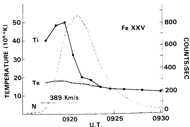
Figure 4.9 HXRBS and BCS results for the April 10, 1980 flare. T_i is a measure of the nonthermal broadening. See Antonucci et al. (1982) for details.
