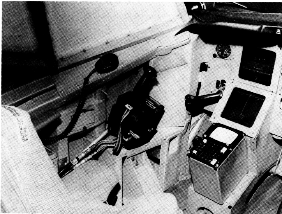
Figure 2. Two-axis sidestick controller.
