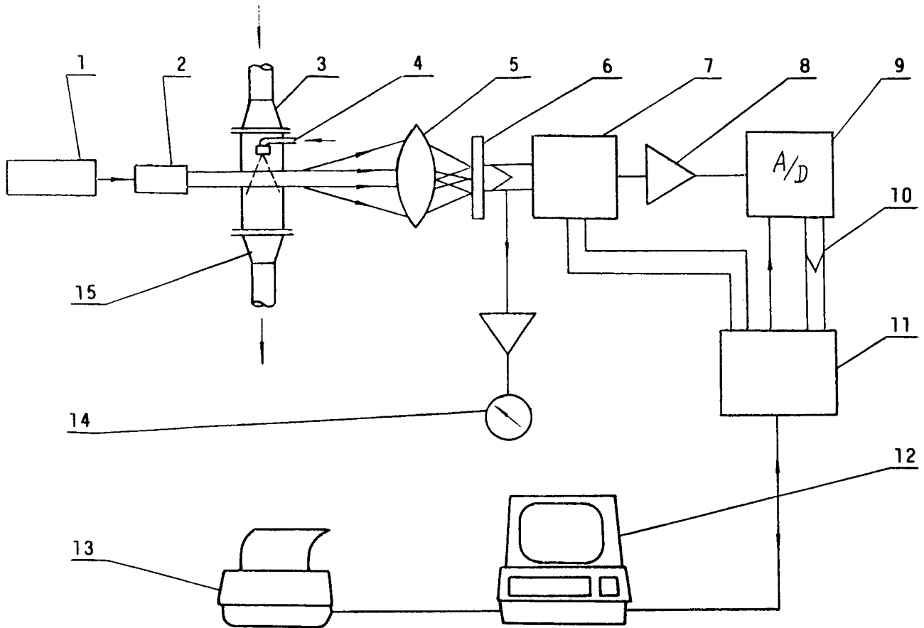
Figure 4. - Laser drop particle sizer. Laser, 1; beam expander, 2; test section, 3; fuel nozzle, 4; lens, 5; photo detector, 6; solid valve, 7; amplifier, 8; A/D converter, 9; data transfer, 10; interface, 11; computer, 12; printer, 13; micro tune, 14.
