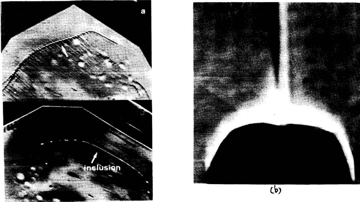
fig.3 Inclusion trap due to the development of a convection plume, when the supersaturation is above 0.5%, (a) surface micrograph and (b) Schlieren image
