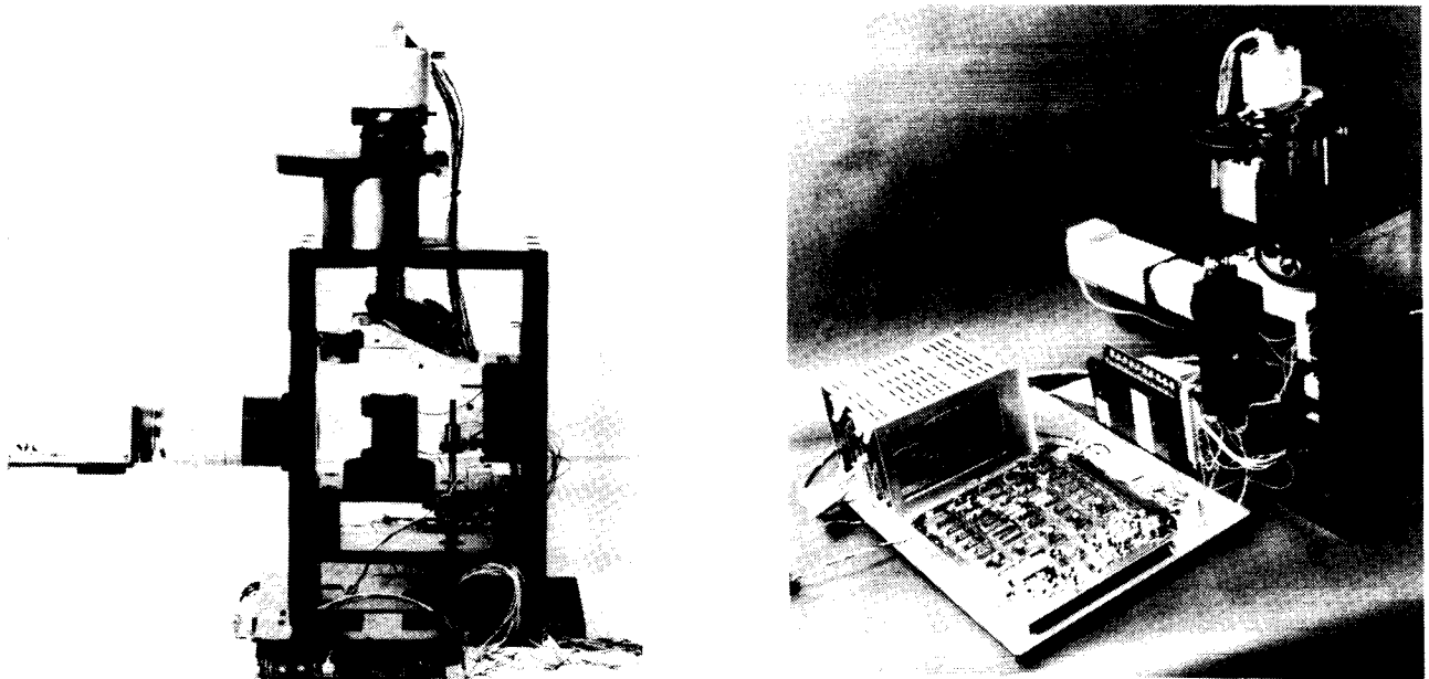
fig.5 Proto-type microscope in microgravity, by which one can observe growth steps with mono-molecular height and automatically measure the growth rate of a crystal
