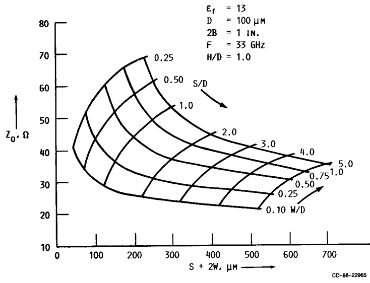
FIGURE 16.- INVERTED CPW.
