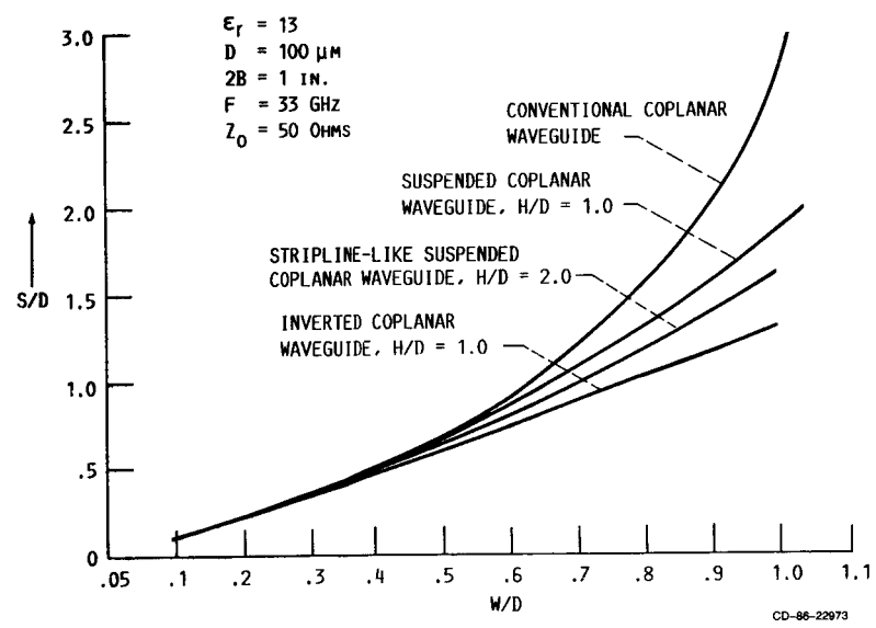
FIGURE 17.- 50 OHMS CPW TRANSMISSION LINES.
