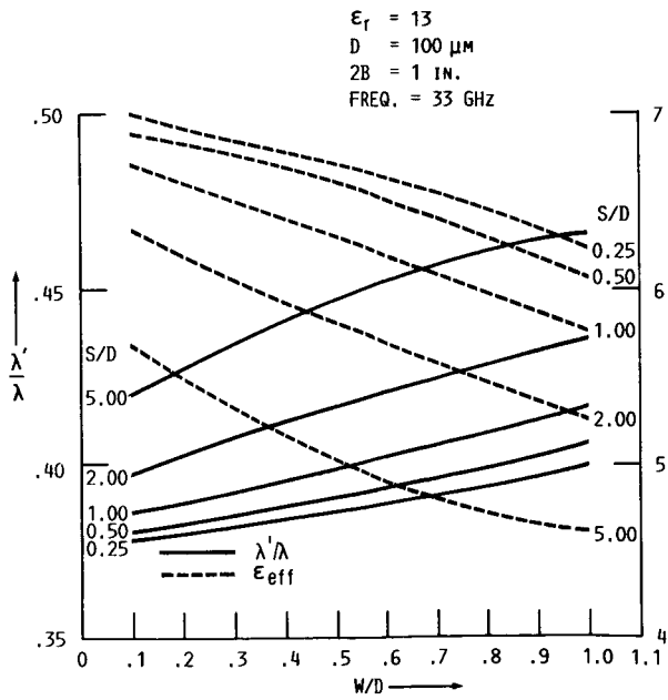
FIGURE 4.- CONVENTIONAL CPW.
