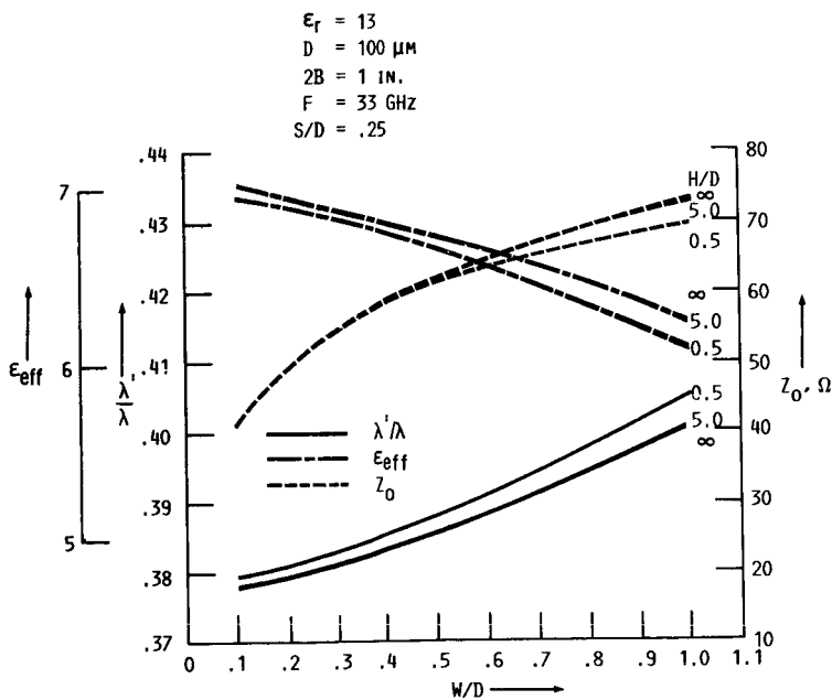
FIGURE 8.- SUSPENDED CPW.
