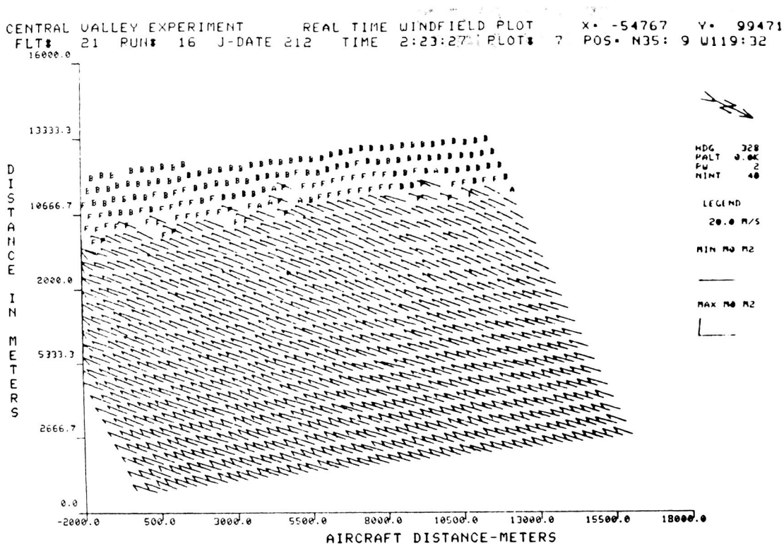
Figure 13. VECTOR VELOCITY MAP OF A UNIFORM FLOW FIELD IN A HORIZONTAL PLANE AT THE ALTITUDE OF THE AIRCRAFT.
