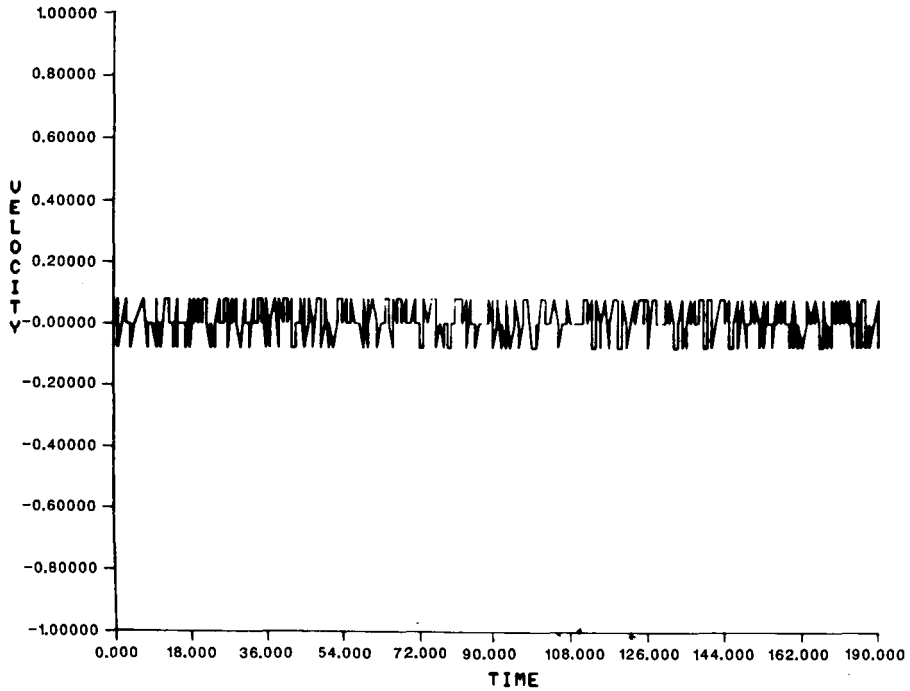
Figure 7. APPARENT DOPPLER VELOCITY OF A MOUNTAIN AT A RANGE OF 4 KM.
