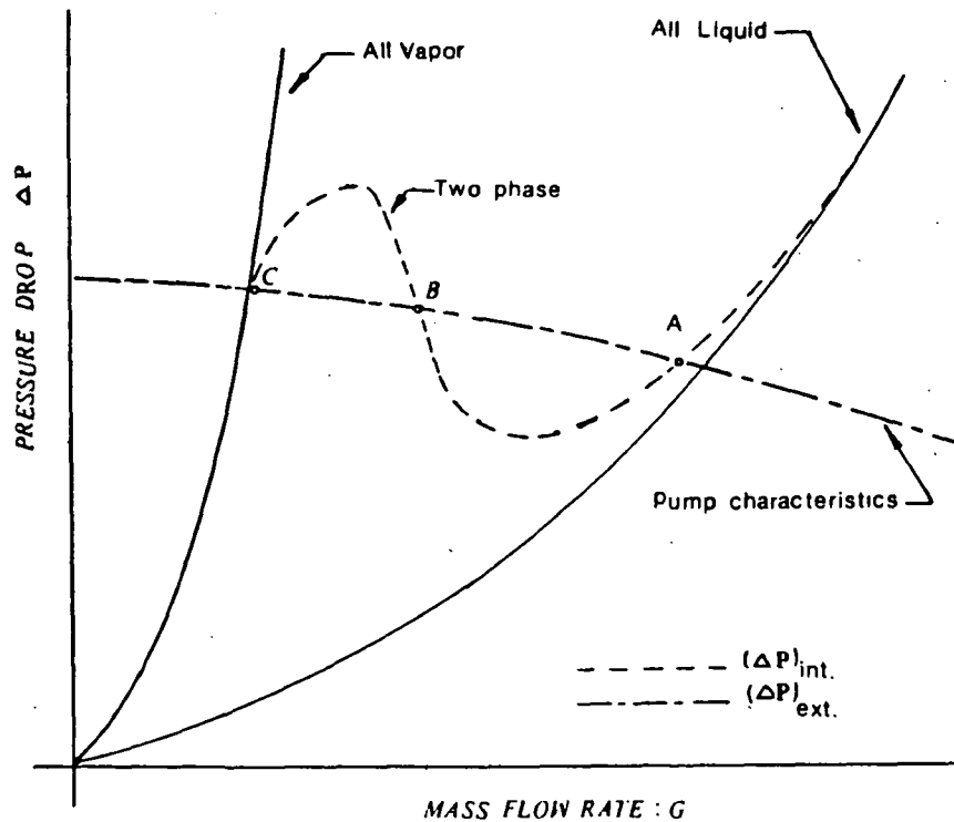
Figure 6 - Two-Phase Flow Pressure Drop Characteristics
