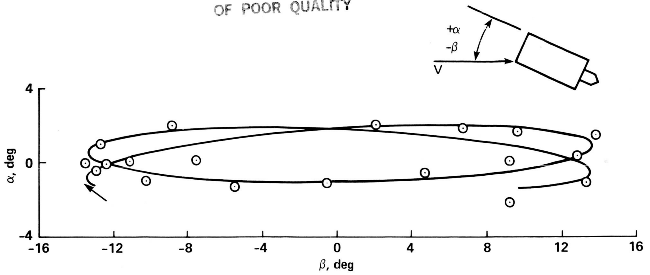
(a) Angular motions, test 1818.
