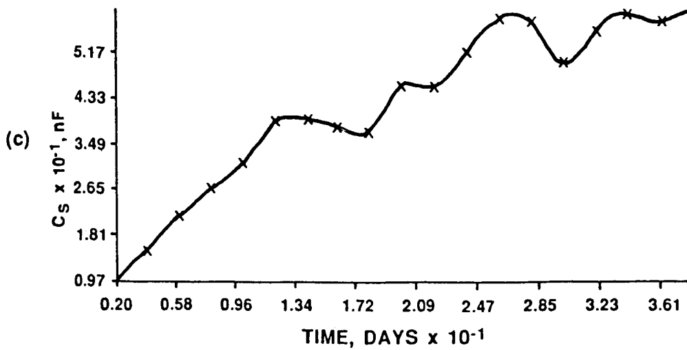
Figure 16. R_p , C_f , and C_s versus time at pH 8.2.
