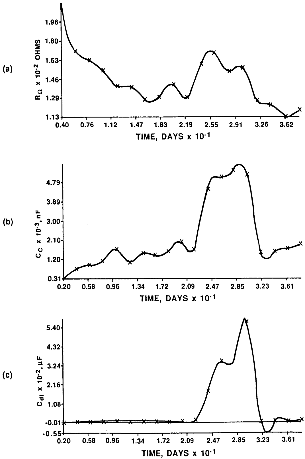
Figure 11. R_{\Omega} , C_C , and C_{dl} versus time at pH 5.5.
