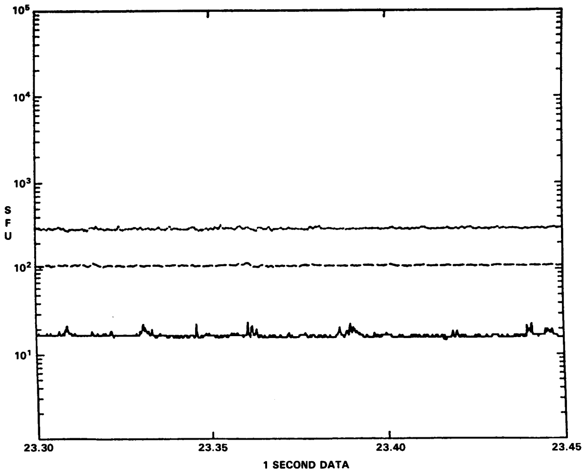
Figure 2. Preflare interval (interval A) for 245, 1415 and 8800 MHz. Data are at 1-second resolution from 2330 UT to 2345 UT on 24 April.
