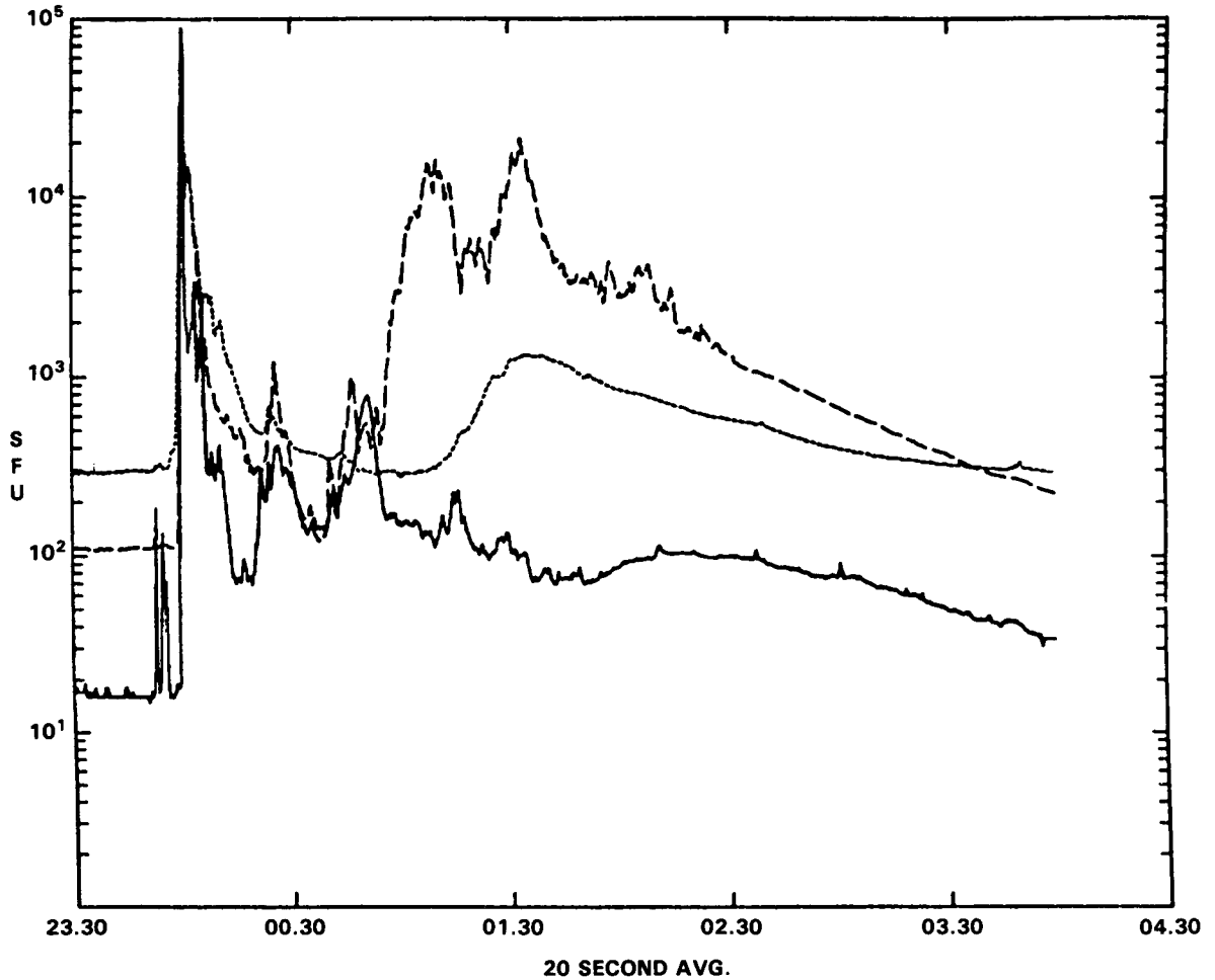
Figure 1. Plots of the 24-25 April 1984 radio burst using 20-second averages at 245, 1415 and 8800 MHz. Data from Learmonth, Australia.
