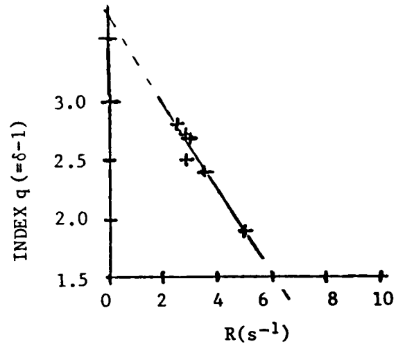
Figure 7 - Scatter diagram between pulse repetition rates and X-ray spectral index, for the last six burst structures.
