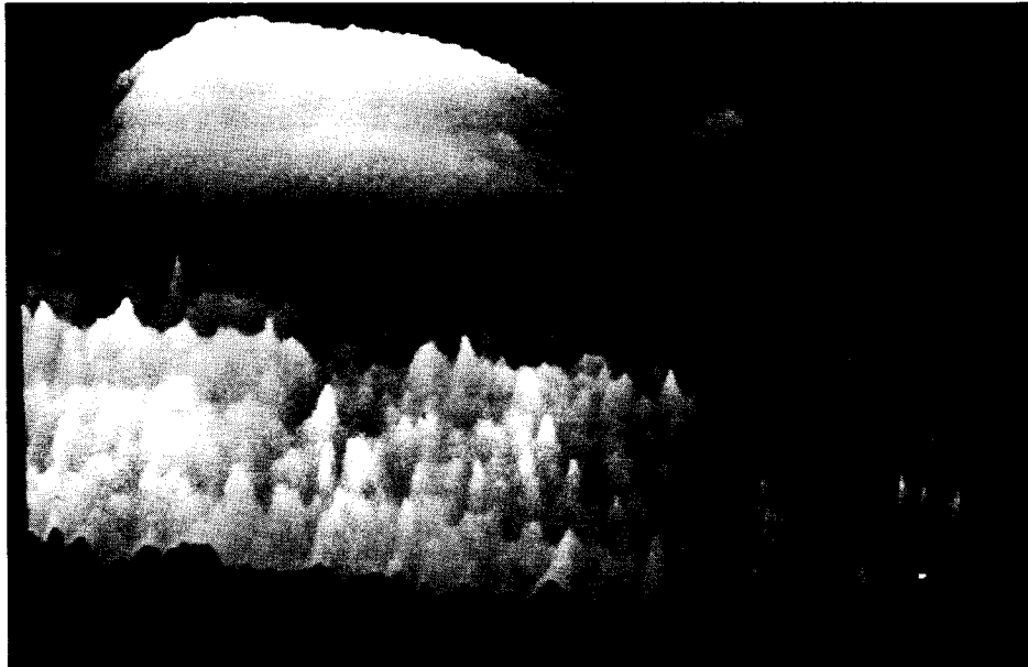
Fig. 2: Three-dimensional representation of spikes (front) and type III bursts (back): time increases to the right (total of 4 seconds is shown). Frequency decreases with depth (370-250 MHz), and flux is shown logarithmically in vertical direction. The data was recorded by the digital spectrometer (IKARUS) in Zurich on 1980, September 24, 0731 UT.
