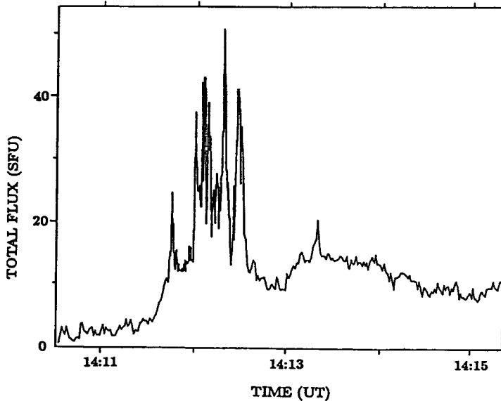
Fig. 5: Observation of spikes at 5.2 GHz by the Institute of Applied Physics in Bern on 1982, February 10. The spikes are superposed on the smoother, impulsive synchrotron emission (courtesy of M. Stähli).
