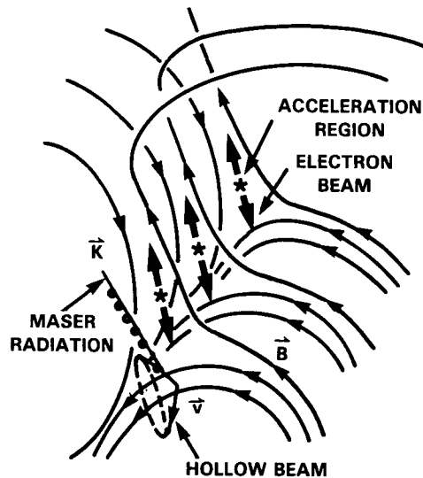
Figure 1. Model of hollow beam driven ECM for SMMSE.
