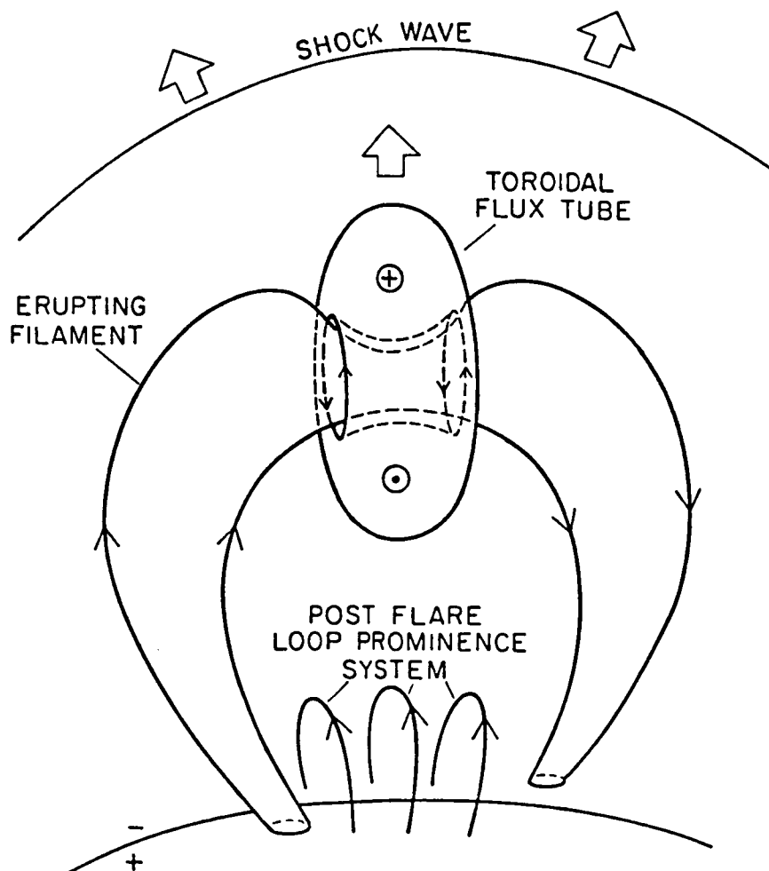
Fig. 20. Schematic representation of situation that arises when a filament, encircled by a toroidal flux tube, is completely ejected from the sun. The toroid would be detectable as a moving type IV radio burst. The shock wave would give rise to a type II radio burst (Sturrock 1986).
