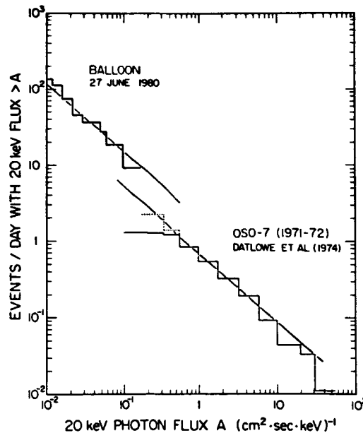
Fig. 5. The distribution of the integral rate of occurrence of events vs. peak 20 keV photon flux for the solar hard X-ray microflares observed in this balloon flight. Also shown for comparison is the distribution of solar flare hard X-ray bursts reported by Datlowe, Elcan, and Hudson (1974) (Lin et al. 1984).
