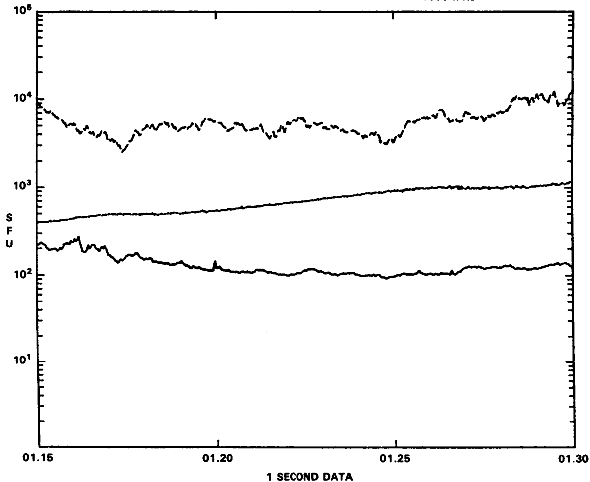
Figure 5. Gradual phase (interval D) for 245, 1415 and 8800 MHz. Data are at 1-second resolution from 0115 UT to 0130 UT on 25 April.
