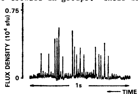
Fig. 3 Weak spike cluster in the noise background occurring at 0910 UT. on July 15, 1981.
