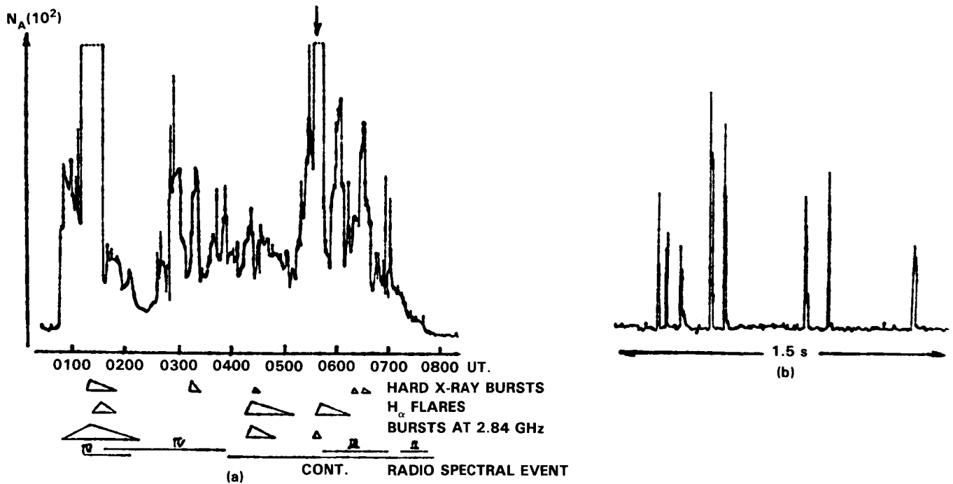
Fig. 8 The event of Feb 2, 1982. a) spike's number per minute ( N_A ) and other solar activities associated. b) the details of flux density at the time indicated by an arrow in Fig. 8a.
