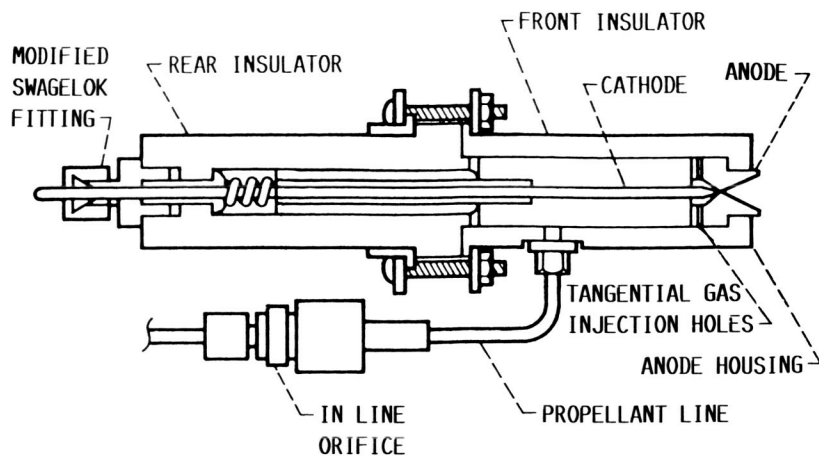
FIGURE 1. - CUTAWAY VIEW OF ARCJET THRUSTER.
