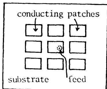
Fig. 1 A 3x5 Subarray of rectangular microstrip patches. Only the center patch is fed.
