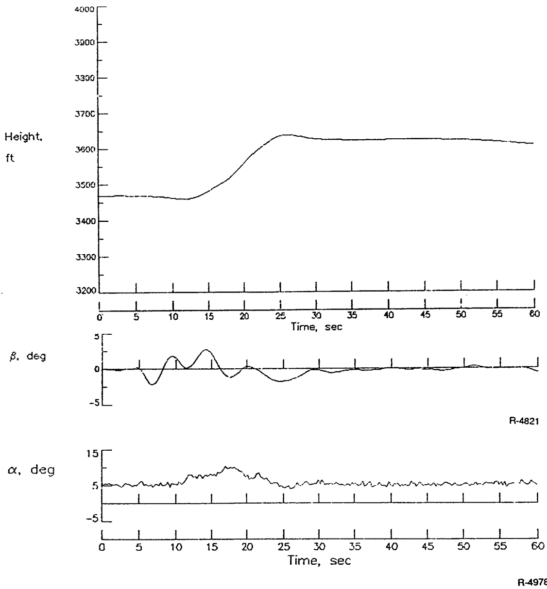
Figure A.6-2. R031, CT1, Limited FCS, Full Reconfiguration
