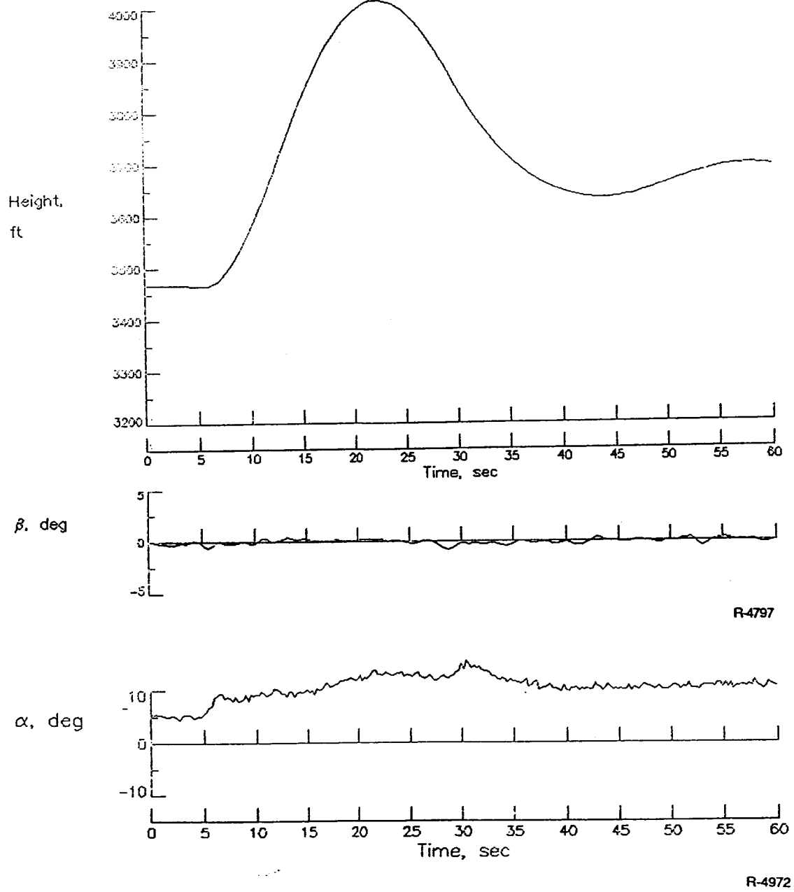
Figure A.3-3. R026, Full FCS, Reconfiguration, Perfect FDI
