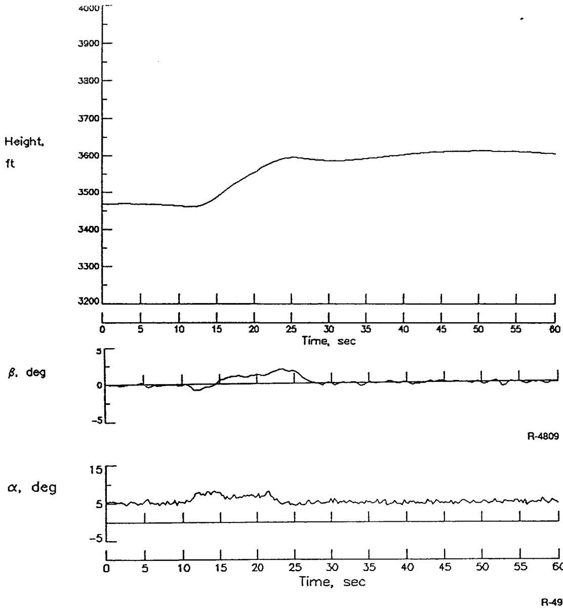
Figure A.5-1. R032, CT1, Limited FCS, No Reconfiguration
