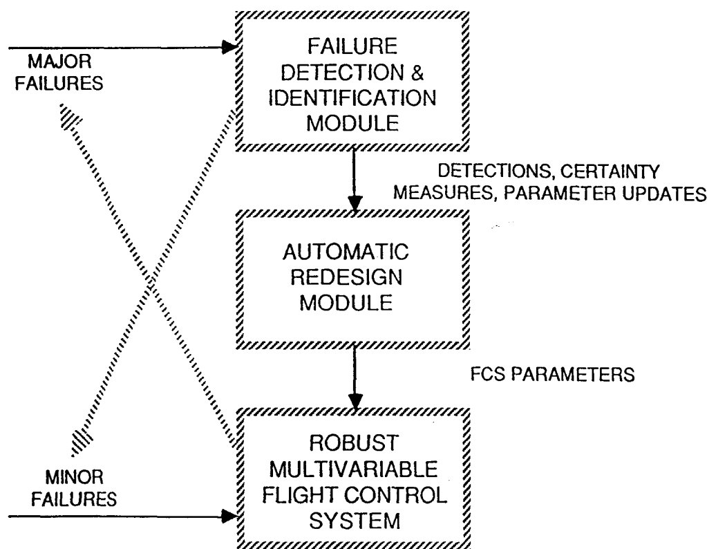
Figure 1-2. RFCS Component Decomposition
