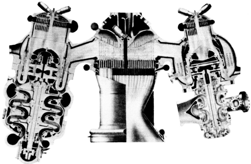
SSME POWERHEAD COMPONENT ARRANGEMENT
