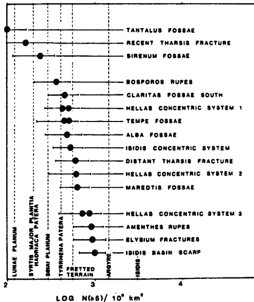
Figure 2. Age plot of dated fracture systems in areal crater density with seven volcanic and impact reference dates.
