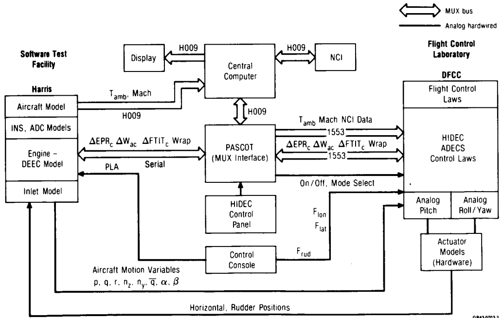
Fig. 10. HIDEC laboratory integration testing, ADECS mode.
