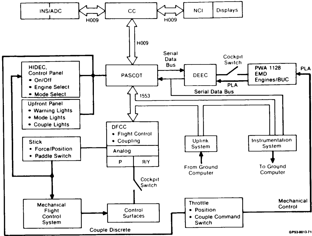
Fig. 7. HIDECS system architecture, ADECS modes.
