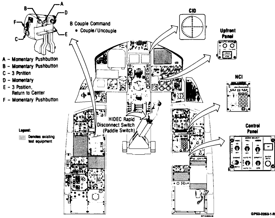
Fig. 9. HIDEC crew station orientation.
