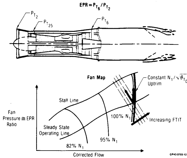
Fig. 5. Adaptive engine control system, subsonic uptrim.
