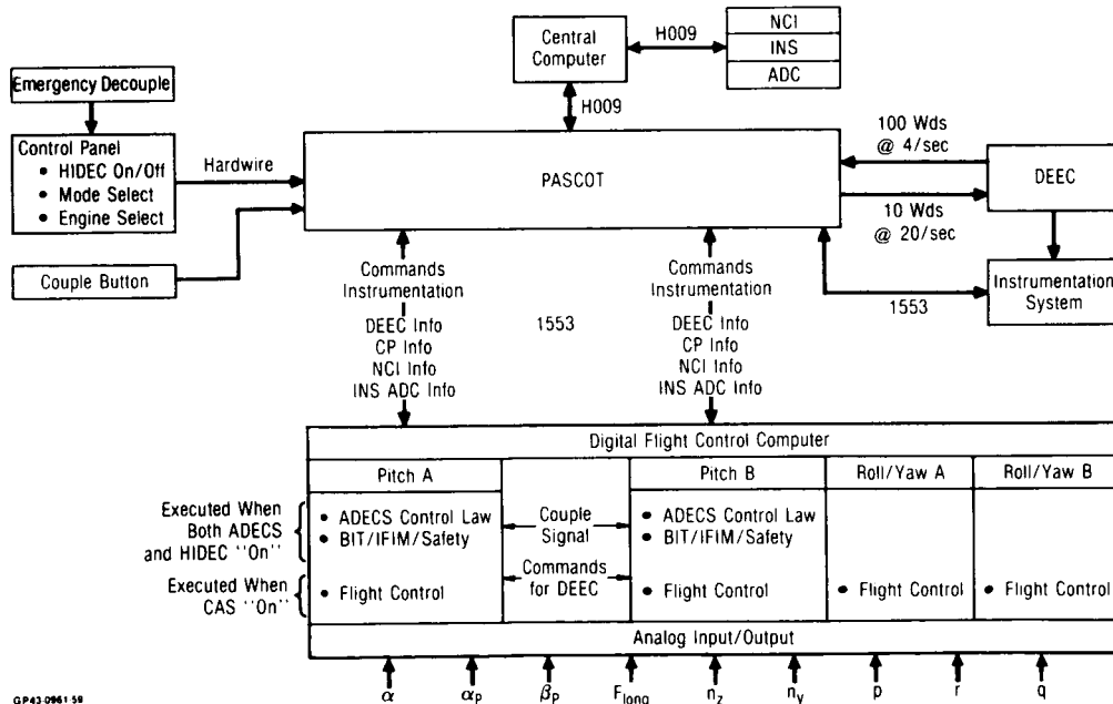
Fig. 8. ADECS architecture.
