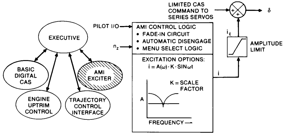
Fig. 3. Aircraft model identification.
