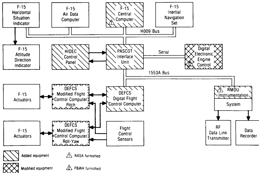
Fig. 2. HIDEC ADECS avionics architecture.
