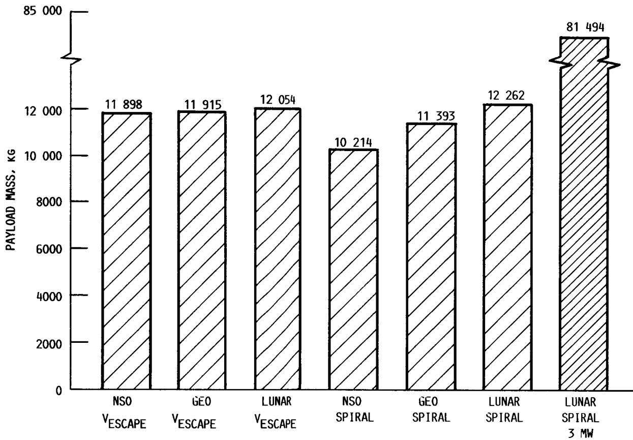
MISSION SCENARIO (B) ARGON, I_{SP} = 9591 SEC. FIGURE 7. - CONCLUDED.
